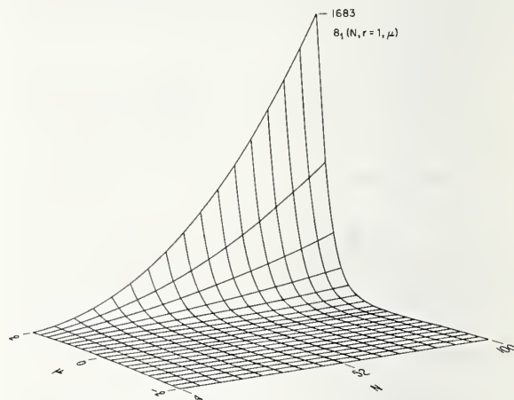
FIGURE 8.2. The bias function, B_1(N, r=1, \mu) .
