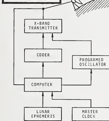
FIGURE 10.53. Simplified diagram of MBTS (Lunar Radio) system.
