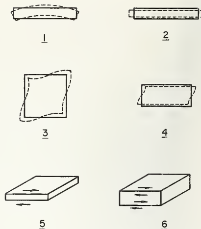
Fig. 2. Basic modes in quartz crystal vibrators. 1 Flexure mode. 2 Extensional mode. 3 and 4 Face shear modes. 5 and 6 Thickness shear modes.
