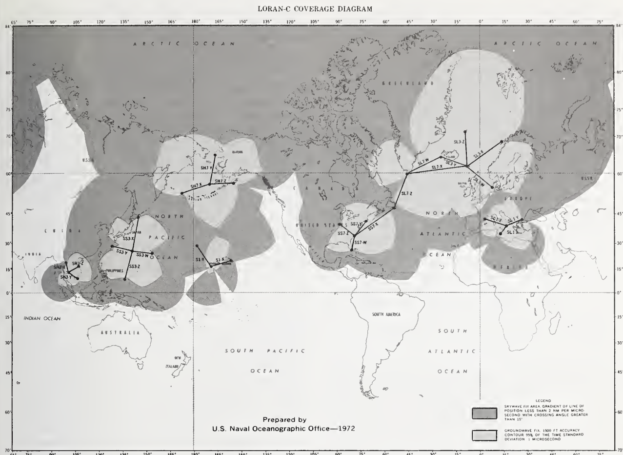
FIGURE 10.18. Coverage of Loran-C navigation system.
