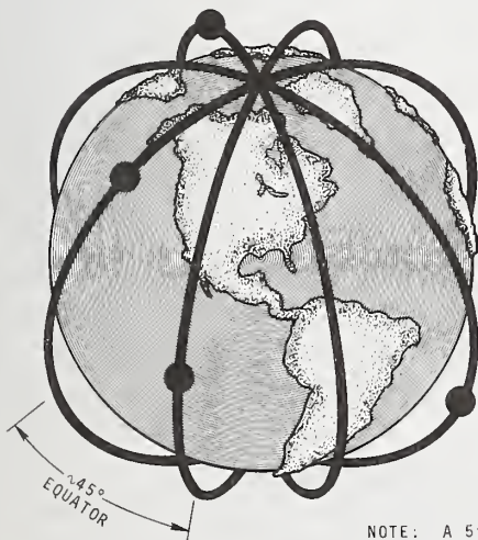
FIGURE 10.38. TRANSIT satellites showing 4 polar orbits. (Consecutive orbits do not repeat around rotating earth.)
