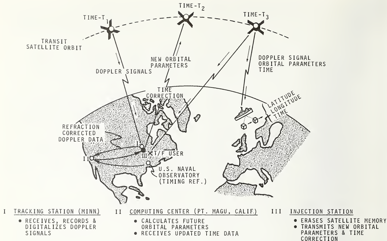
FIGURE 10.39. TRANSIT satellite system operation.
