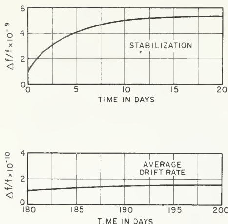
Fig. 21. Initial stabilization period and drift rate of 2.5-MHz precision oscillators.
