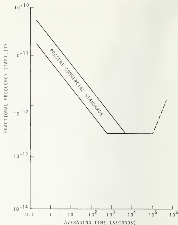
Fig. 4B.6. Stability performance data for commercial rubidium standards.
