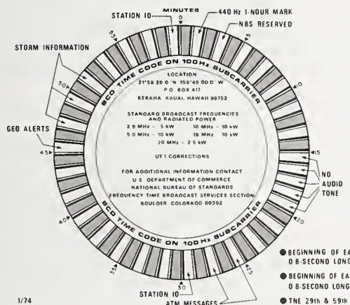
FIGURE 10.10. Hourly broadcast format of WWV (a) and WWVH (b).
