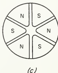
Fig. 3.6. Part (a) gives the energy levels for the ground electronic state ( 1^2S_{1/2} ) of the H atom. Part (b) is a schematic of the H maser. Part (c) is the end view of the hexapolar state selecting magnet typically used in an H maser.
