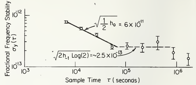
FIGURE 9.5. Hydrogen Maser (NP3), cesium beam (clock 2) comparison, showing the fractional frequency stability as a function of sample time.
