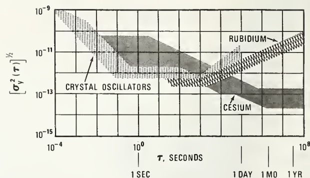
Fig. 2B.6. Stability values of frequency standards, indicating the margin between specified data and performance of selected units.
