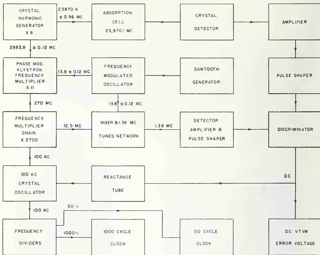
Fig. 10. Block diagram of NBS ammonia clock (courtesy of National Bureau of Standards, Boulder, Colo.).
