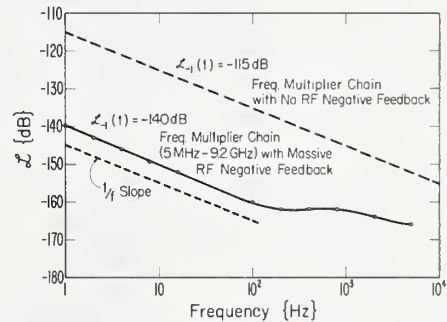
Fig. 3. Normalized spectral density of phase noise power for NBS frequency-multiplier chains.
