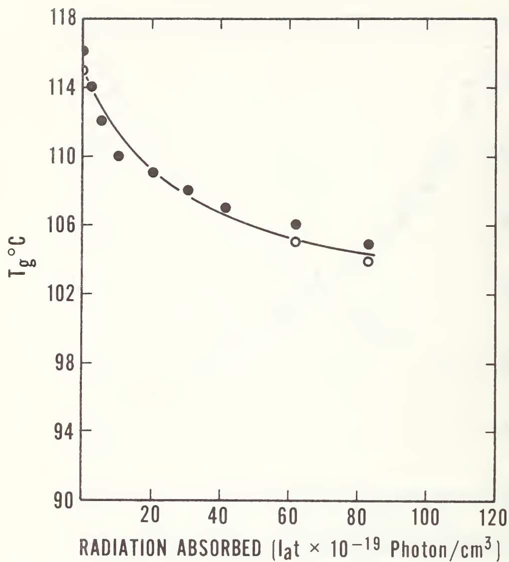
Figure 15. Changes in the glass transition temperature, T_g , of PMMA during irradiation with 300 nm lamps in air; o PMMA I, ● PMMA II.
