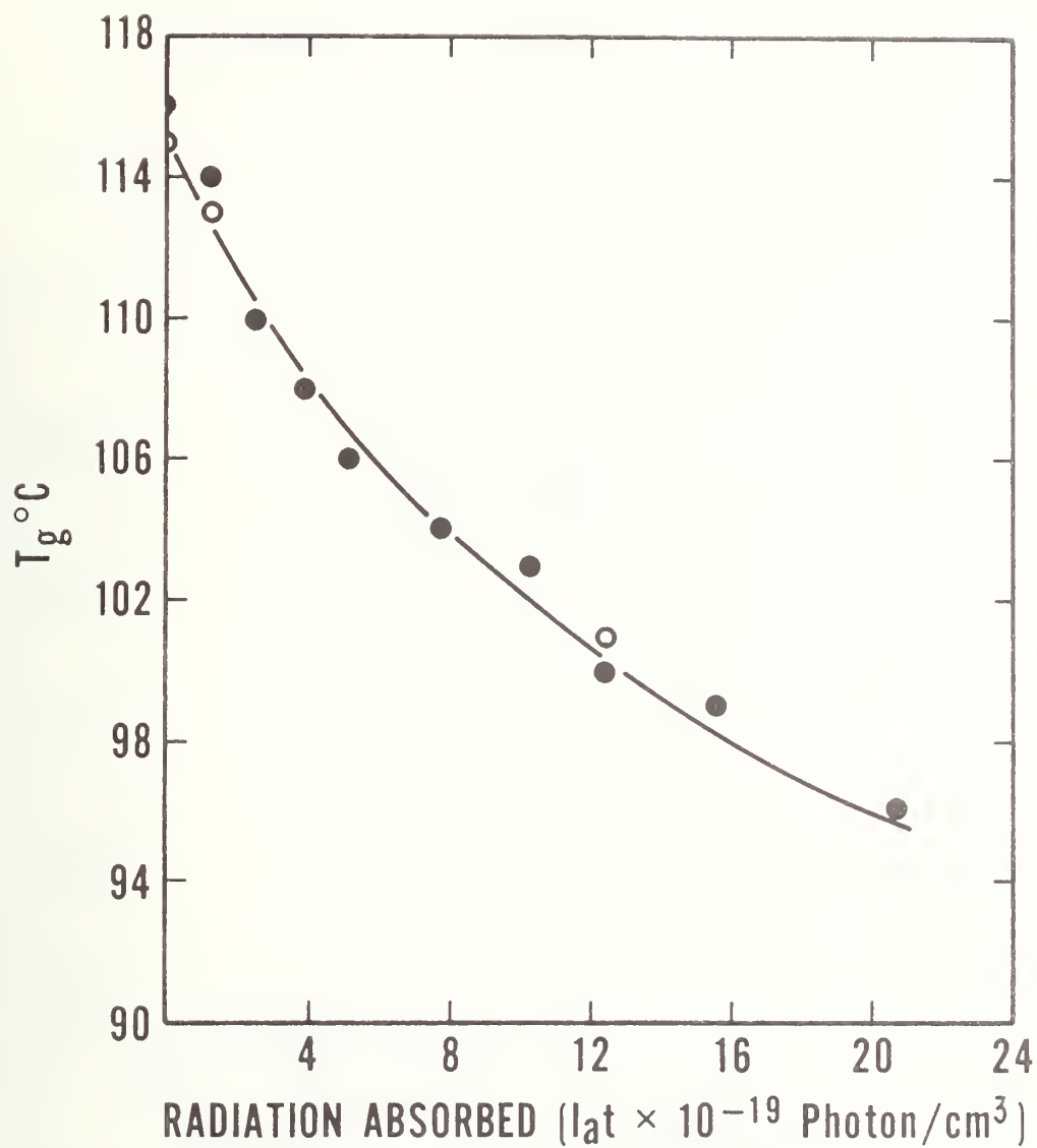
Figure 14. Changes in the glass transition temperature T_g , of PMMA during irradiation with 253.7 nm under vacuum; ○ PMMA I, ● PMMA II.
