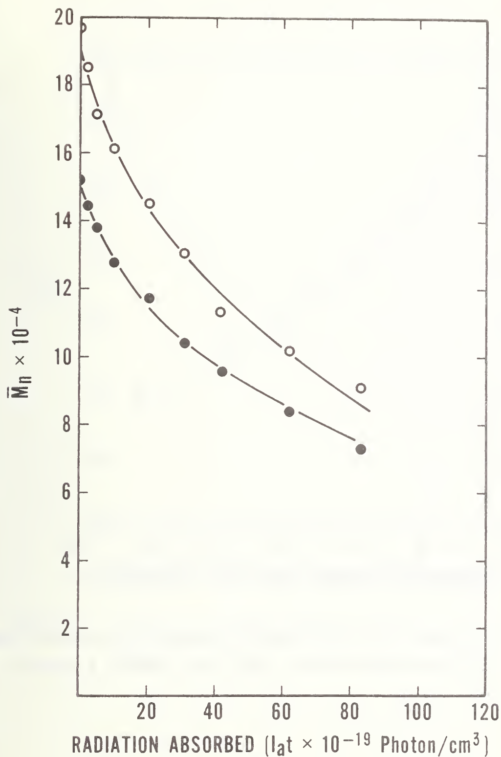
Figure 12. Changes in the number average molecular mass of PMMA during irradiation with 300 nm lamps under vacuum; ● PMMA I, ○ PMMA II.
