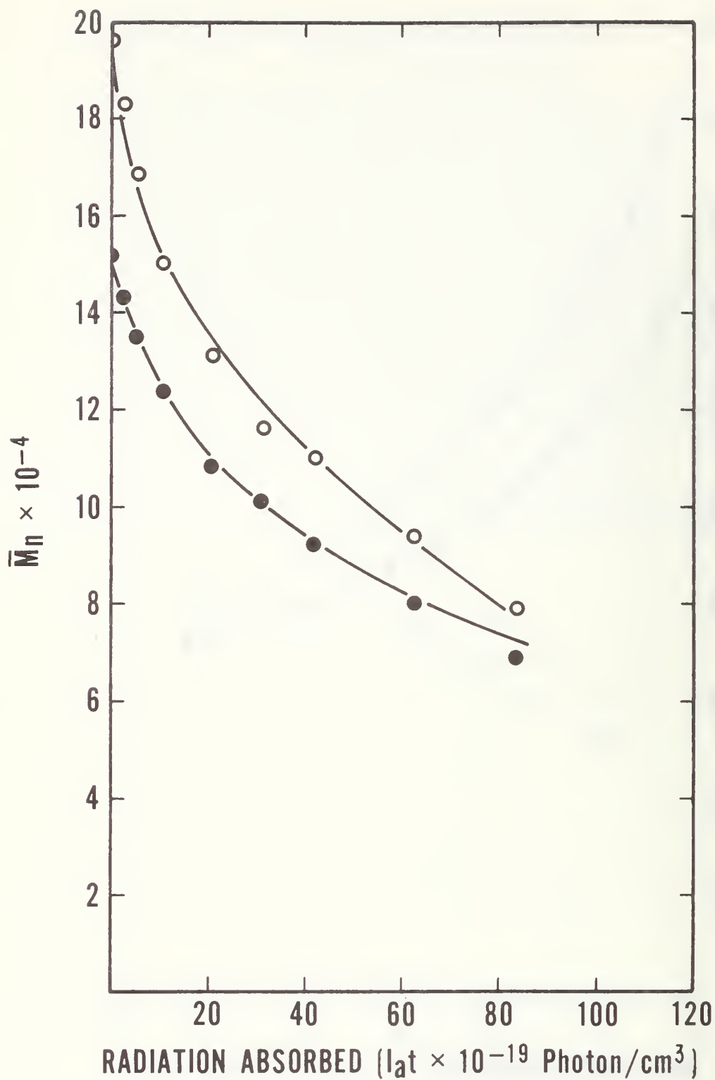
Figure 11. Changes in the number average molecular mass of PMMA during irradiation with 300 nm lamps in air; ● PMMA I, ○ PMMA II.
