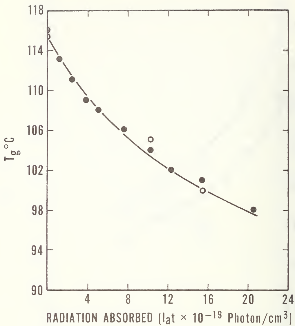
Figure 13. Changes in the glass transition temperature, T_g , of PMMA during irradiation with 253.7 nm lamps in air; o PMMA I, ● PMMA II.
