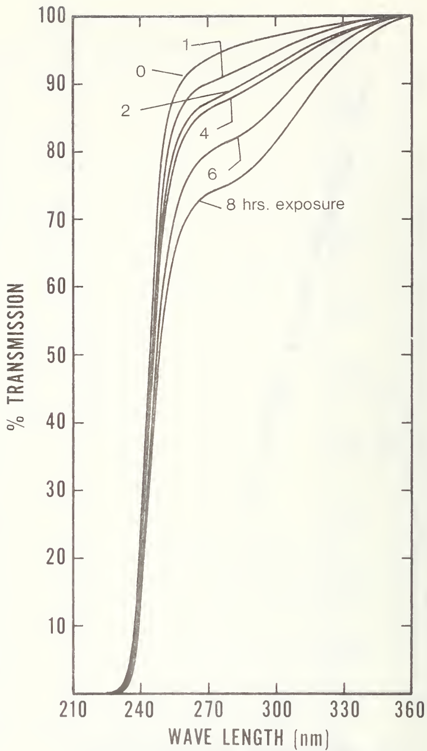
Figure 19. Changes in the ultraviolet spectrum of PMMA II during irradiation with 253.7 nm lamps.
