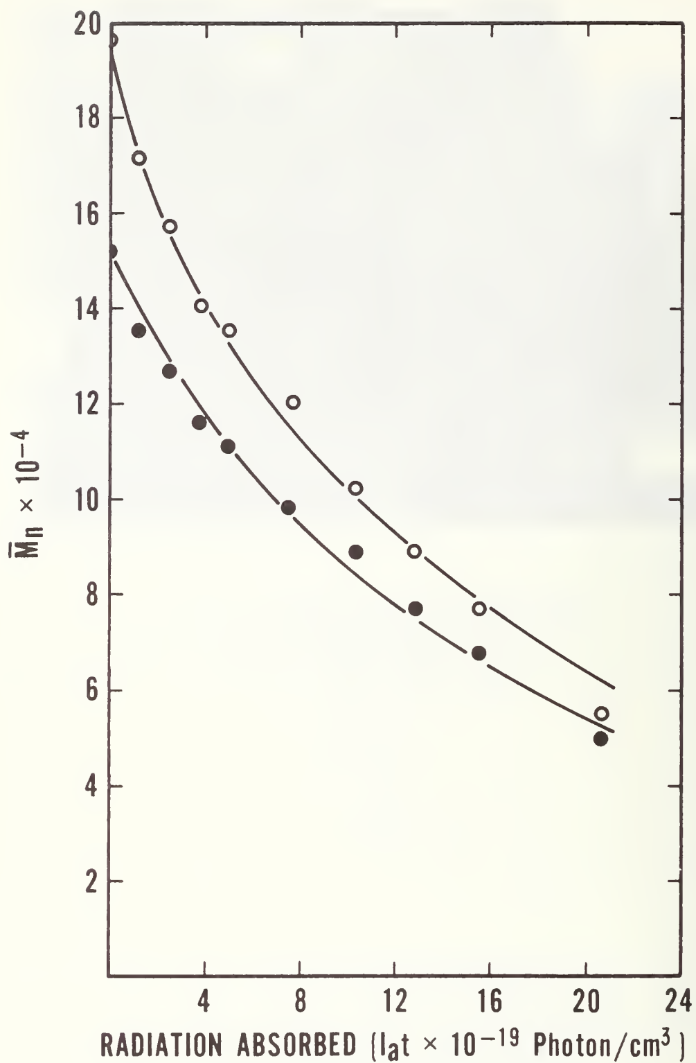
Figure 9. Changes in the number average molecular mass of PMMA during irradiation with 253.7 nm lamps in air; o PMMA I, ● PMMA II.
