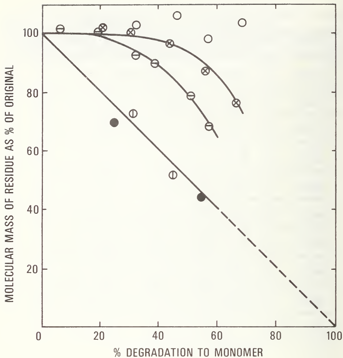
Fig. 1. Grassie [29] . Effect of thermal degradation on the molecular mass of PMMA of various initial molecular mass; \circ 44000, \otimes 94000, \ominus 179000, \oplus 650000, \bullet 725000
