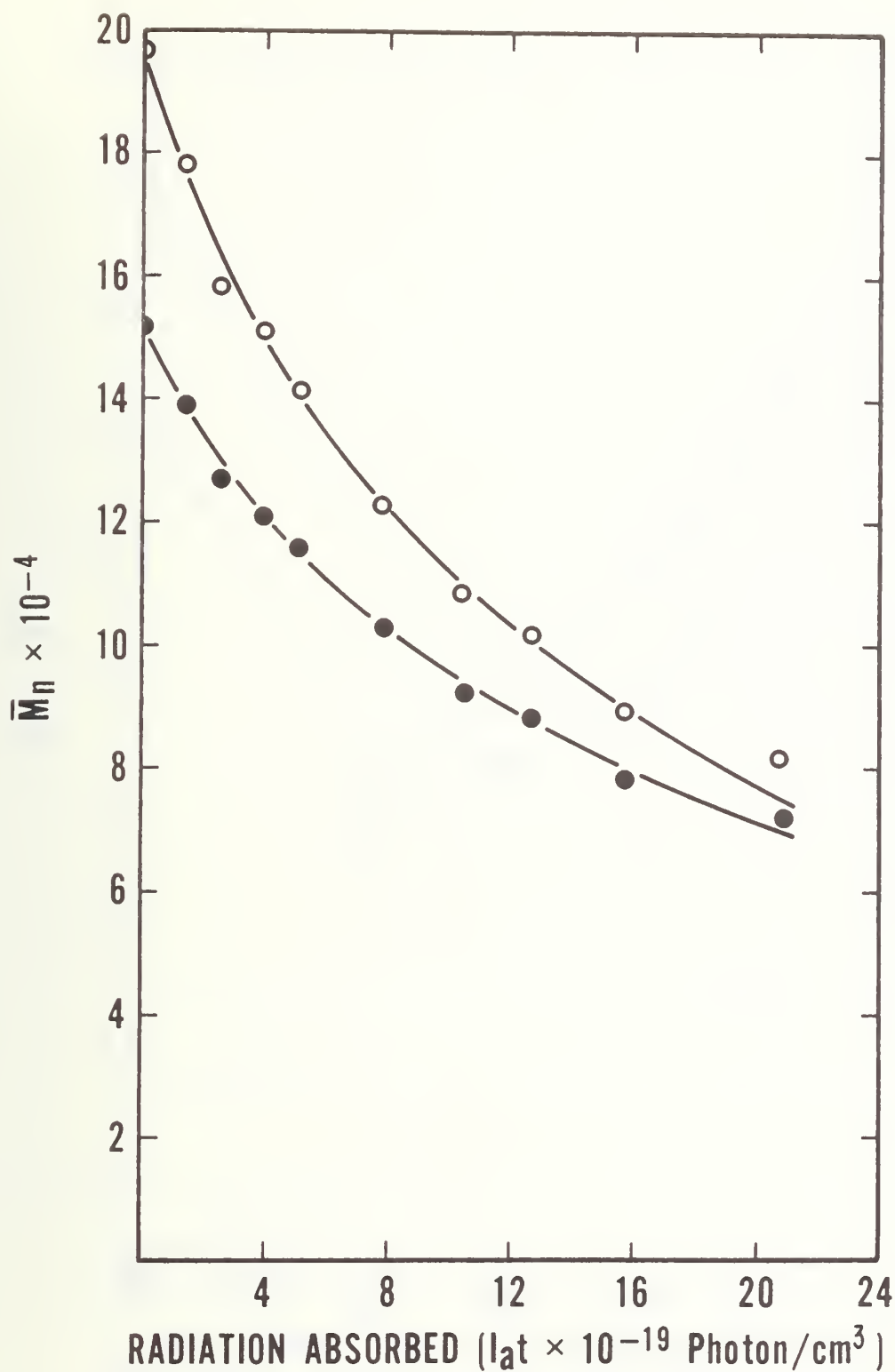
Figure 10. Change in the number average molecular mass of PMMA during irradiation with 253.7 lamps under vacuum; ● PMMA I, ○ PMMA II.
