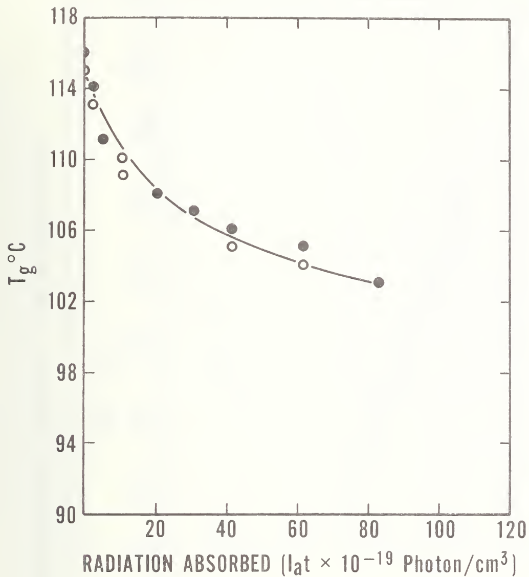
Figure 16. Changes in the glass transition temperature, T_g , of PMMA during irradiation with 300 nm lamps under vacuum; o PMMA I, ● PMMA II.
