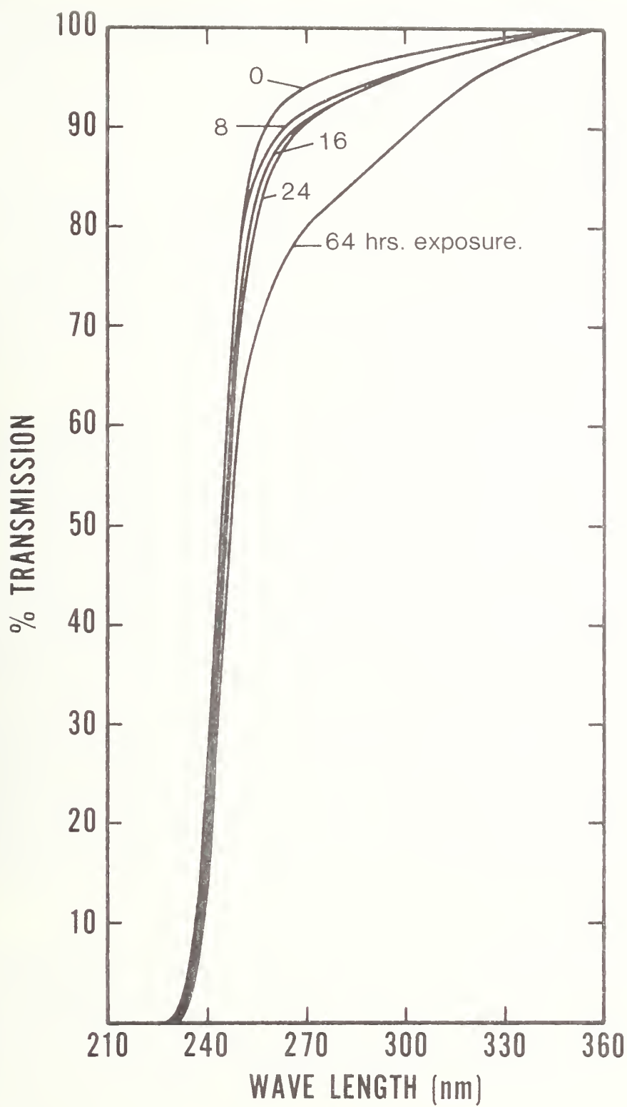
Figure 20. Changes in the ultraviolet spectrum of PMMA II during irradiation with 300 nm lamps.
