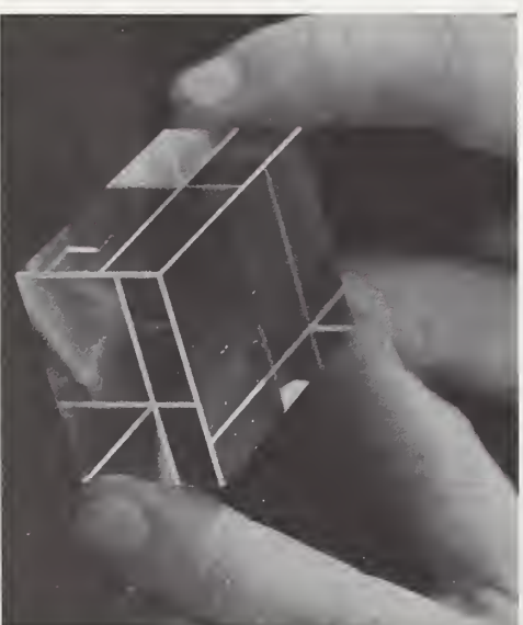
Thomas Proctor determined the velocity of sound in this borosilicate block by measuring the time required for a sound pulse to cross the block and be reflected back to a transducer applied to one of the faces.
