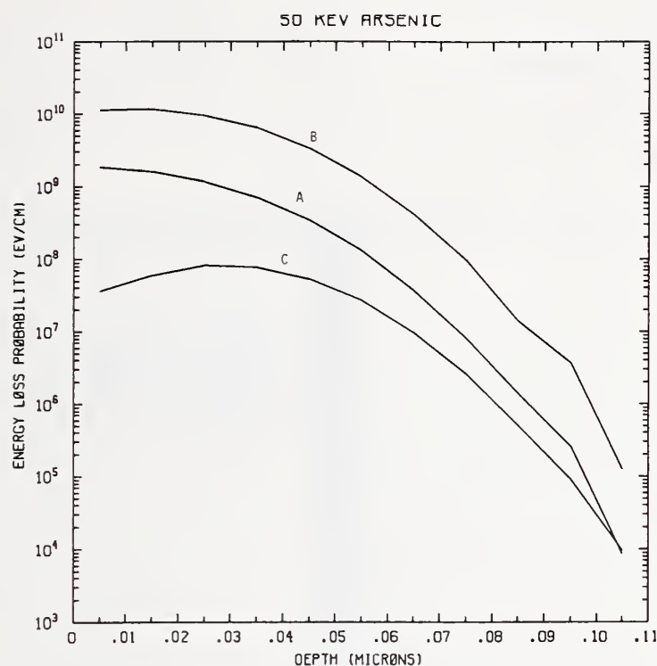
Figure As50-1 One-dimensional probability distributions for energy loss due to electronic excitation (A), displacement damage (B), and phonon excitation (C) for 50 keV arsenic normally incident on a silicon target.
