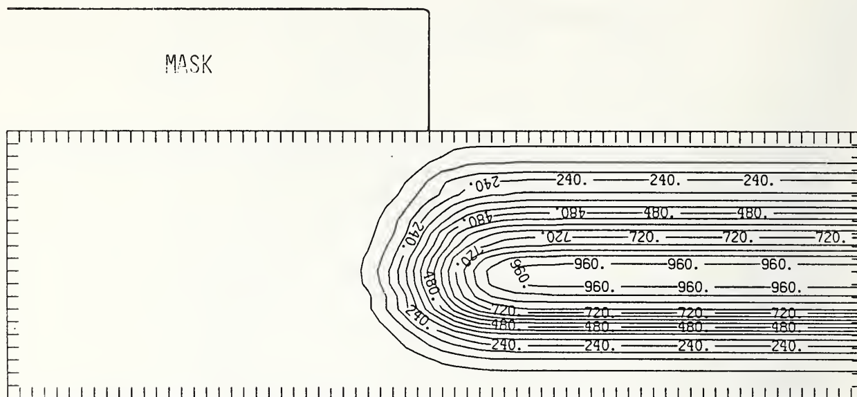
Figure Si150-3 Two-dimensional distribution of 150 keV silicon implanted past a mask edge. The length increment (distance between tick marks) is 0.02 \mu\text{m} and the scale factor is 1000.
