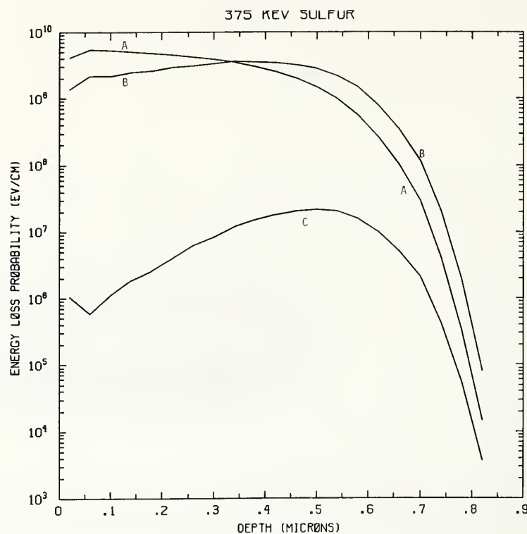
Figure S375-1 One-dimensional probability distributions for energy loss due to electronic excitation (A), displacement damage(B), and phonon excitation (C) for 375 keV sulfur normally incident on a silicon target.
