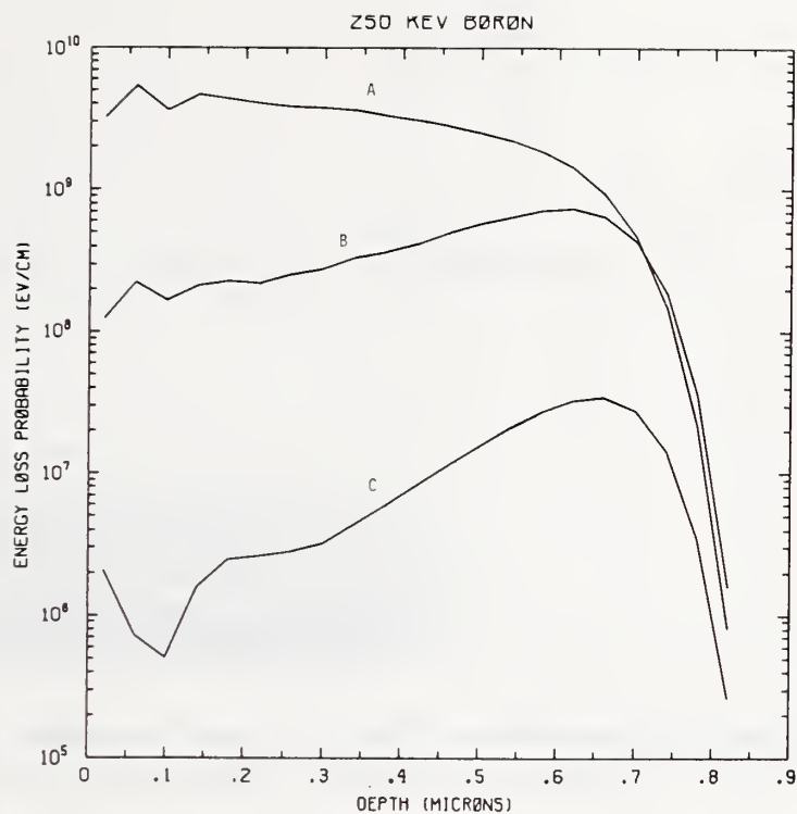
Figure B250-1 One-dimensional probability distributions for energy loss due to electronic excitation (A), displacement damage(B), and phonon excitation (C) for 250 keV boron normally incident on a silicon target.
