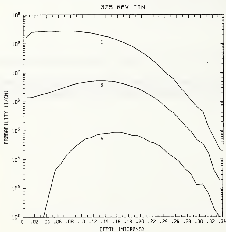
Figure Sn325-2 One-dimensional probability distributions for implanted tin (A), primary silicon displacements (B), and Frenkel pairs (C) for 325 keV tin normally incident on a silicon target.
