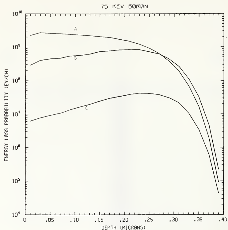
Figure B75-1 One-dimensional probability distributions for energy loss due to electronic excitation (A), displacement damage (B), and phonon excitation (C) for 75 keV boron normally incident on a silicon target.
