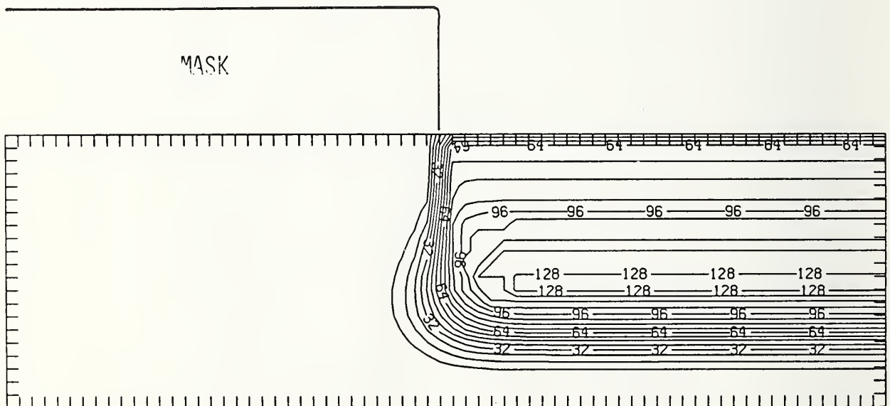
Figure Al350-4 Two-dimensional distribution of Frenkel pairs created by 350 keV aluminum implanted past a mask edge. The length increment (distance between tick marks) is 0.04 \mu\text{m} and the scale factor is 0.1.
