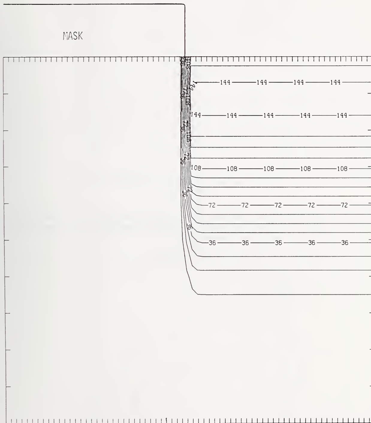
Figure Ge125-4 Two-dimensional distribution of Frenkel pairs created by 125 keV germanium implanted past a mask edge. The length increment (distance between tick marks) is 0.02 \mu\text{m} and the scale factor is 0.1.
