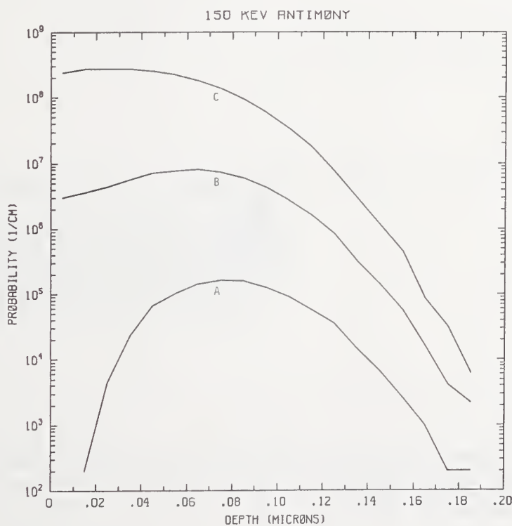
Figure Sb150-2 One-dimensional probability distributions for implanted antimony (A), primary silicon displacements (B), and Frenkel pairs (C) for 150 keV antimony normally incident on a silicon target.
