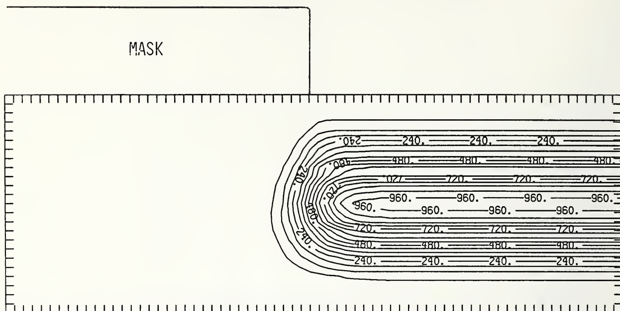
Figure Ga350-3 Two-dimensional distribution of 350 keV gallium implanted past a mask edge. The length increment (distance between tick marks) is 0.02 \mu\text{m} and the scale factor is 1000.
