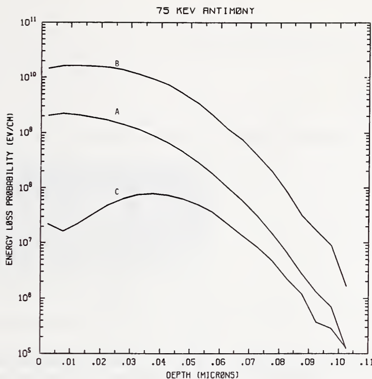
Figure Sb75-1 One-dimensional probability distributions for energy loss due to electronic excitation (A), displacement damage (B), and phonon excitation (C) for 75 keV antimony normally incident on a silicon target.
