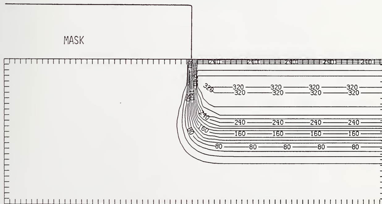
Figure Ge375-4 Two-dimensional distribution of Frenkel pairs created by 375 keV germanium implanted past a mask edge. The length increment (distance between tick marks) is 0.02 \mu\text{m} and the scale factor is 0.1.
