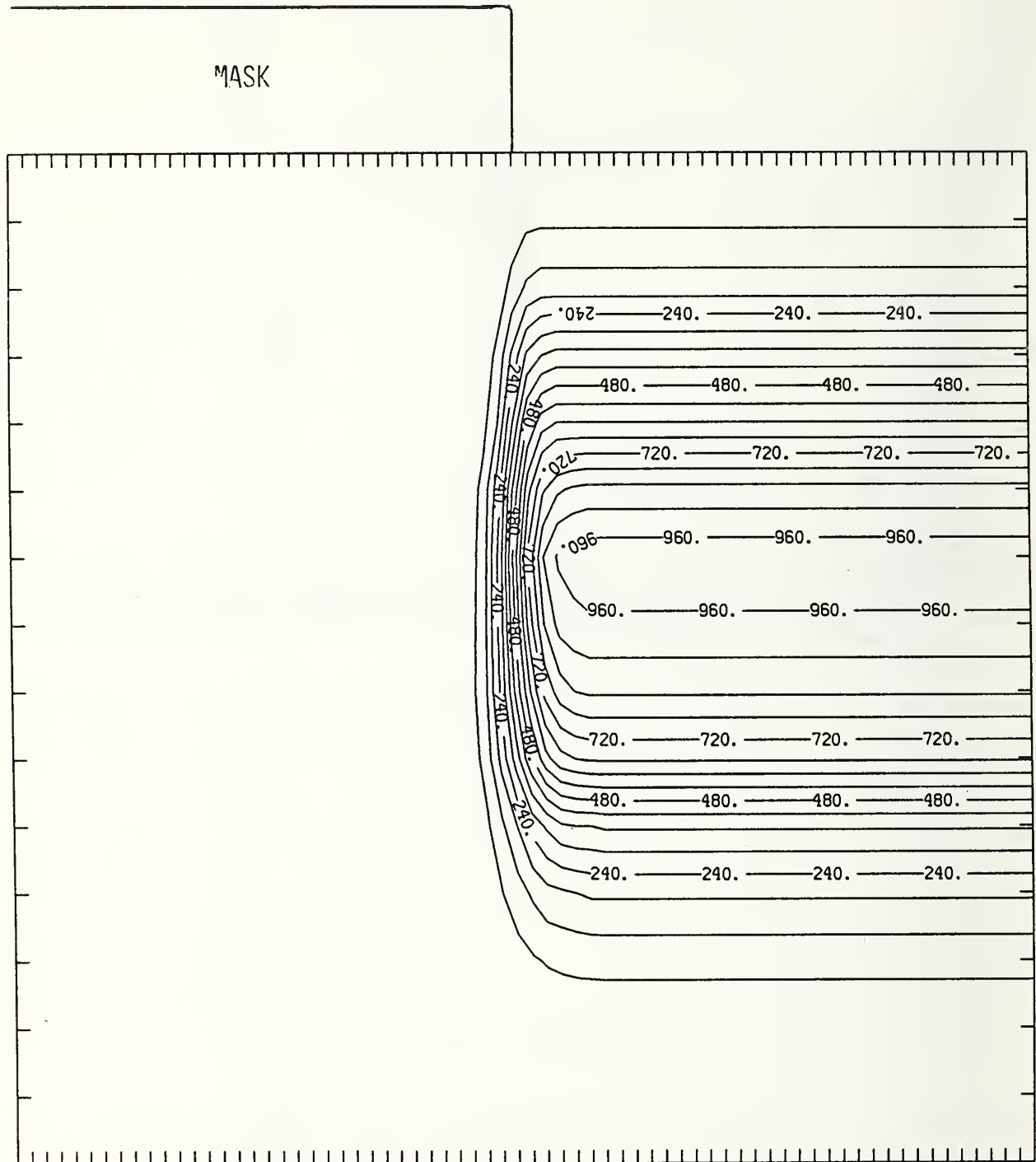
Figure Ga200-3 Two-dimensional distribution of 200 keV gallium implanted past a mask edge. The length increment (distance between tick marks) is 0.02 \mu\text{m} and the scale factor is 1000.
