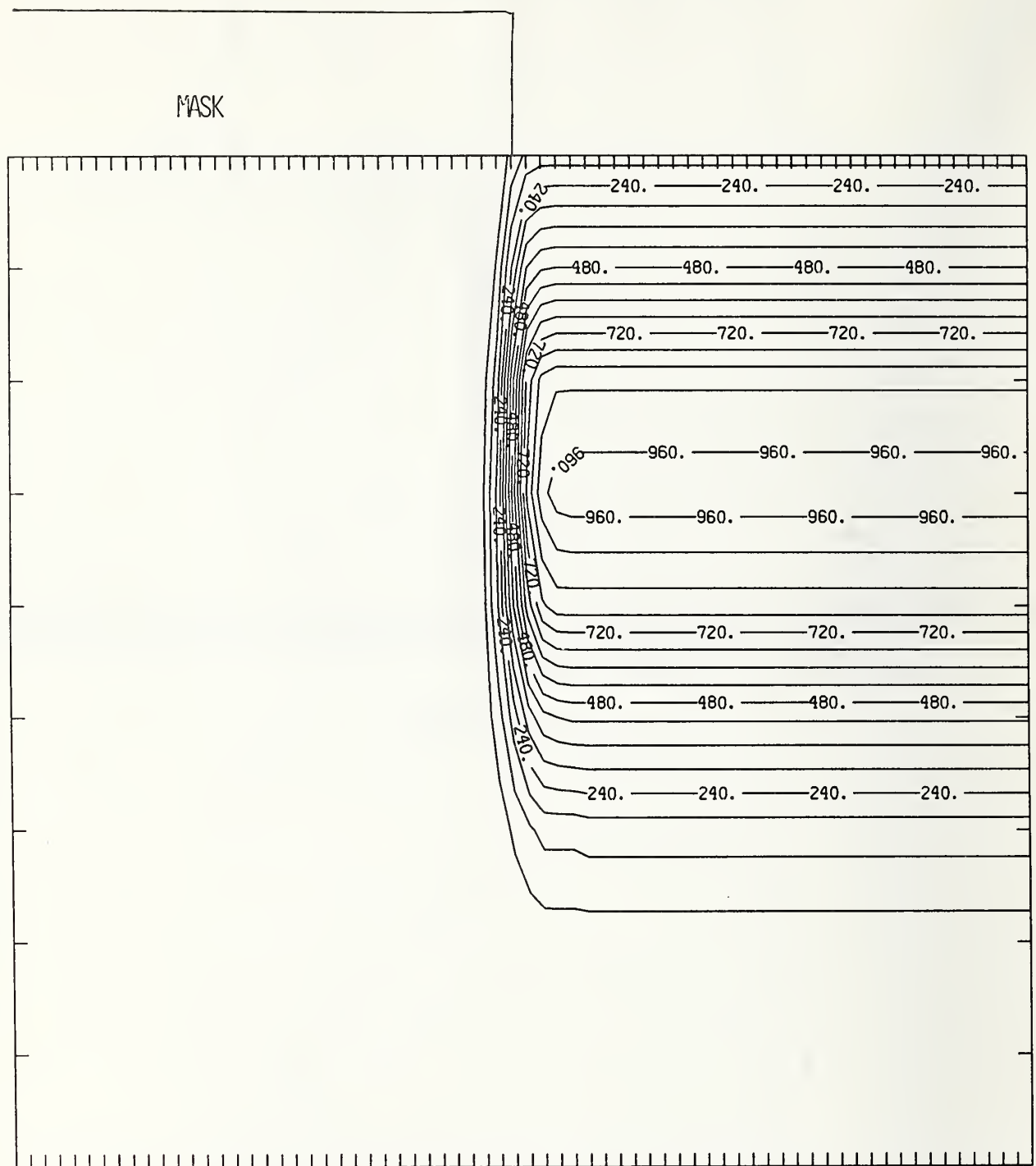
Figure P50-3 Two-dimensional distribution of 50 keV phosphorus implanted past a mask edge. The length increment (distance between tick marks) is 0.02 \mu\text{m} and the scale factor is 1000.
