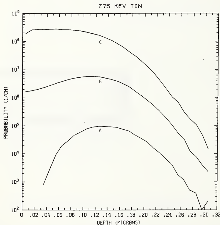
Figure Sn275-2 One-dimensional probability distributions for implanted tin (A), primary silicon displacements (B), and Frenkel pairs (C) for 275 keV tin normally incident on a silicon target.
