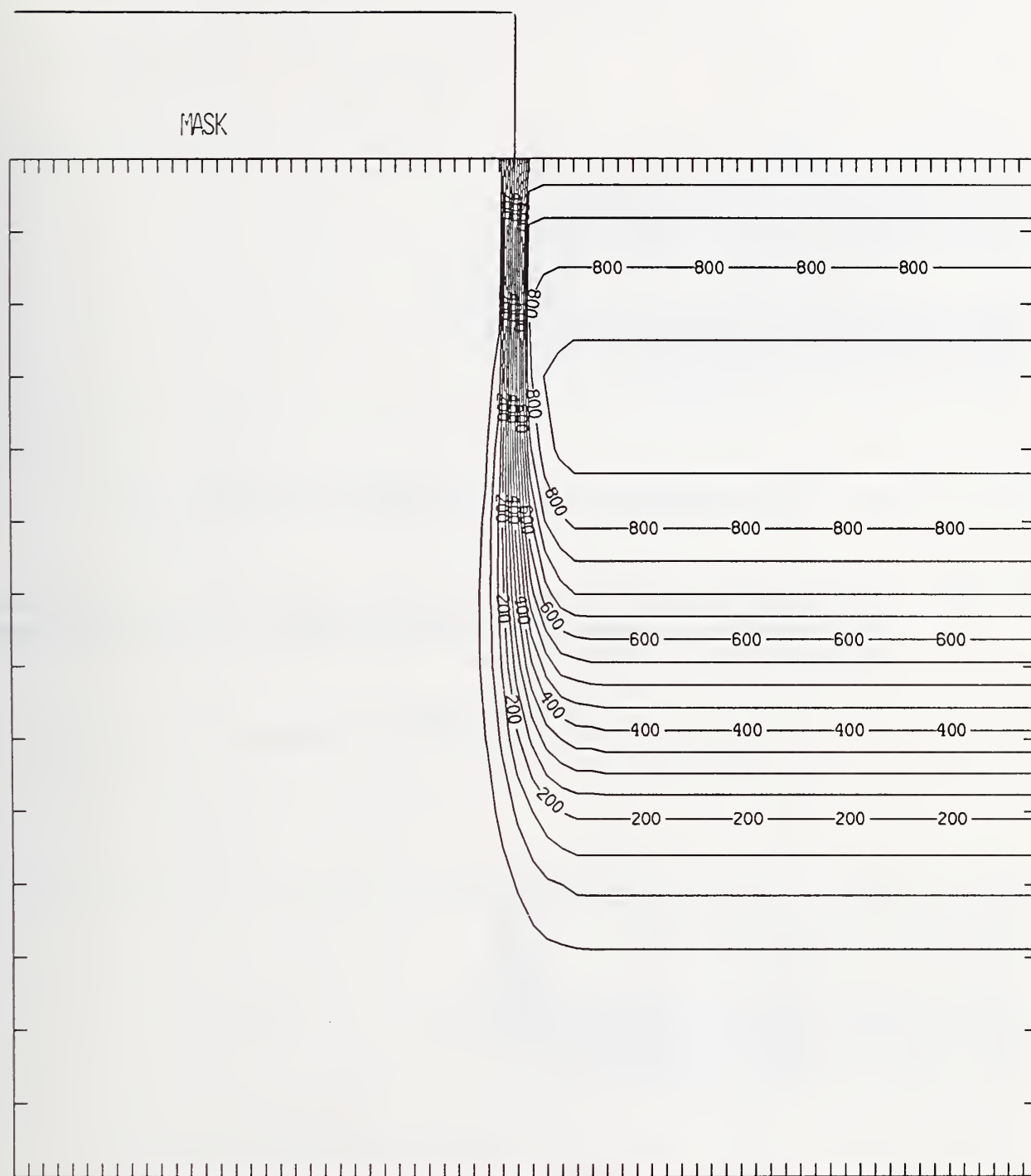
Figure P100-4 Two-dimensional distribution of Frenkel pairs created by 100 keV phosphorus implanted past a mask edge. The length increment (distance between tick marks) is 0.02 \mu\text{m} and the scale factor is 1.
