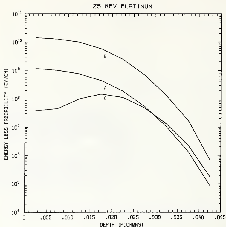
Figure Pt25-1 One-dimensional probability distributions for energy loss due to electronic excitation (A), displacement damage(B), and phonon excitation (C) for 25 keV platinum normally incident on a silicon target.
