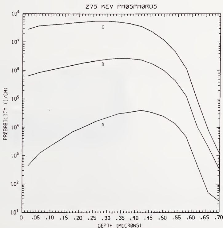
Figure P275-2 One-dimensional probability distributions for implanted phosphorus (A), primary silicon displacements (B), and Frenkel pairs (C) for 275 keV phosphorus normally incident on a silicon target.
