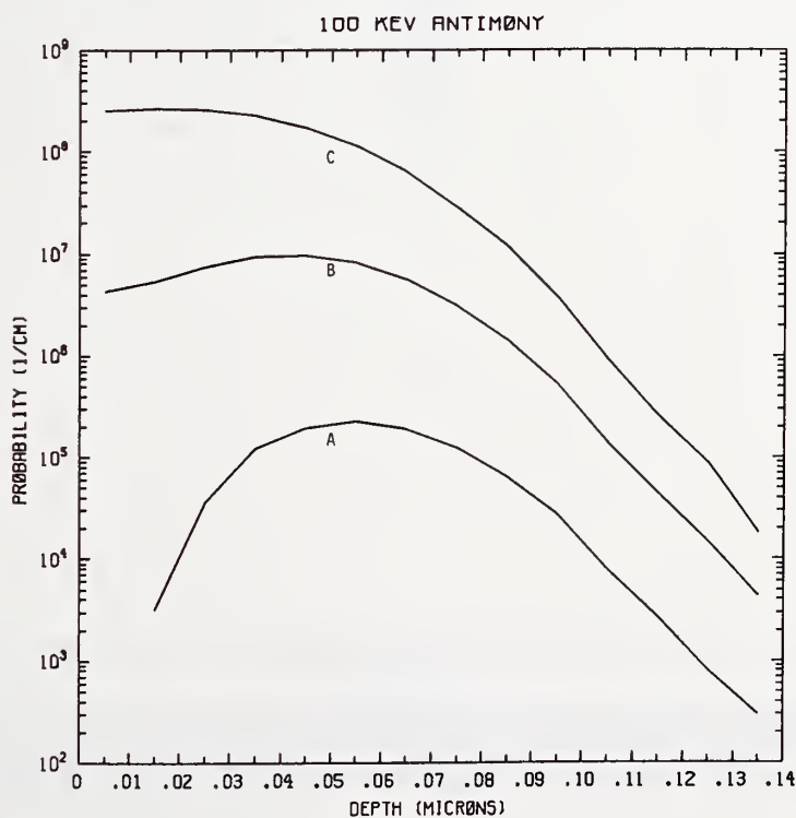
Figure Sb100-2 One-dimensional probability distributions for implanted antimony (A), primary silicon displacements (B), and Frenkel pairs (C) for 100 keV antimony normally incident on a silicon target.
