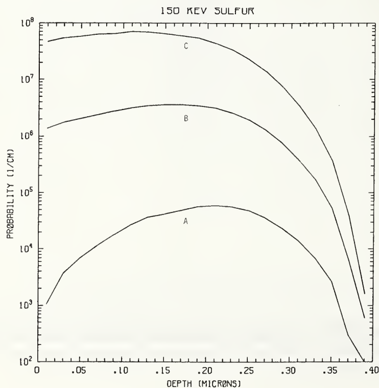
Figure S150-2 One-dimensional probability distributions for implanted sulfur (A), primary silicon displacements (B), and Frenkel pairs (C) for 150 keV sulfur normally incident on a silicon target.
