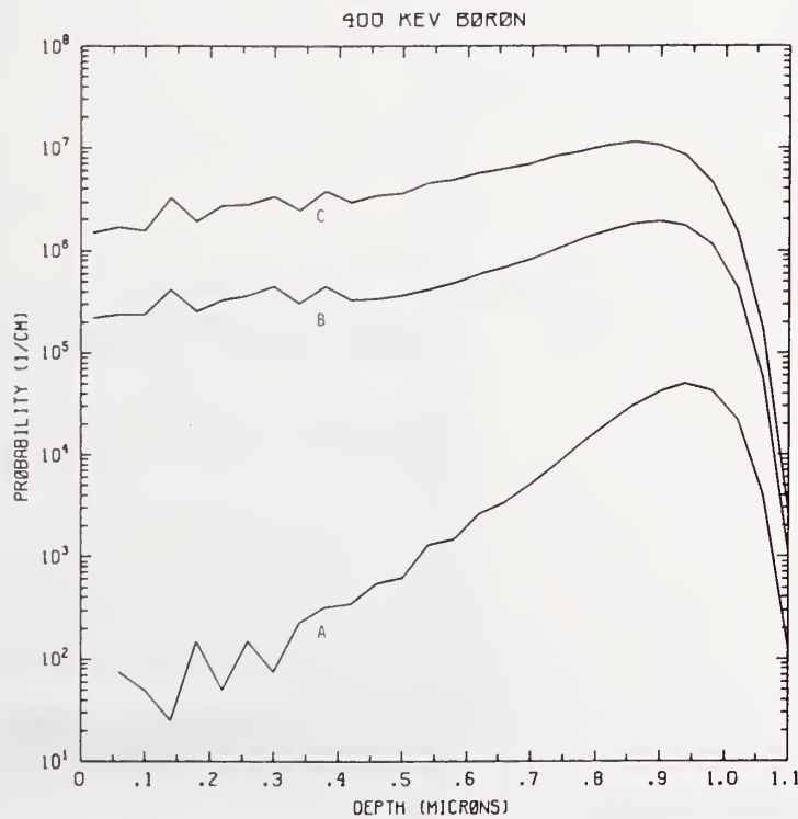
Figure B400-2 One-dimensional probability distributions for implanted boron (A), primary silicon displacements (B), and Frenkel pairs (C) for 400 keV boron normally incident on a silicon target.
