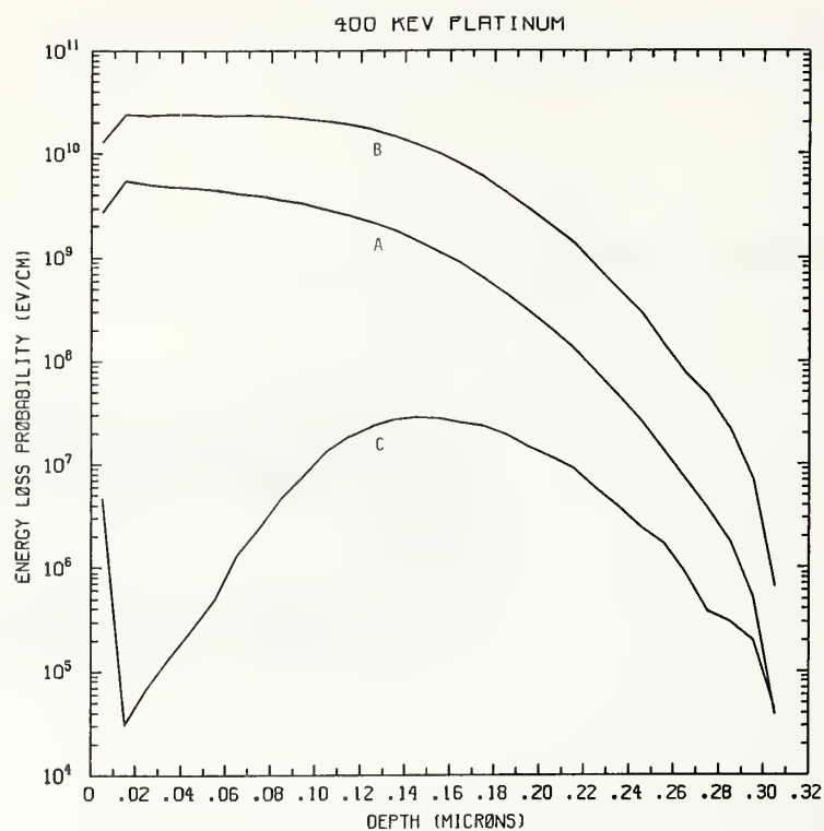
Figure Pt400-1 One-dimensional probability distributions for energy loss due to electronic excitation (A), displacement damage (B), and phonon excitation (C) for 400 keV platinum normally incident on a silicon target.
