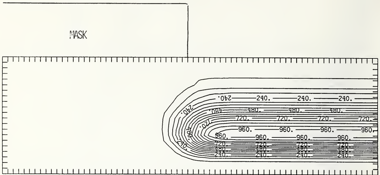
Figure P375-3 Two-dimensional distribution of 375 keV phosphorus implanted past a mask edge. The length increment (distance between tick marks) is 0.04 \mu\text{m} and the scale factor is 1000.
