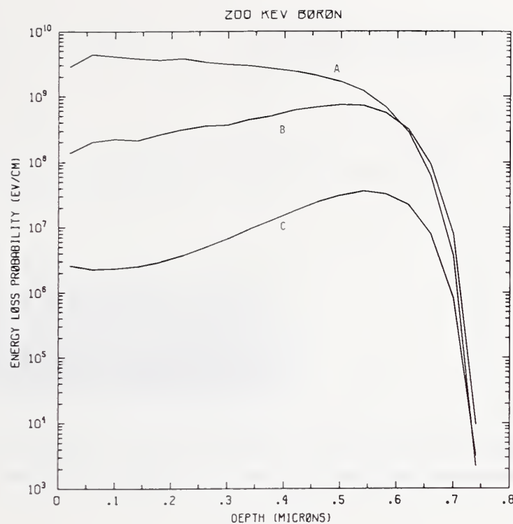
Figure B200-1 One-dimensional probability distributions for energy loss due to electronic excitation (A), displacement damage(B), and phonon excitation (C) for 200 keV boron normally incident on a silicon target.
