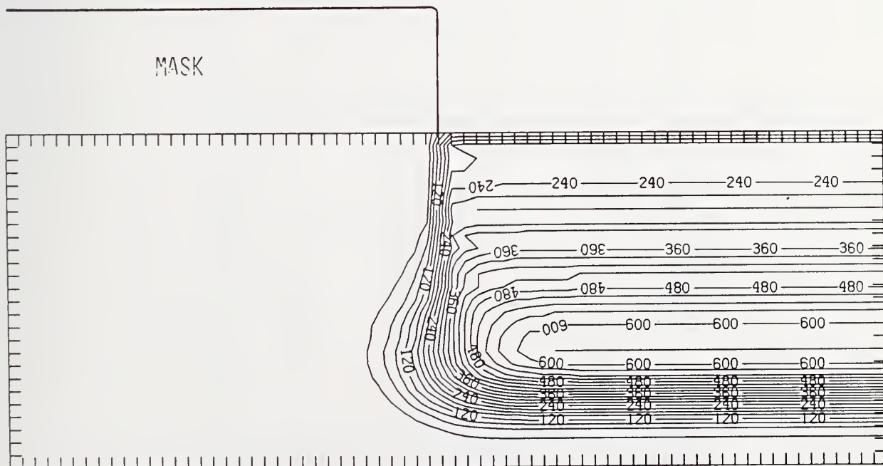
Figure O325-4 Two-dimensional distribution of Frenkel pairs created by 325 keV oxygen implanted past a mask edge. The length increment (distance between tick marks) is 0.04 \mu\text{m} and the scale factor is 1.
