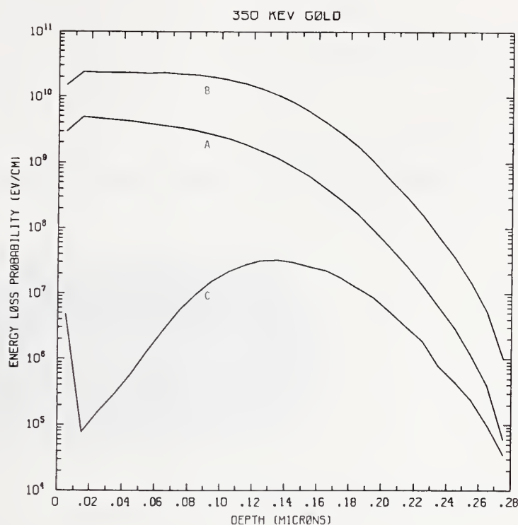
Figure Au350-1 One-dimensional probability distributions for energy loss due to electronic excitation (A), displacement damage(B), and phonon excitation (C) for 350 keV gold normally incident on a silicon target.
