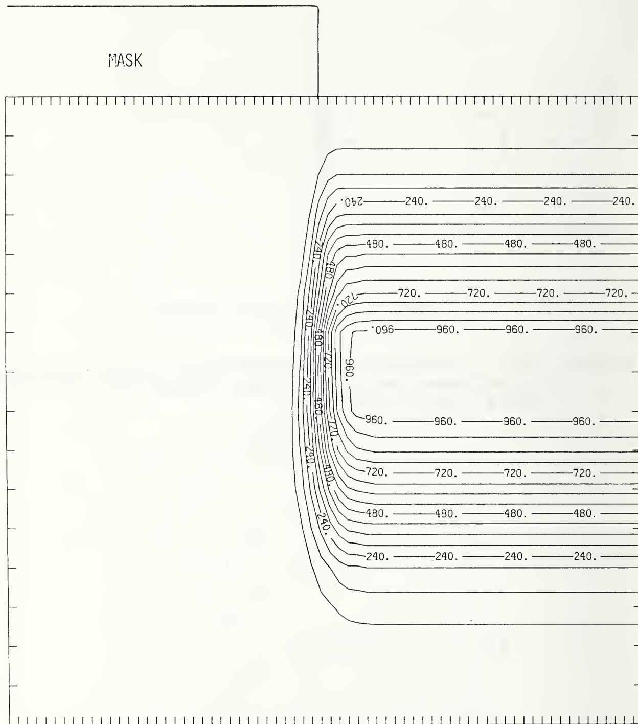
Figure Ge225-3 Two-dimensional distribution of 225 keV germanium implanted past a mask edge. The length increment (distance between tick marks) is 0.02 \mu\text{m} and the scale factor is 1000.
