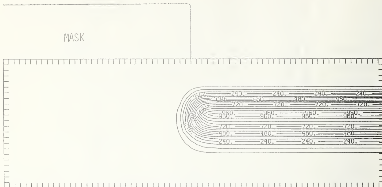
Figure Au250-3 Two-dimensional distribution of 250 keV gold implanted past a mask edge. The length increment (distance between tick marks) is 0.01 \mu\text{m} and the scale factor is 1000.
