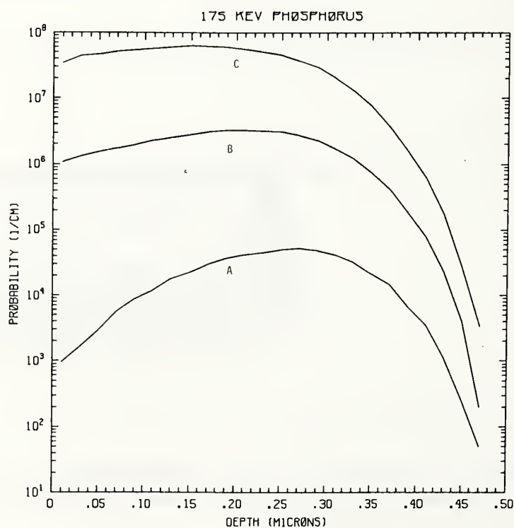
Figure P175-2 One-dimensional probability distributions for implanted phosphorus (A), primary silicon displacements (B), and Frenkel pairs (C) for 175 keV phosphorus normally incident on a silicon target.
