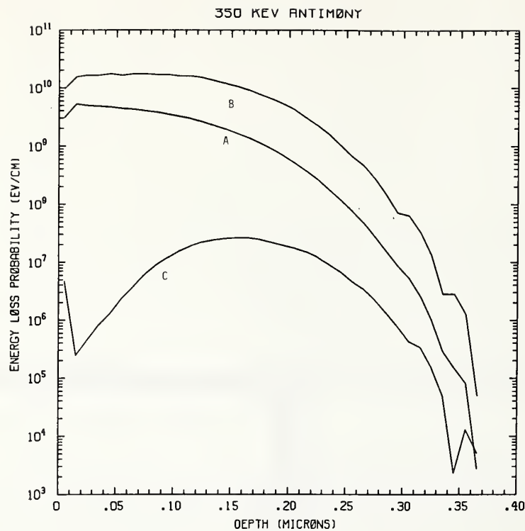
Figure Sb350-1 One-dimensional probability distributions for energy loss due to electronic excitation (A), displacement damage (B), and phonon excitation (C) for 350 keV antimony normally incident on a silicon target.
