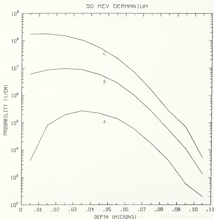
Figure Ge50-2 One-dimensional probability distributions for implanted germanium (A), primary silicon displacements (B), and Frenkel pairs (C) for 50 keV germanium normally incident on a silicon target.
