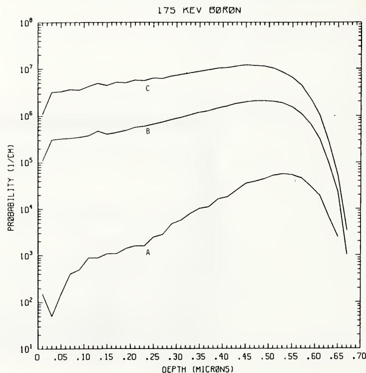
Figure B175-2 One-dimensional probability distributions for implanted boron (A), primary silicon displacements (B), and Frenkel pairs (C) for 175 keV boron normally incident on a silicon target.
