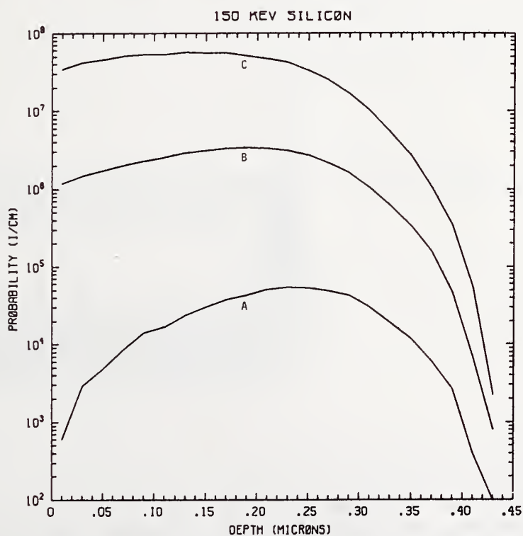
Figure Si150-2 One-dimensional probability distributions for implanted silicon (A), primary silicon displacements (B), and Frenkel pairs (C) for 150 keV silicon normally incident on a silicon target.
