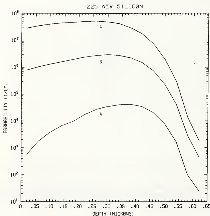
Figure Si225-2 One-dimensional probability distributions for implanted silicon (A), primary silicon displacements (B), and Frenkel pairs (C) for 225 keV silicon normally incident on a silicon target.
