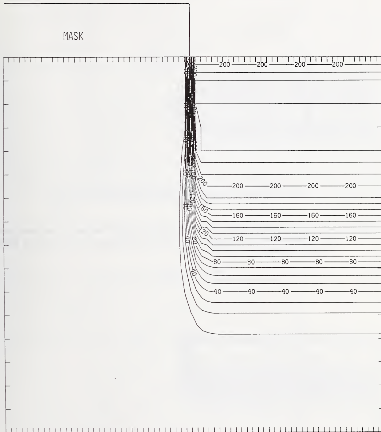
Figure Ge225-4 Two-dimensional distribution of Frenkel pairs created by 225 keV germanium implanted past a mask edge. The length increment (distance between tick marks) is 0.02\ \mu\text{m} and the scale factor is 0.1.
