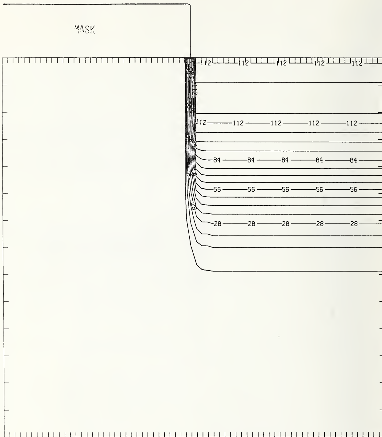
Figure Sn100-4 Two-dimensional distribution of Frenkel pairs created by 100 keV tin implanted past a mask edge. The length increment (distance between tick marks) is 0.01 \mu\text{m} and the scale factor is 0.1.
