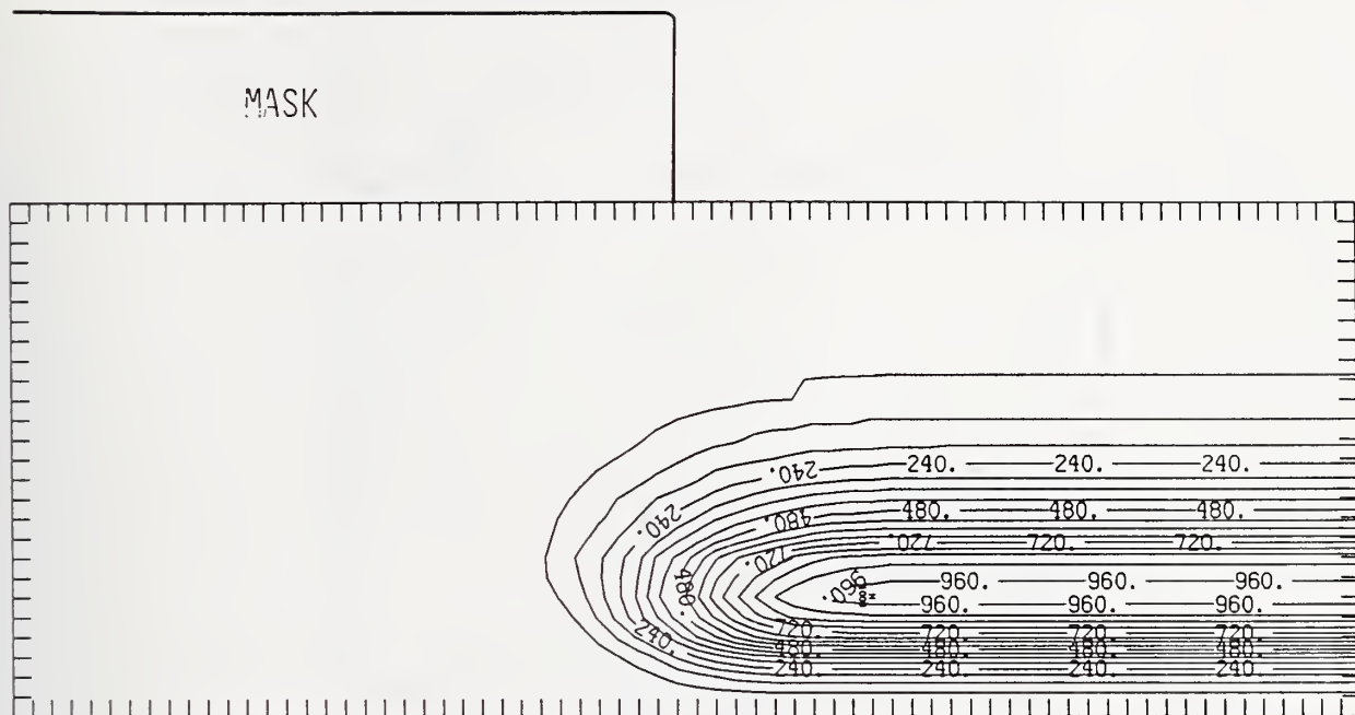
Figure O325-3 Two-dimensional distribution of 325 keV oxygen implanted past a mask edge. The length increment (distance between tick marks) is 0.04 \mu\text{m} and the scale factor is 1000.
