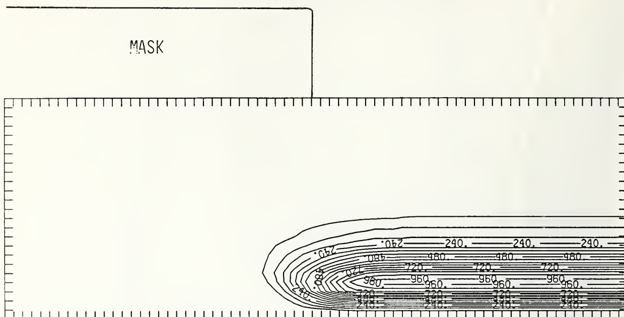
Figure B325-3 Two-dimensional distribution of 325 keV boron implanted past a mask edge. The length increment (distance between tick marks) is 0.04 \mu\text{m} and the scale factor is 1000.
