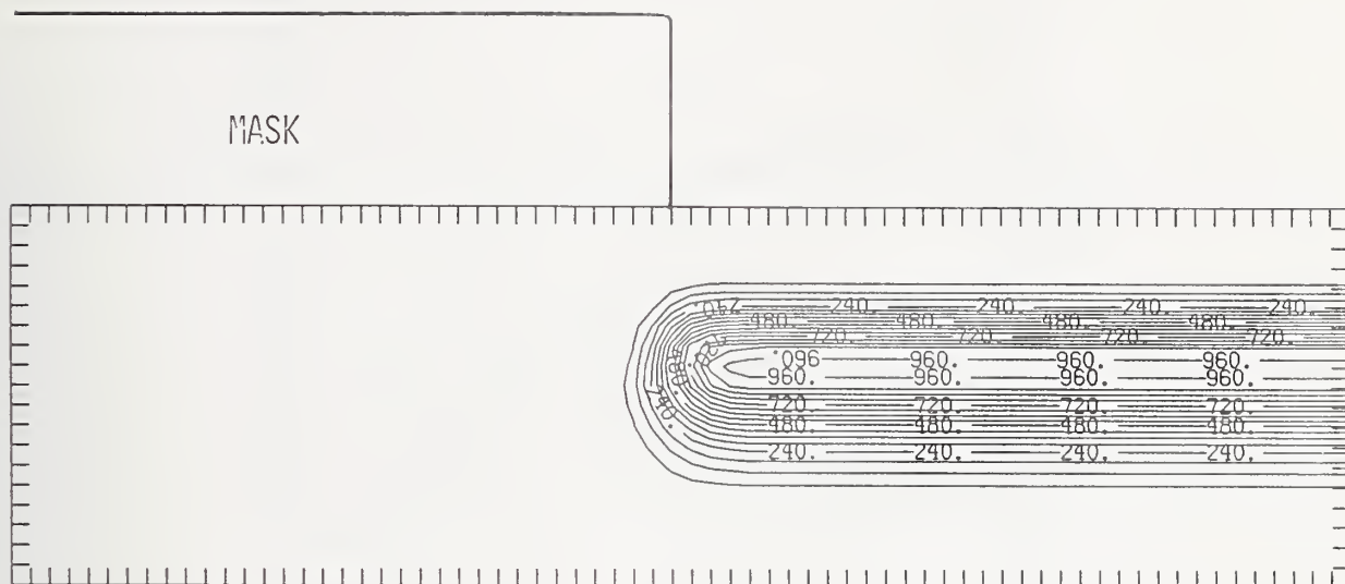
Figure Pt75-3 Two-dimensional distribution of 75 keV platinum implanted past a mask edge. The length increment (distance between tick marks) is 0.005\text{ }\mu\text{m} and the scale factor is 1000.
