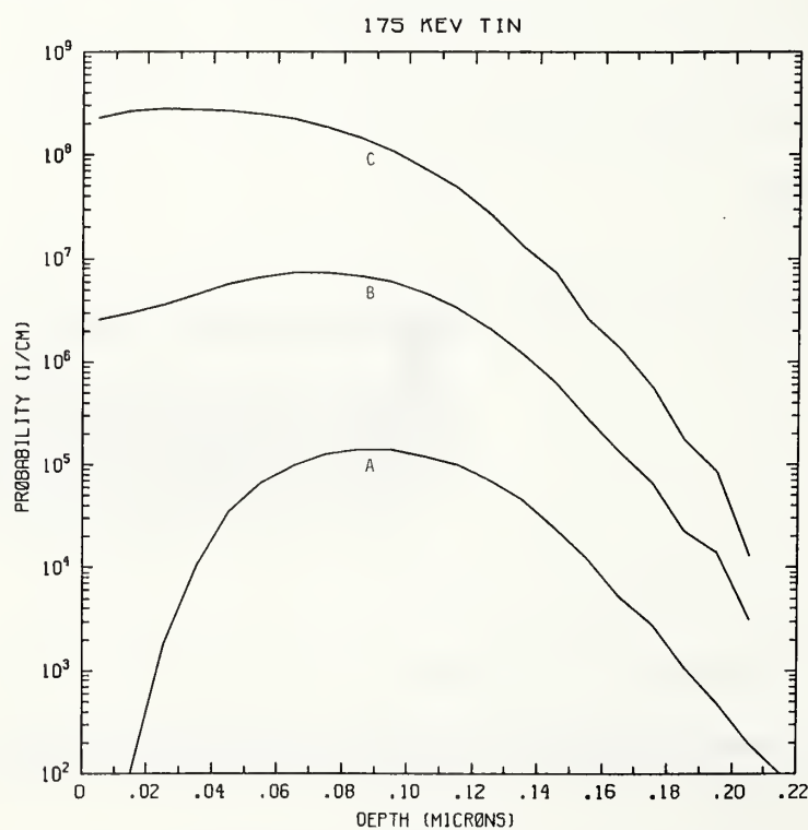
Figure Sn175-2 One-dimensional probability distributions for implanted tin (A), primary silicon displacements (B), and Frenkel pairs (C) for 175 keV tin normally incident on a silicon target.
