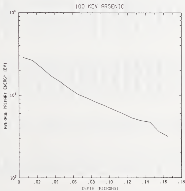
Figure 13. Average energy per primary resulting from 100-keV arsenic in silicon.
