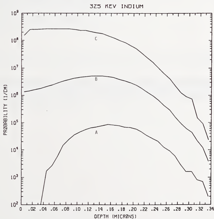
Figure In325-2 One-dimensional probability distributions for implanted indium (A), primary silicon displacements (B), and Frenkel pairs (C) for 325 keV indium normally incident on a silicon target.
