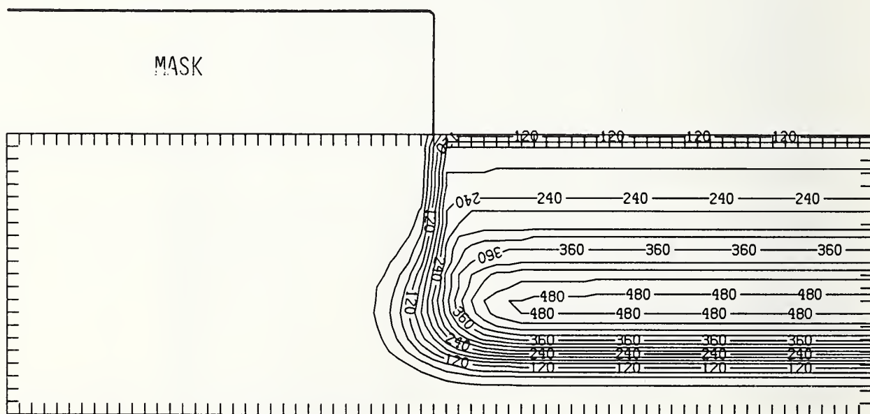
Figure N225-4 Two-dimensional distribution of Frenkel pairs created by 225 keV nitrogen implanted past a mask edge. The length increment (distance between tick marks) is 0.04 \mu\text{m} and the scale factor is 1.
