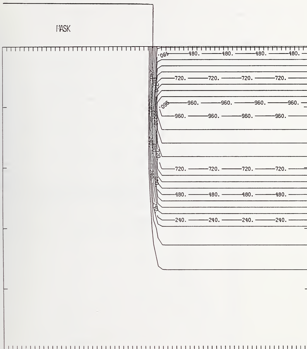
Figure P25-3 Two-dimensional distribution of 25 keV phosphorus implanted past a mask edge. The length increment (distance between tick marks) is 0.02 \mu\text{m} and the scale factor is 1000.
