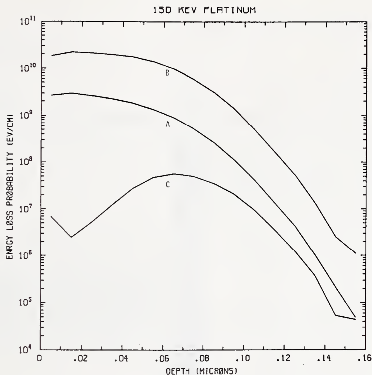
Figure Pt150-1 One-dimensional probability distributions for energy loss due to electronic excitation (A), displacement damage (B), and phonon excitation (C) for 150 keV platinum normally incident on a silicon target.
