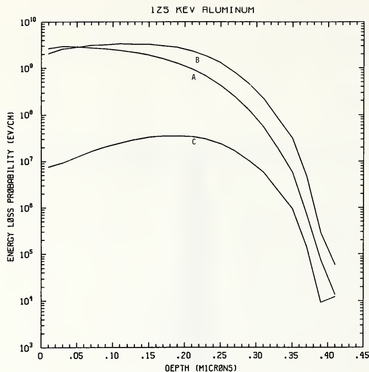
Figure A1125-1 One-dimensional probability distributions for energy loss due to electronic excitation (A), displacement damage (B), and phonon excitation (C) for 125 keV aluminum normally incident on a silicon target.
