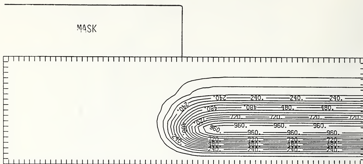
Figure Al325-3 Two-dimensional distribution of 325 keV aluminum implanted past a mask edge. The length increment (distance between tick marks) is 0.04 \mu\text{m} and the scale factor is 1000.
