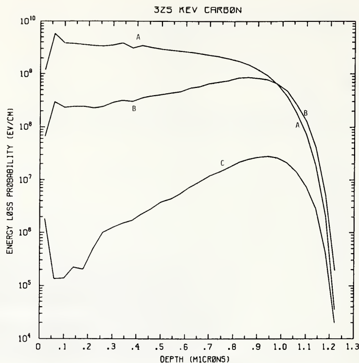
Figure C325-1 One-dimensional probability distributions for energy loss due to electronic excitation (A), displacement damage (B), and phonon excitation (C) for 325 keV carbon normally incident on a silicon target.
