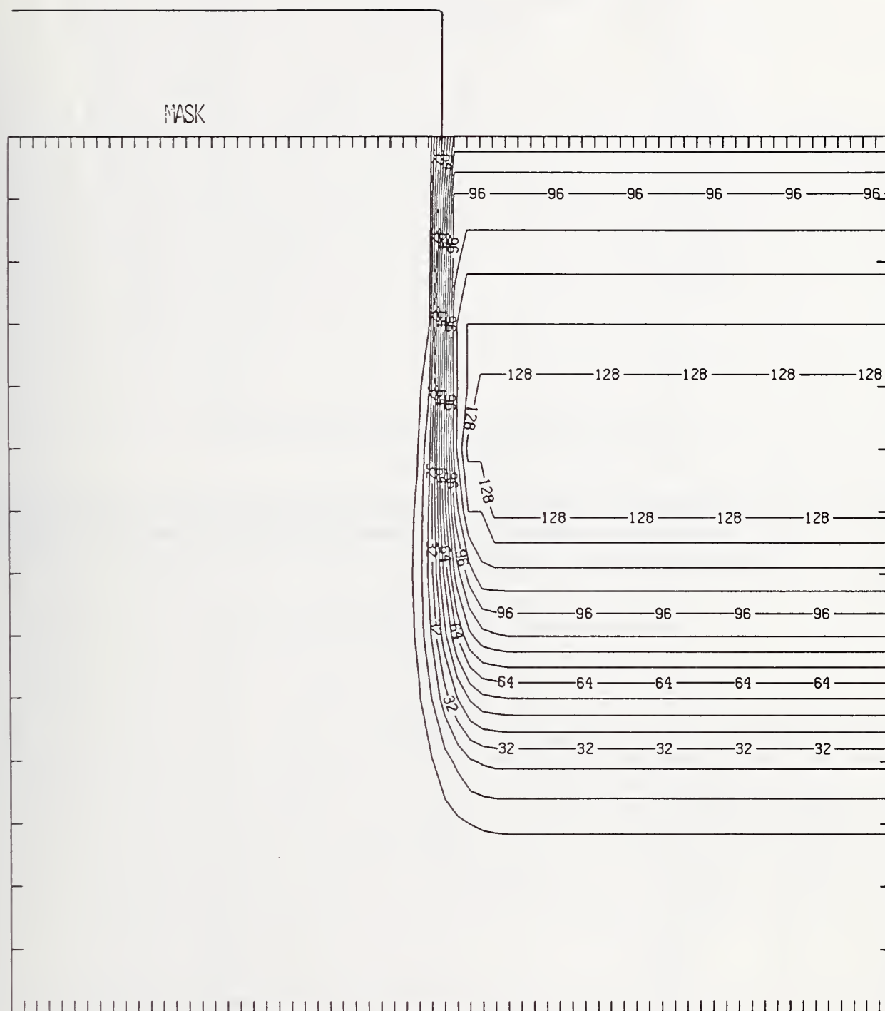
Figure P225-4 Two-dimensional distribution of Frenkel pairs created by 225 keV phosphorus implanted past a mask edge. The length increment (distance between tick marks) is 0.04 \mu\text{m} and the scale factor is 0.1.
