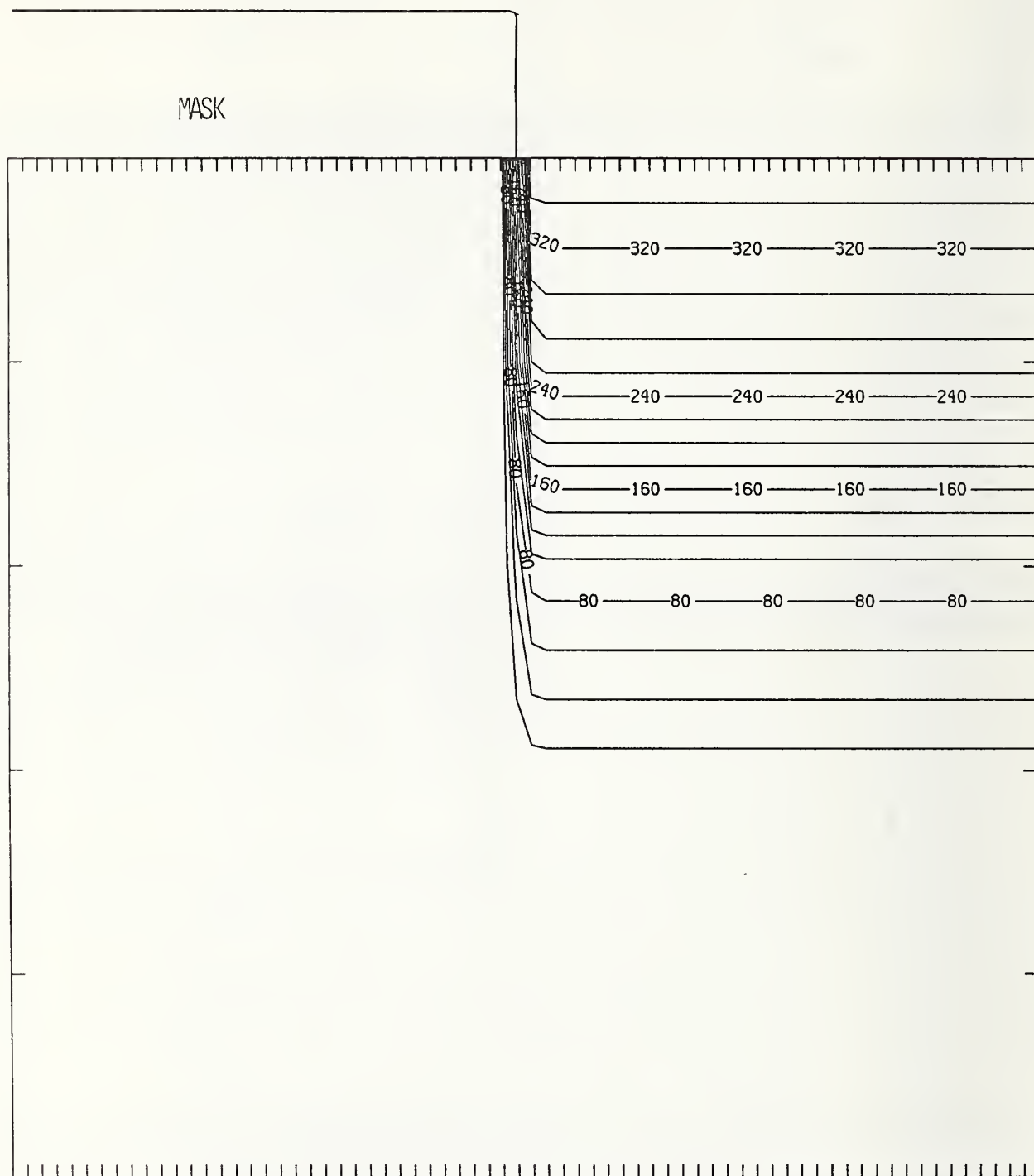
Figure P25-4 Two-dimensional distribution of Frenkel pairs created by 25 keV phosphorus implanted past a mask edge. The length increment (distance between tick marks) is 0.02 \mu\text{m} and the scale factor is 1.
