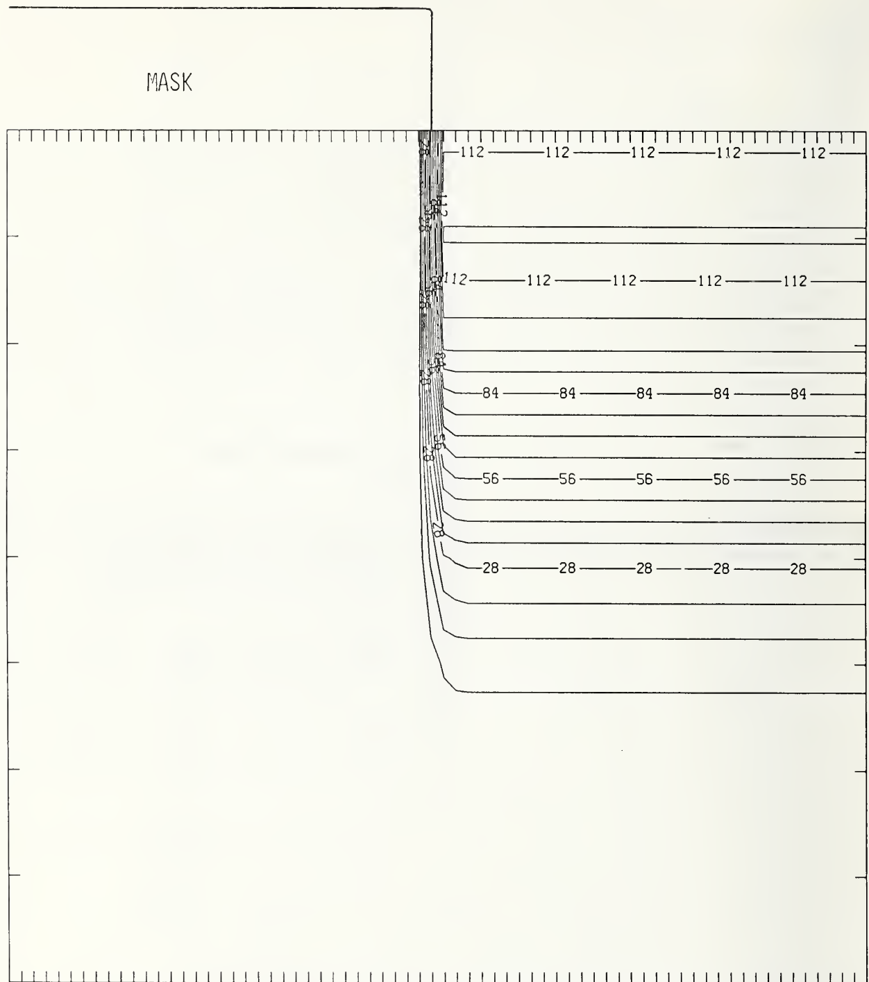
Figure Ge100-4 Two-dimensional distribution of Frenkel pairs created by 100 keV germanium implanted past a mask edge. The length increment (distance between tick marks) is 0.02 \mu\text{m} and the scale factor is 0.1.
