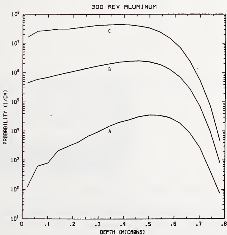
Figure A1300-2 One-dimensional probability distributions for implanted aluminum (A), primary silicon displacements (B), and Frenkel pairs (C) for 300 keV aluminum normally incident on a silicon target.
