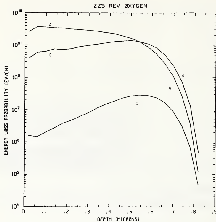
Figure O225-1 One-dimensional probability distributions for energy loss due to electronic excitation (A), displacement damage(B), and phonon excitation (C) for 225 keV oxygen normally incident on a silicon target.
