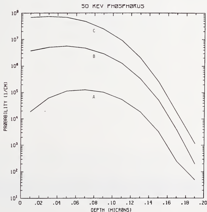
Figure P50-2 One-dimensional probability distributions for implanted phosphorus (A), primary silicon displacements (B), and Frenkel pairs (C) for 50 keV phosphorus normally incident on a silicon target.
