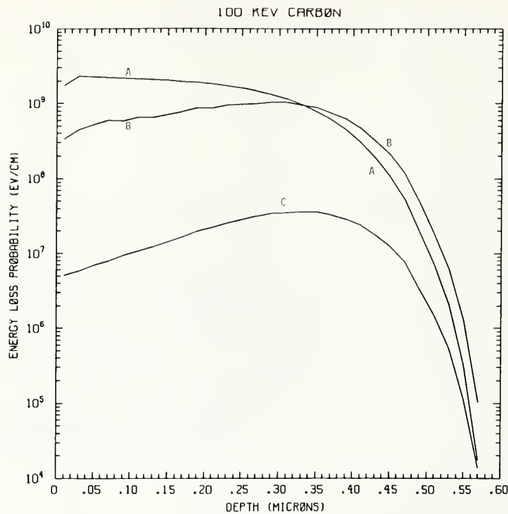
Figure C100-1 One-dimensional probability distributions for energy loss due to electronic excitation (A), displacement damage (B), and phonon excitation (C) for 100 keV carbon normally incident on a silicon target.
