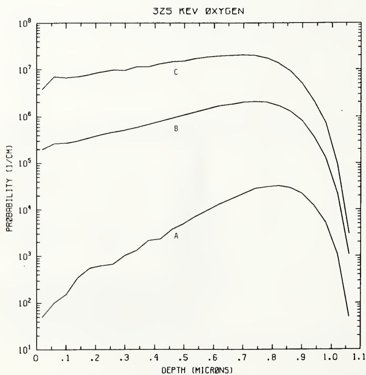
Figure O325-2 One-dimensional probability distributions for implanted oxygen (A), primary silicon displacements (B), and Frenkel pairs (C) for 325 keV oxygen normally incident on a silicon target.
