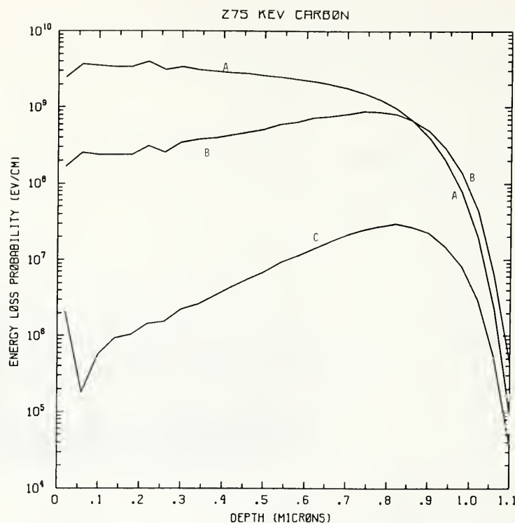
Figure C275-1 One-dimensional probability distributions for energy loss due to electronic excitation (A), displacement damage (B), and phonon excitation (C) for 275 keV carbon normally incident on a silicon target.
