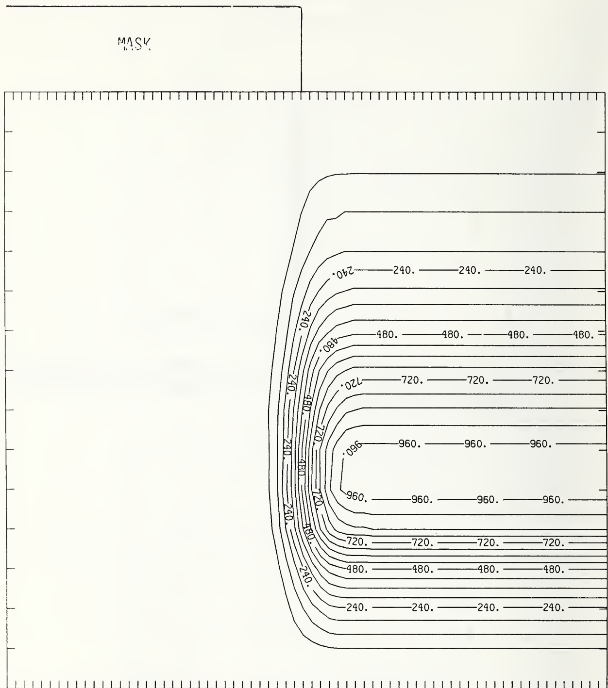
Figure Si250-3 Two-dimensional distribution of 250 keV silicon implanted past a mask edge. The length increment (distance between tick marks) is 0.04 \mu\text{m} and the scale factor is 1000.
