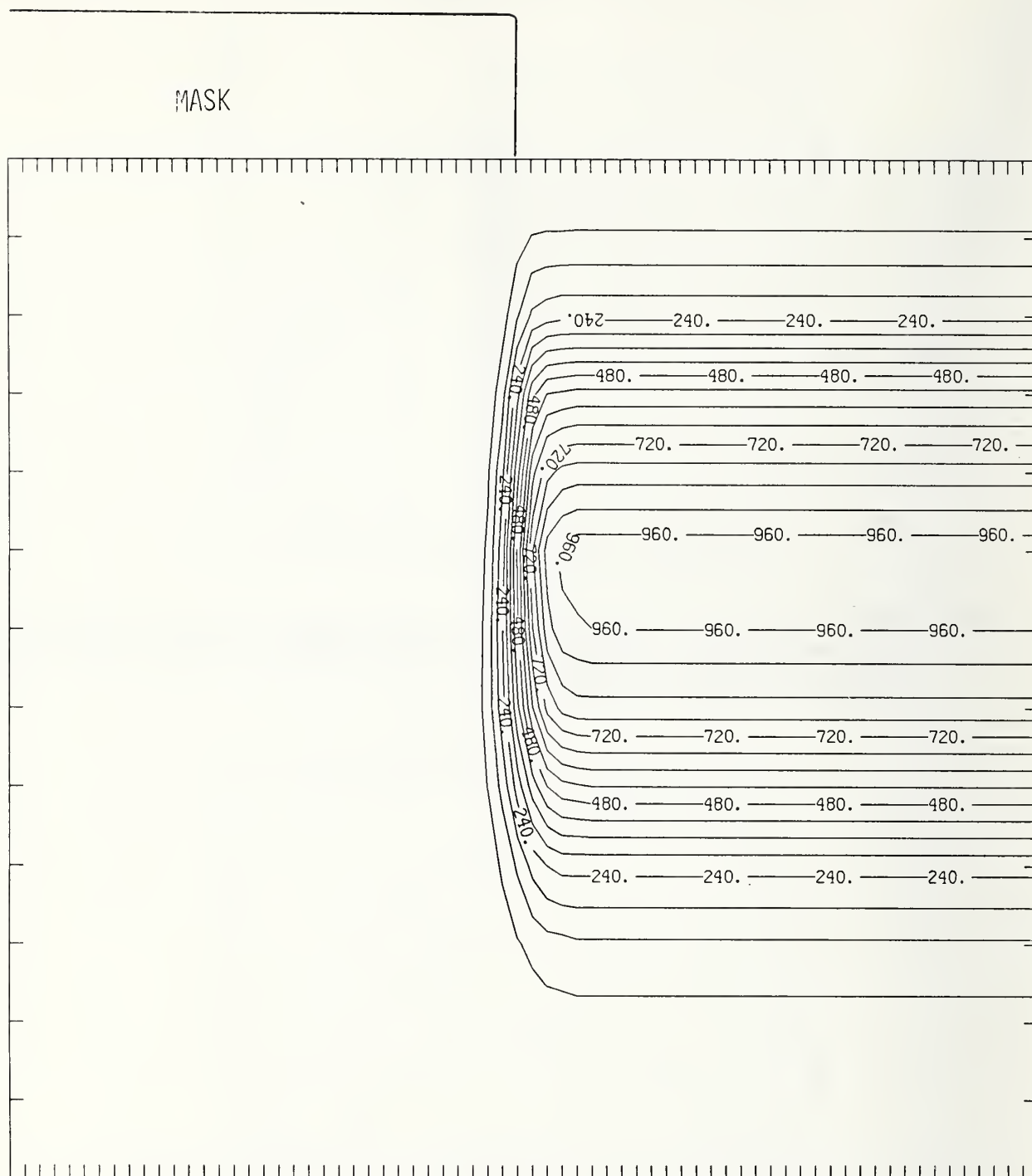
Figure Ge175-3 Two-dimensional distribution of 175 keV germanium implanted past a mask edge. The length increment (distance between tick marks) is 0.02 \mu\text{m} and the scale factor is 1000.
