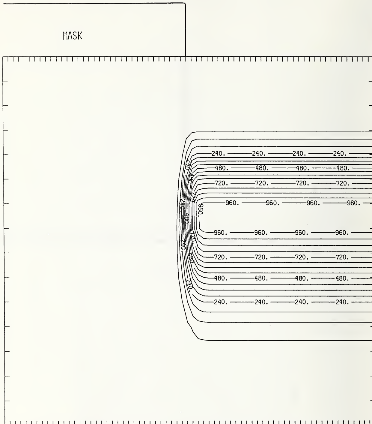
Figure Pt150-3 Two-dimensional distribution of 150 keV platinum implanted past a mask edge. The length increment (distance between tick marks) is 0.01 \mu\text{m} and the scale factor is 1000.
