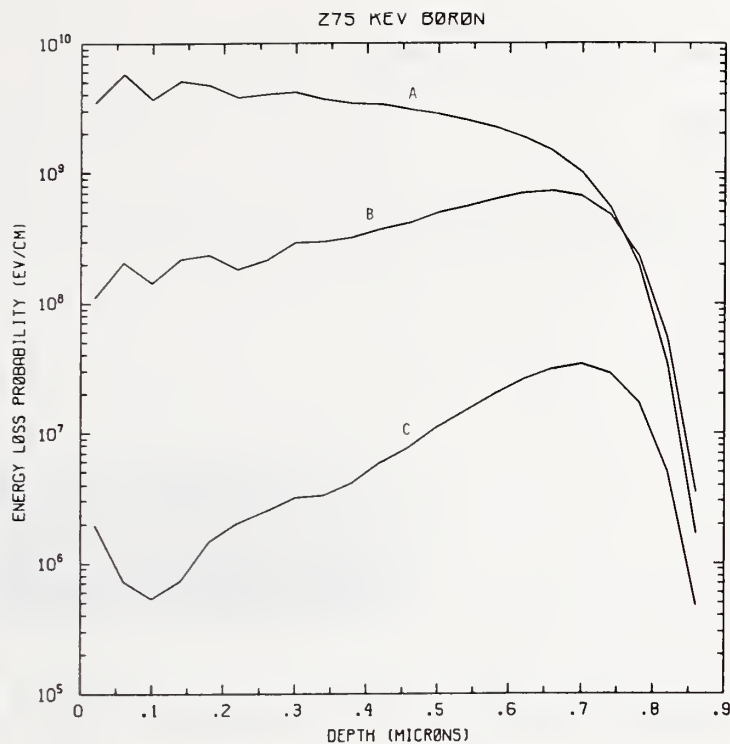
Figure B275-1 One-dimensional probability distributions for energy loss due to electronic excitation (A), displacement damage(B), and phonon excitation (C) for 275 keV boron normally incident on a silicon target.
