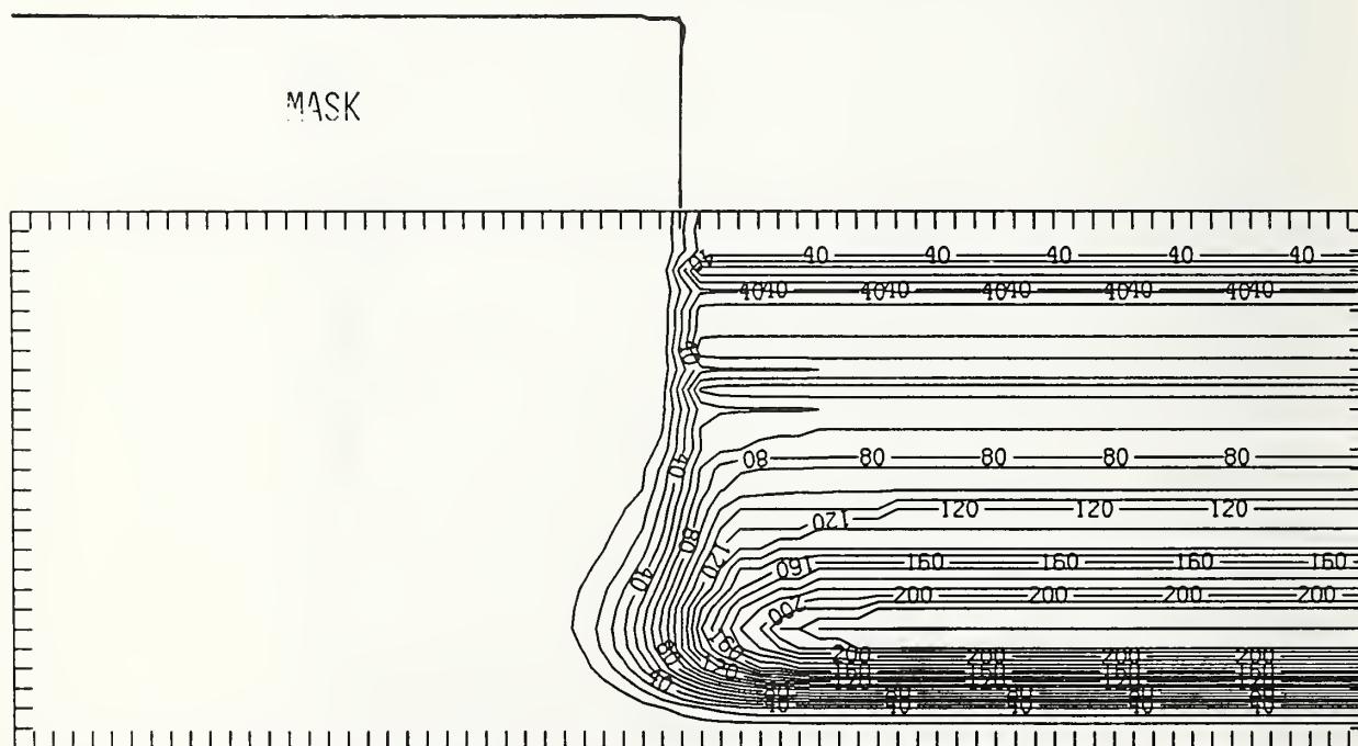
Figure B400-4 Two-dimensional distribution of Frenkel pairs created by 400 keV boron implanted past a mask edge. The length increment (distance between tick marks) is 0.04\ \mu\text{m} and the scale factor is 1.
