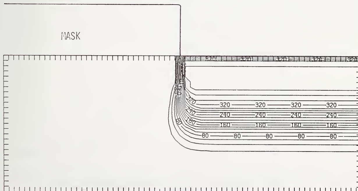
Figure Sb400-4 Two-dimensional distribution of Frenkel pairs created by 400 keV antimony implanted past a mask edge. The length increment (distance between tick marks) is 0.015 \mu\text{m} and the scale factor is 0.1.
