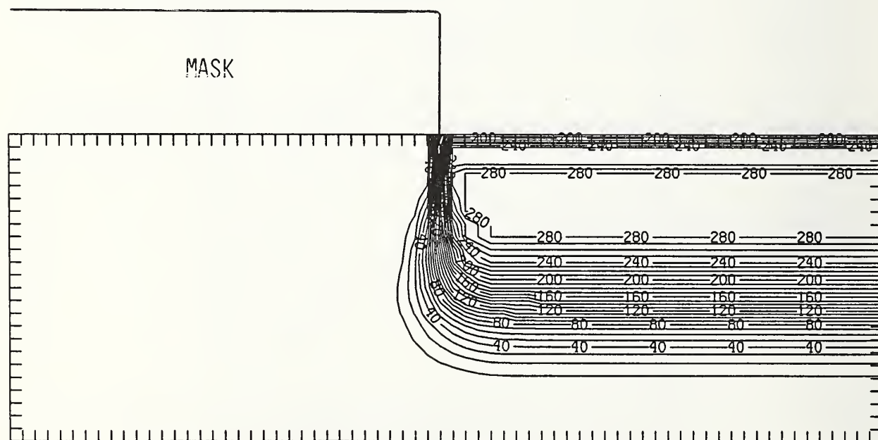
Figure Ga350-4 Two-dimensional distribution of Frenkel pairs created by 350 keV gallium implanted past a mask edge. The length increment (distance between tick marks) is 0.02 \mu\text{m} and the scale factor is 0.1.
