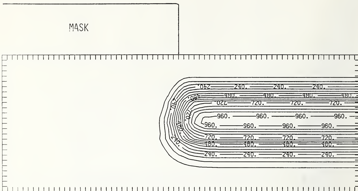
Figure Sn400-3 Two-dimensional distribution of 400 keV tin implanted past a mask edge. The length increment (distance between tick marks) is 0.015 \mu\text{m} and the scale factor is 1000.
