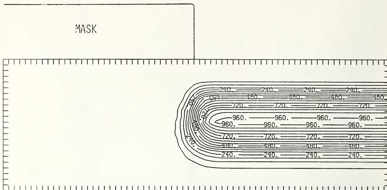
Figure Sn350-3 Two-dimensional distribution of 350 keV tin implanted past a mask edge. The length increment (distance between tick marks) is 0.015 \mu\text{m} and the scale factor is 1000.
