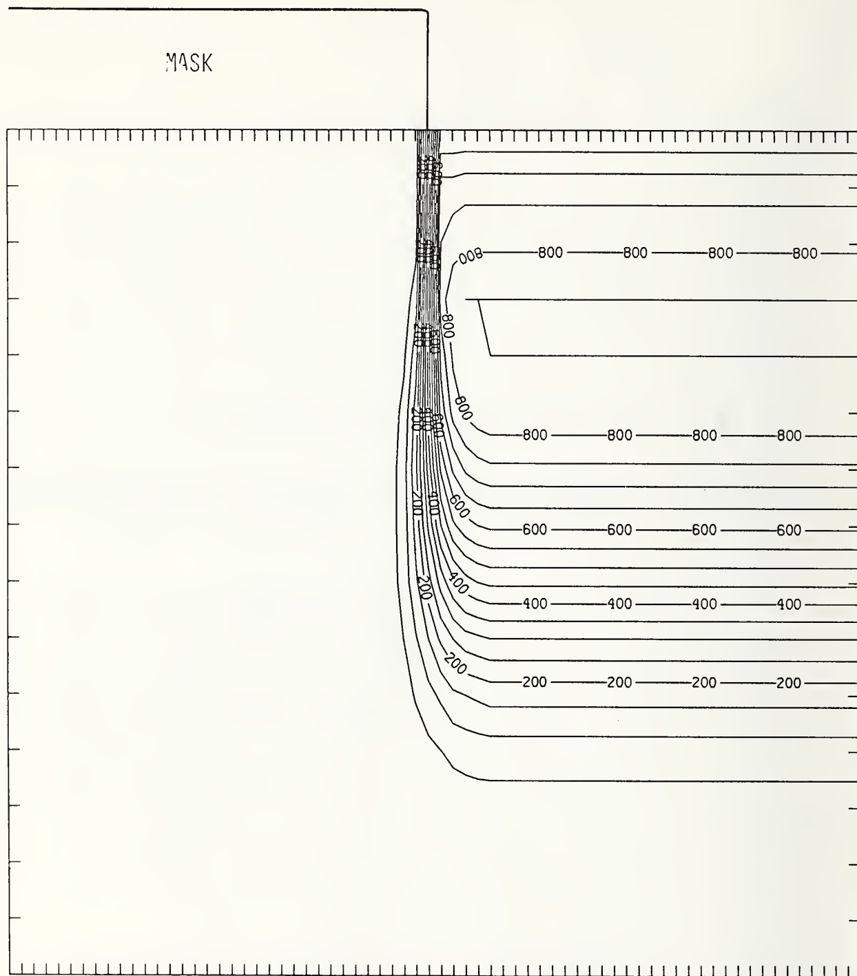
Figure Si100-4 Two-dimensional distribution of Frenkel pairs created by 100 keV silicon implanted past a mask edge. The length increment (distance between tick marks) is 0.02 \mu\text{m} and the scale factor is 1.
