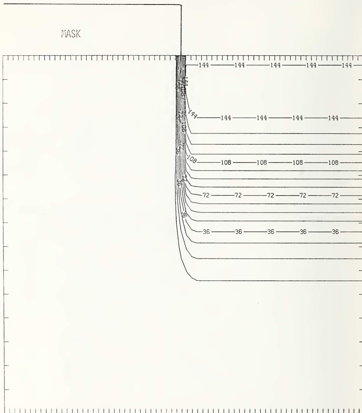
Figure Sb125-4 Two-dimensional distribution of Frenkel pairs created by 125 keV antimony implanted past a mask edge. The length increment (distance between tick marks) is 0.01 \mu\text{m} and the scale factor is 0.1.
