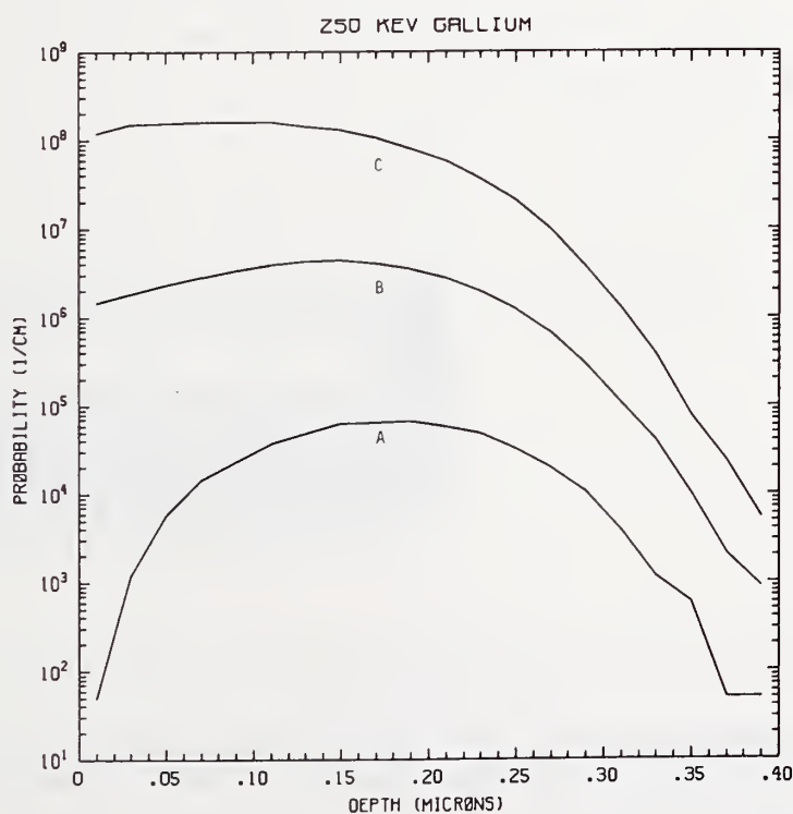
Figure Ga250-2 One-dimensional probability distributions for implanted gallium (A), primary silicon displacements (B), and Frenkel pairs (C) for 250 keV gallium normally incident on a silicon target.
