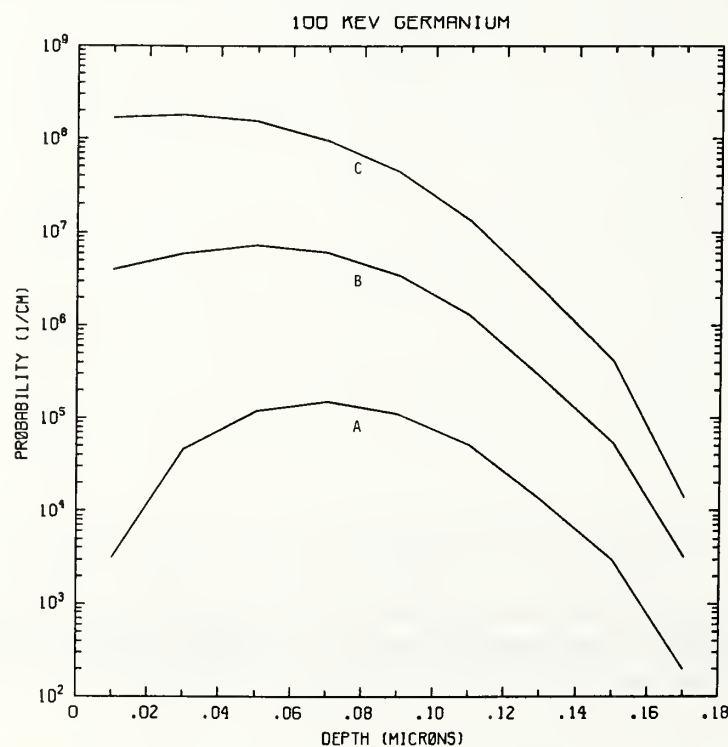
Figure Ge100-2 One-dimensional probability distributions for implanted germanium (A), primary silicon displacements (B), and Frenkel pairs (C) for 100 keV germanium normally incident on a silicon target.
