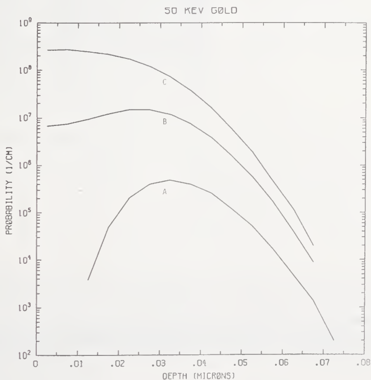
Figure Au50-2 One-dimensional probability distributions for implanted gold (A), primary silicon displacements (B), and Frenkel pairs (C) for 50 keV gold normally incident on a silicon target.
