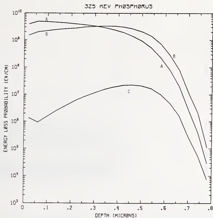
Figure P325-1 One-dimensional probability distributions for energy loss due to electronic excitation (A), displacement damage(B), and phonon excitation (C) for 325 keV phosphorus normally incident on a silicon target.
