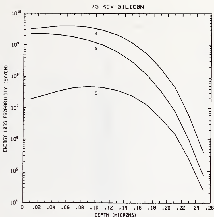
Figure Si75-1 One-dimensional probability distributions for energy loss due to electronic excitation (A), displacement damage (B), and phonon excitation (C) for 75 keV silicon normally incident on a silicon target.
