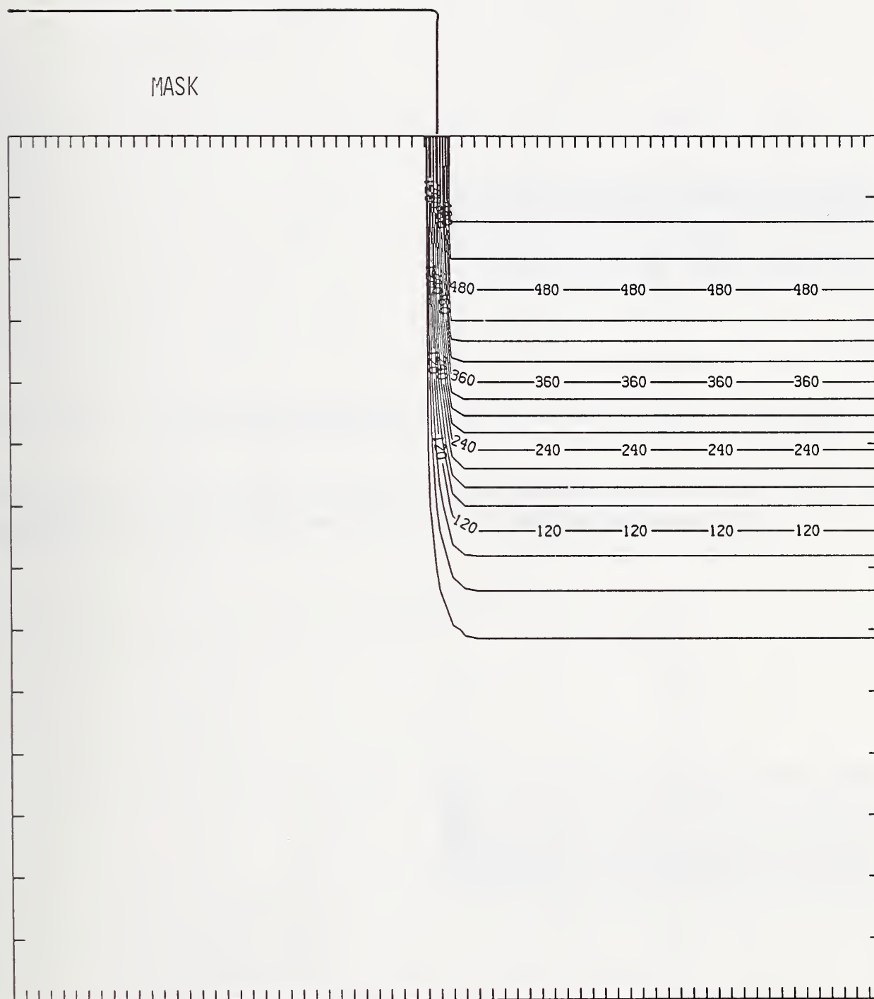
Figure Au50-4 Two-dimensional distribution of Frenkel pairs created by 50 keV gold implanted past a mask edge. The length increment (distance between tick marks) is 0.005 \mu\text{m} and the scale factor is 1.
