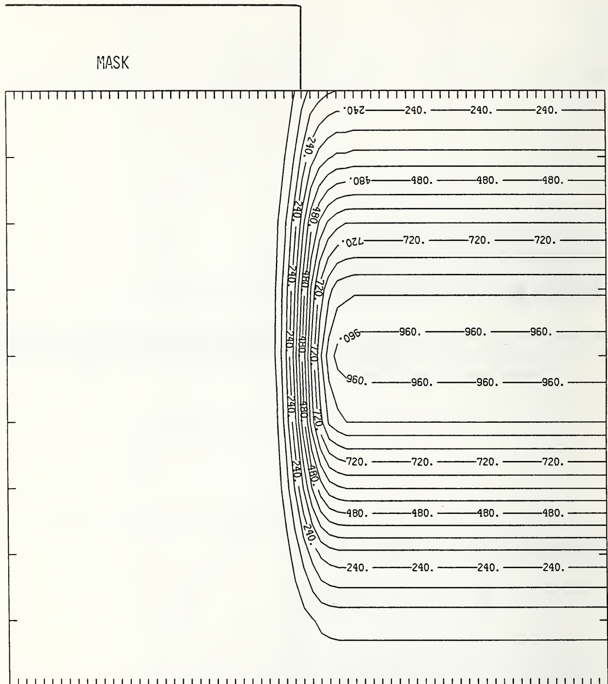
Figure C25-3 Two-dimensional distribution of 25 keV carbon implanted past a mask edge. The length increment (distance between tick marks) is 0.02 \mu\text{m} and the scale factor is 1000.
