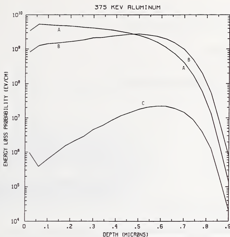
Figure Al375-1 One-dimensional probability distributions for energy loss due to electronic excitation (A), displacement damage(B), and phonon excitation (C) for 375 keV aluminum normally incident on a silicon target.
