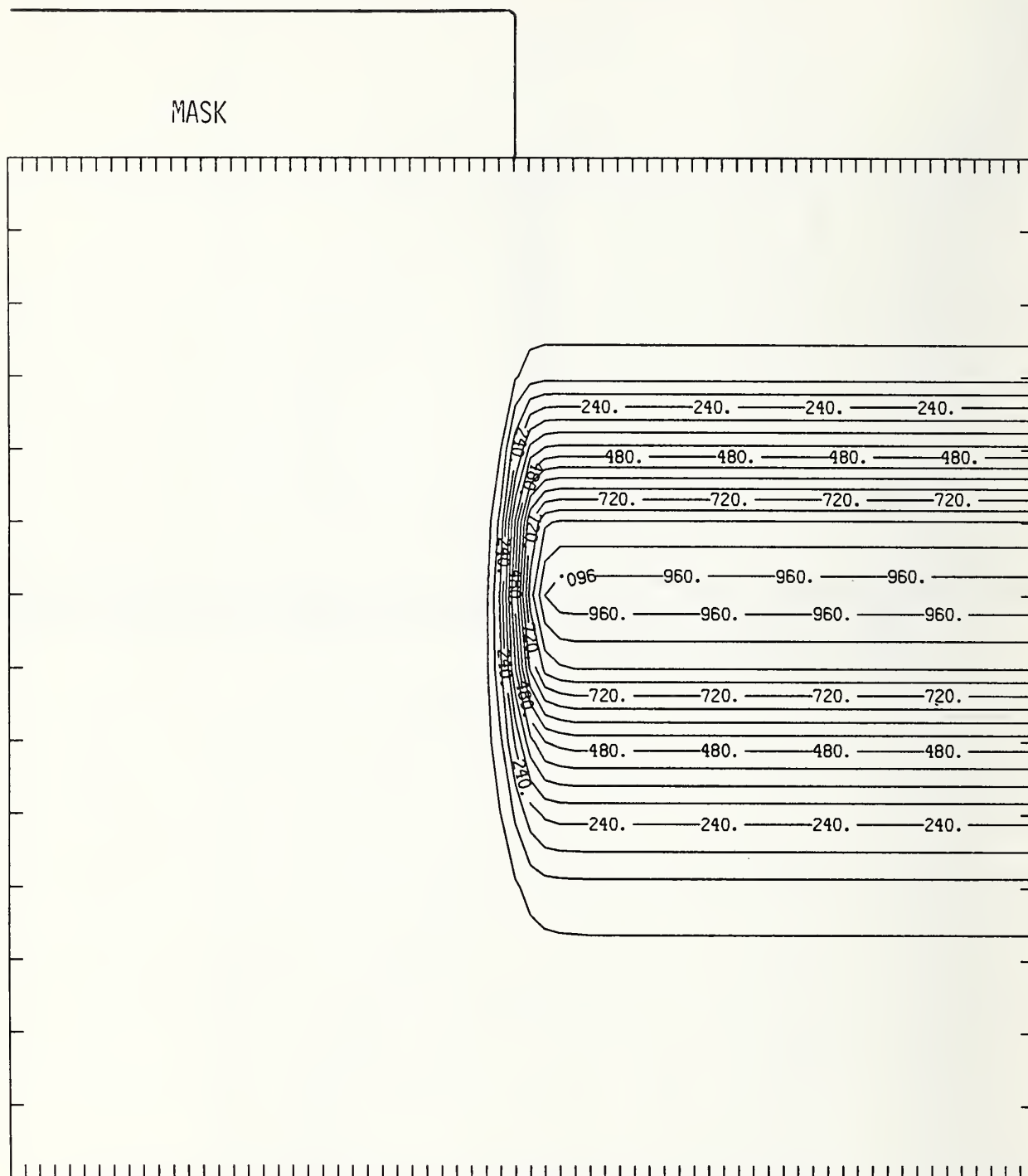
Figure Pt50-3 Two-dimensional distribution of 50 keV platinum implanted past a mask edge. The length increment (distance between tick marks) is 0.005 \mu\text{m} and the scale factor is 1000.
