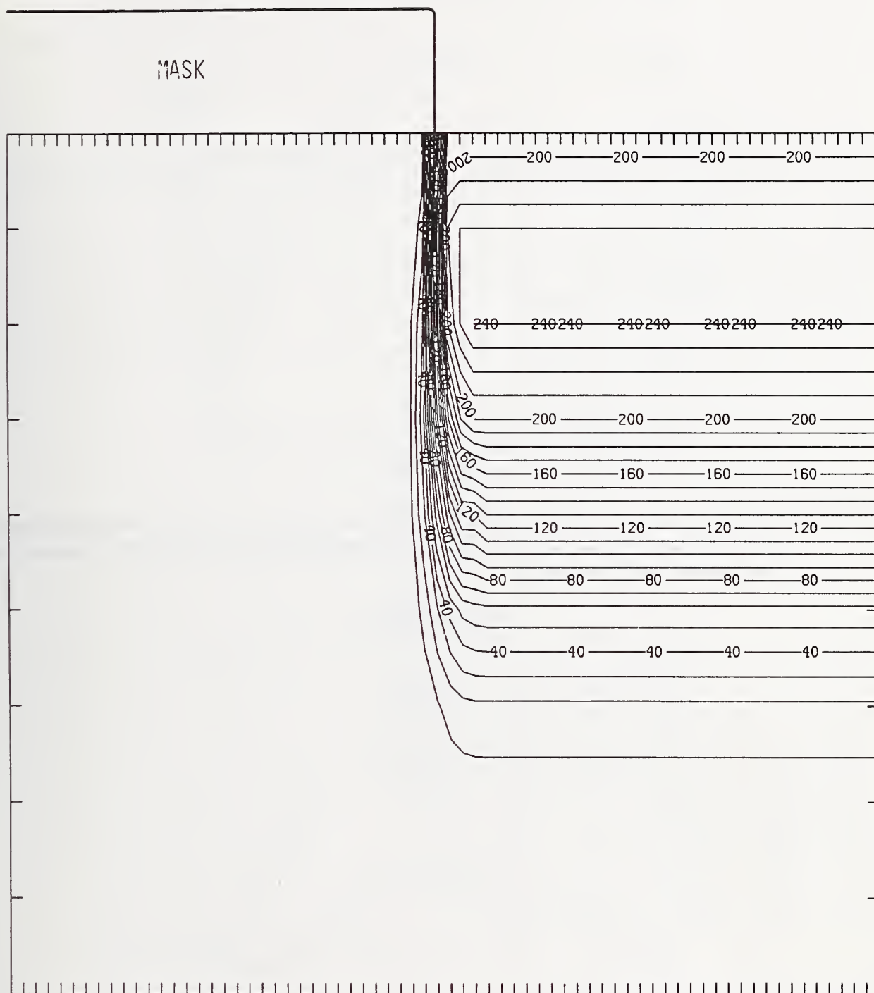
Figure N25-4 Two-dimensional distribution of Frenkel pairs created by 25 keV nitrogen implanted past a mask edge. The length increment (distance between tick marks) is 0.02 \mu\text{m} and the scale factor is 1.
