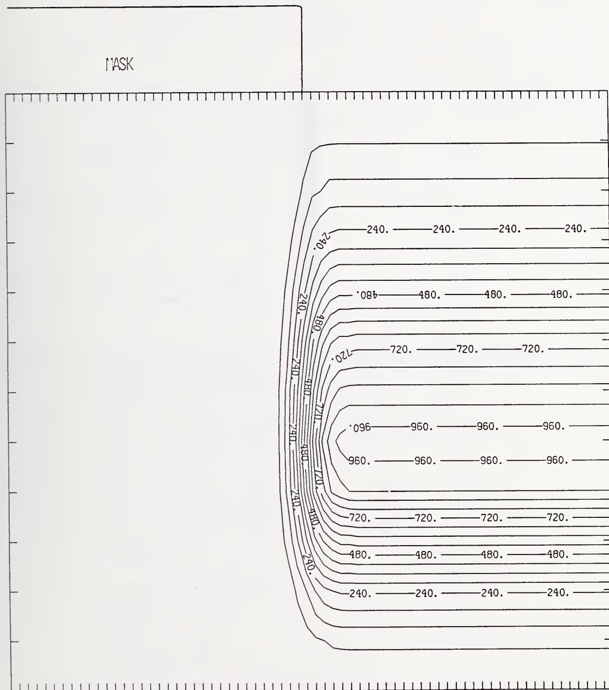
Figure P200-3 Two-dimensional distribution of 200 keV phosphorus implanted past a mask edge. The length increment (distance between tick marks) is 0.04 \mu\text{m} and the scale factor is 1000.
