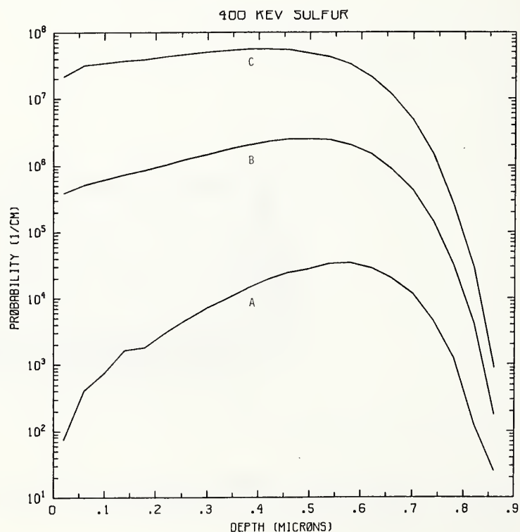
Figure S400-2 One-dimensional probability distributions for implanted sulfur (A), primary silicon displacements (B), and Frenkel pairs (C) for 400 keV sulfur normally incident on a silicon target.
