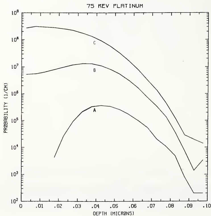
Figure Pt75-2 One-dimensional probability distributions for implanted platinum (A), primary silicon displacements (B), and Frenkel pairs (C) for 75 keV platinum normally incident on a silicon target.
