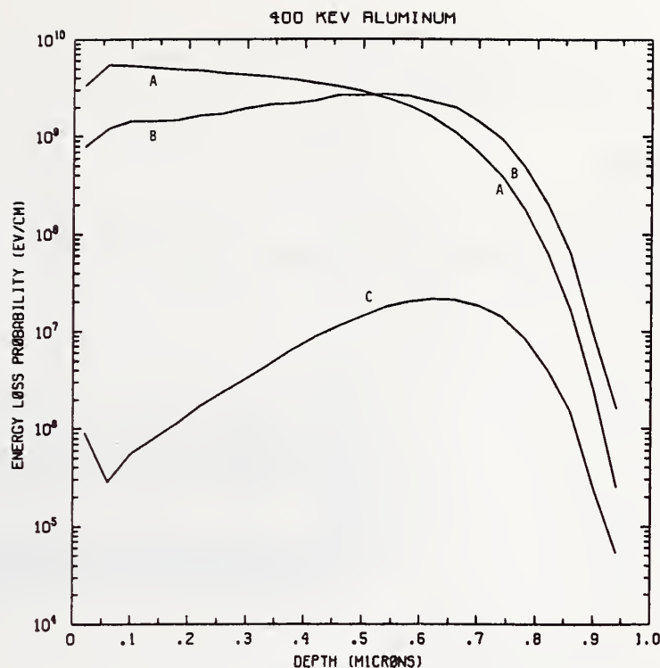
Figure Al400-1 One-dimensional probability distributions for energy loss due to electronic excitation (A), displacement damage (B), and phonon excitation (C) for 400 keV aluminum normally incident on a silicon target.
