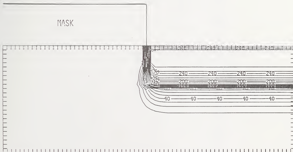
Figure Sn225-4 Two-dimensional distribution of Frenkel pairs created by 225 keV tin implanted past a mask edge. The length increment (distance between tick marks) is 0.01 \mu\text{m} and the scale factor is 0.1.
