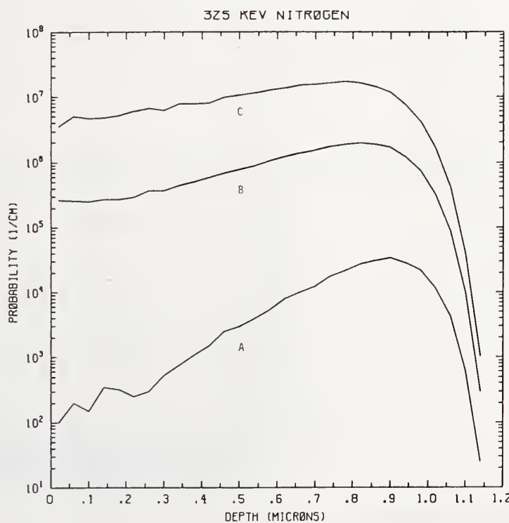
Figure N325-2 One-dimensional probability distributions for implanted nitrogen (A), primary silicon displacements (B), and Frenkel pairs (C) for 325 keV nitrogen normally incident on a silicon target.
