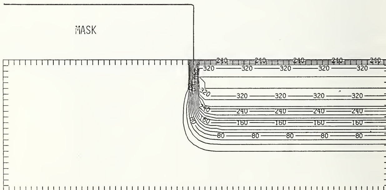
Figure Sn350-4 Two-dimensional distribution of Frenkel pairs created by 350 keV tin implanted past a mask edge. The length increment (distance between tick marks) is 0.015 \mu\text{m} and the scale factor is 0.1.
