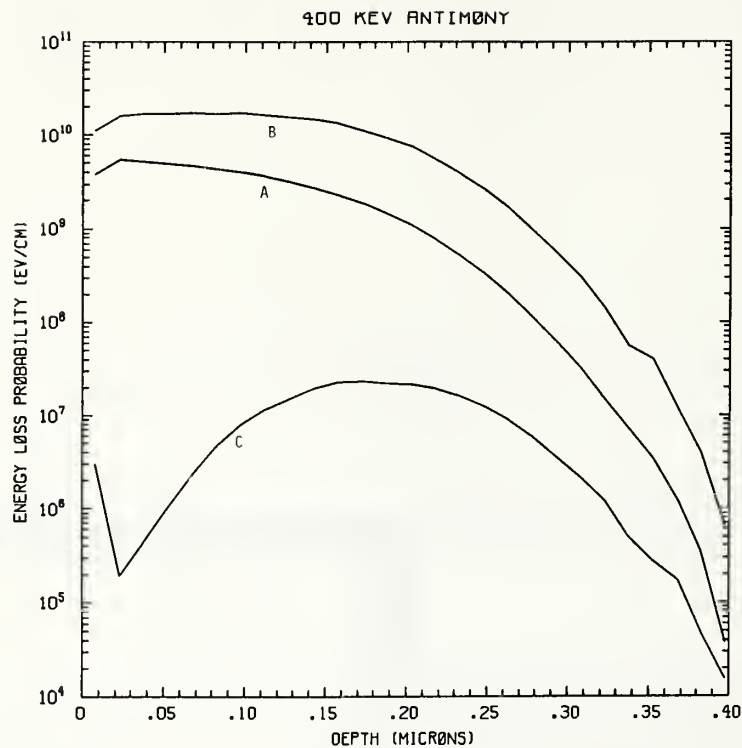
Figure Sb400-1 One-dimensional probability distributions for energy loss due to electronic excitation (A), displacement damage (B), and phonon excitation (C) for 400 keV antimony normally incident on a silicon target.
