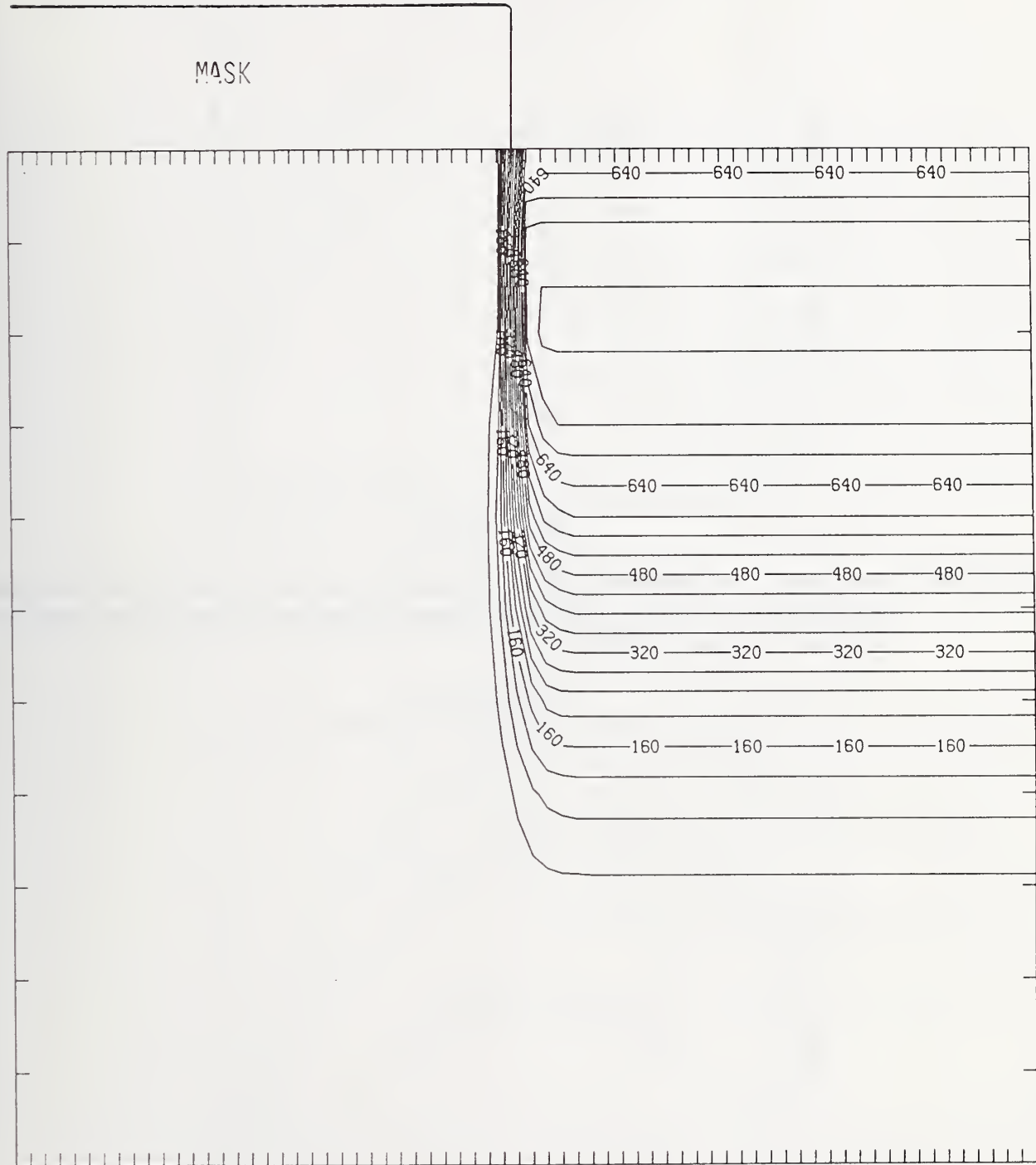
Figure S75-4 Two-dimensional distribution of Frenkel pairs created by 75 keV sulfur implanted past a mask edge. The length increment (distance between tick marks) is 0.02 \mu\text{m} and the scale factor is 1.
