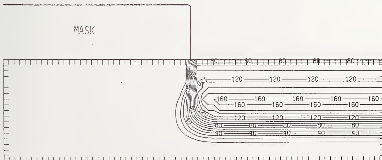
Figure S325-4 Two-dimensional distribution of Frenkel pairs created by 325 keV sulfur implanted past a mask edge. The length increment (distance between tick marks) is 0.04 \mu\text{m} and the scale factor is 0.1.
