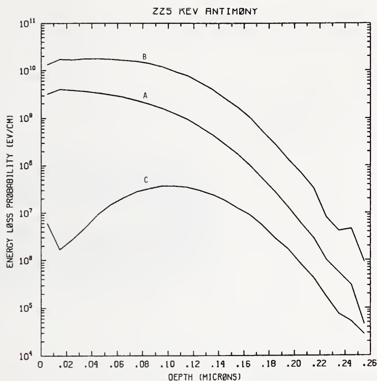
Figure Sb225-1 One-dimensional probability distributions for energy loss due to electronic excitation (A), displacement damage(B), and phonon excitation (C) for 225 keV antimony normally incident on a silicon target.
