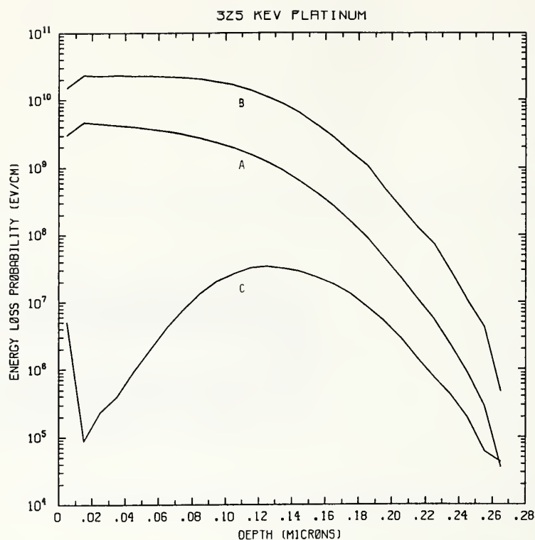
Figure Pt325-1 One-dimensional probability distributions for energy loss due to electronic excitation (A), displacement damage(B), and phonon excitation (C) for 325 keV platinum normally incident on a silicon target.
