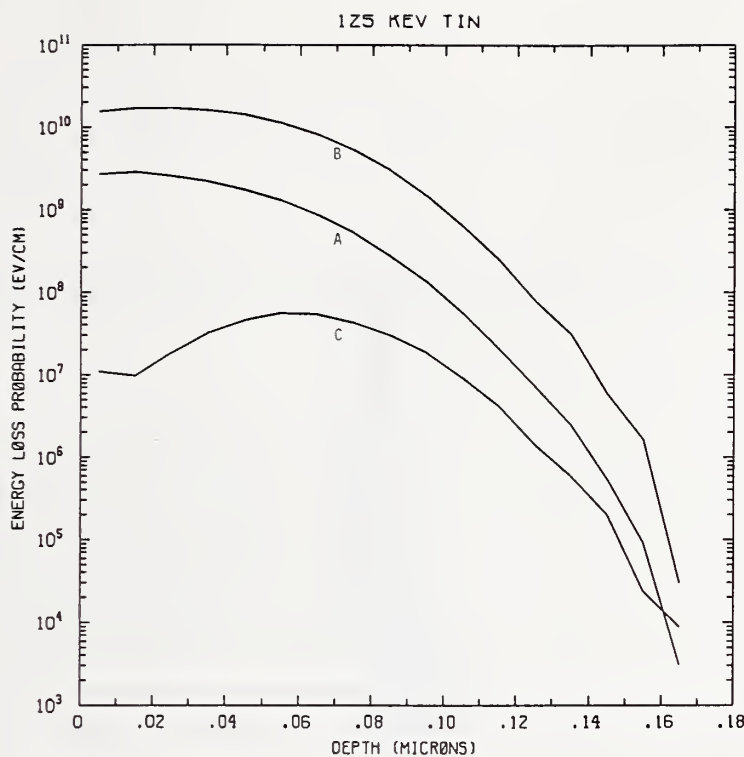
Figure Sn125-1 One-dimensional probability distributions for energy loss due to electronic excitation (A), displacement damage(B), and phonon excitation (C) for 125 keV tin normally incident on a silicon target.
