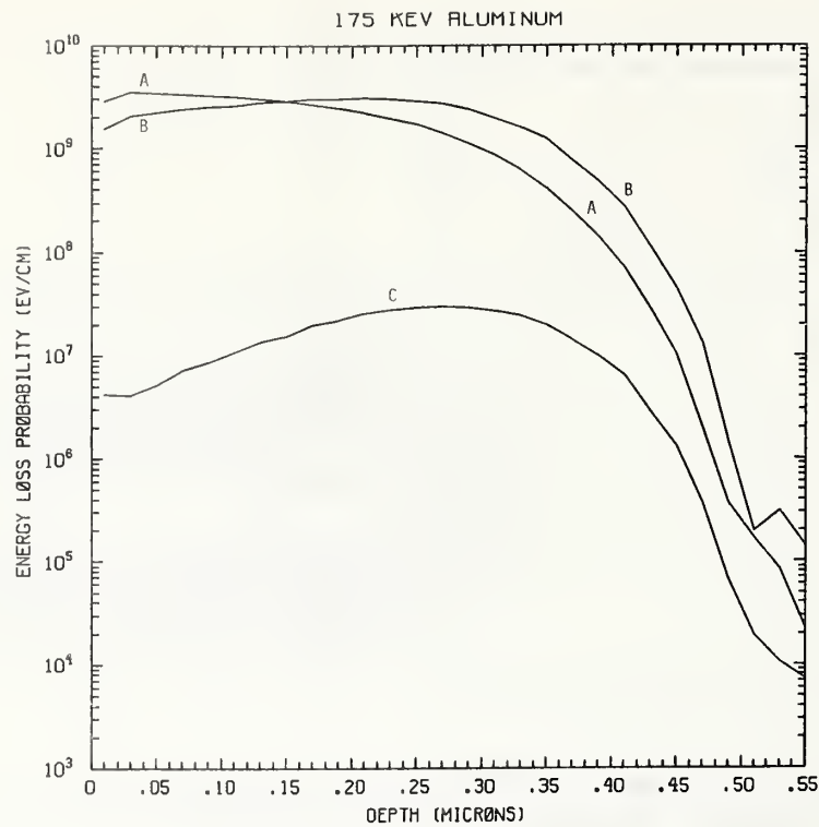
Figure Al175-1 One-dimensional probability distributions for energy loss due to electronic excitation (A), displacement damage (B), and phonon excitation (C) for 175 keV aluminum normally incident on a silicon target.
