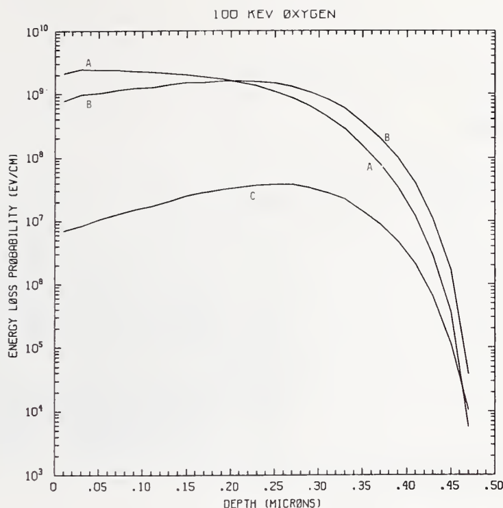
Figure O100-1 One-dimensional probability distributions for energy loss due to electronic excitation (A), displacement damage(B), and phonon excitation (C) for 100 keV oxygen normally incident on a silicon target.
