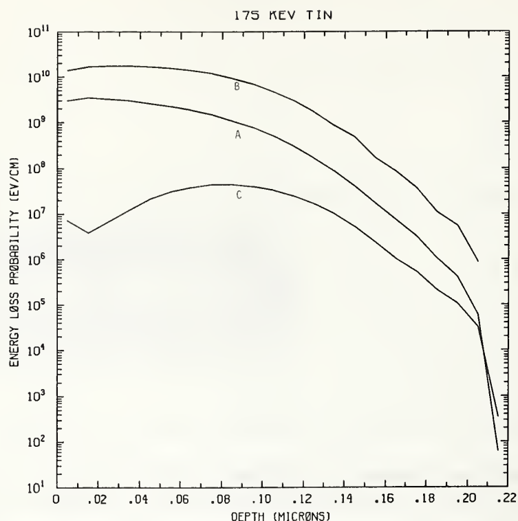
Figure Sn175-1 One-dimensional probability distributions for energy loss due to electronic excitation (A), displacement damage(B), and phonon excitation (C) for 175 keV tin normally incident on a silicon target.
