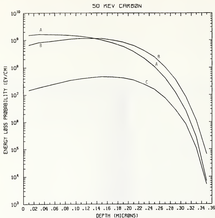
Figure C50-1 One-dimensional probability distributions for energy loss due to electronic excitation (A), displacement damage(B), and phonon excitation (C) for 50 keV carbon normally incident on a silicon target.
