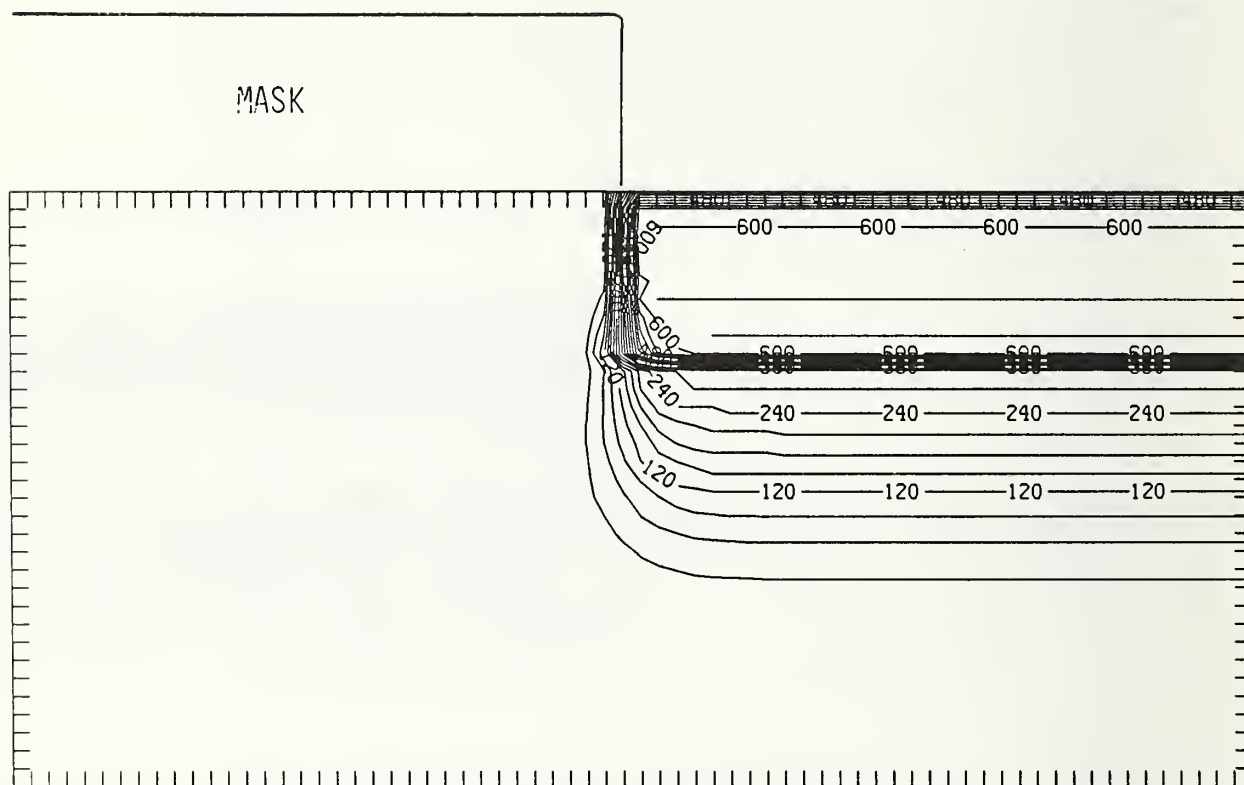
Figure Sn325-4 Two-dimensional distribution of Frenkel pairs created by 325 keV tin implanted past a mask edge. The length increment (distance between tick marks) is 0.01\ \mu\text{m} and the scale factor is 0.1.
