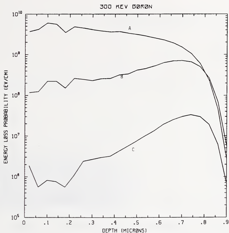
Figure B300-1 One-dimensional probability distributions for energy loss due to electronic excitation (A), displacement damage(B), and phonon excitation (C) for 300 keV boron normally incident on a silicon target.
