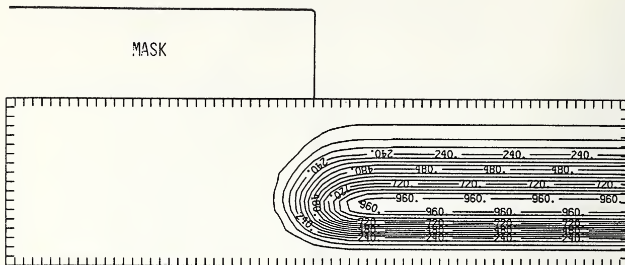
Figure Al275-3 Two-dimensional distribution of 275 keV aluminum implanted past a mask edge. The length increment (distance between tick marks) is 0.04 \mu\text{m} and the scale factor is 1000.
