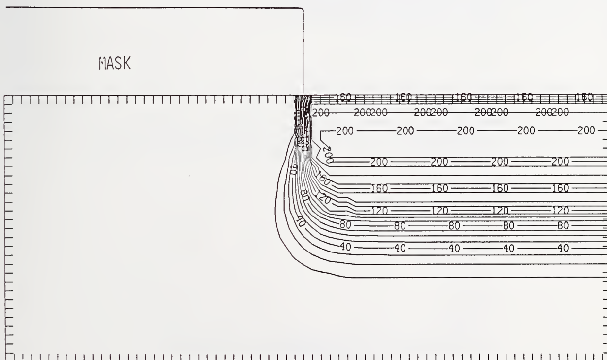
Figure As200-4 Two-dimensional distribution of Frenkel pairs created by 200 keV arsenic implanted past a mask edge. The length increment (distance between tick marks) is 0.01 \mu\text{m} and the scale factor is 0.1.
