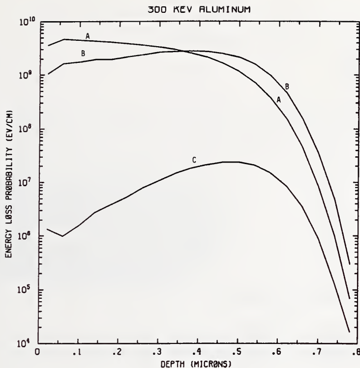
Figure A1300-1 One-dimensional probability distributions for energy loss due to electronic excitation (A), displacement damage (B), and phonon excitation (C) for 300 keV aluminum normally incident on a silicon target.
