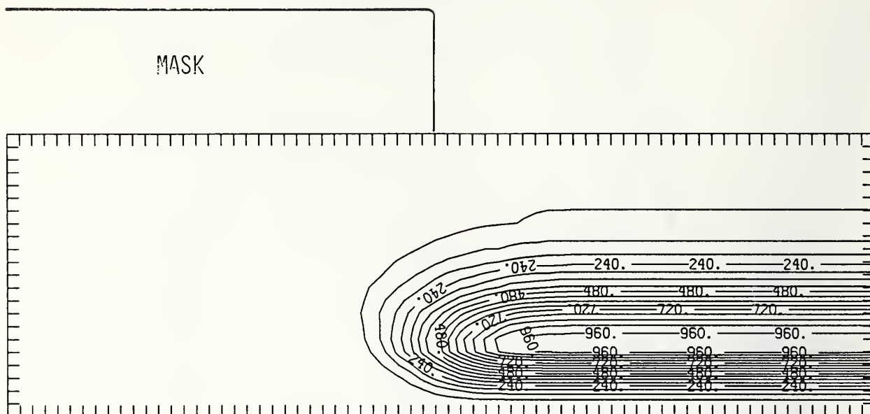
Figure N225-3 Two-dimensional distribution of 225 keV nitrogen implanted past a mask edge. The length increment (distance between tick marks) is 0.04 \mu\text{m} and the scale factor is 1000.
