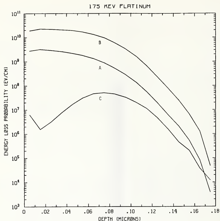
Figure Pt175-1 One-dimensional probability distributions for energy loss due to electronic excitation (A), displacement damage(B), and phonon excitation (C) for 175 keV platinum normally incident on a silicon target.
