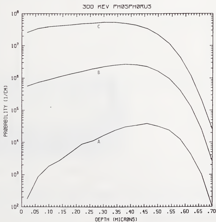
Figure P300-2 One-dimensional probability distributions for implanted phosphorus (A), primary silicon displacements (B), and Frenkel pairs (C) for 300 keV phosphorus normally incident on a silicon target.
