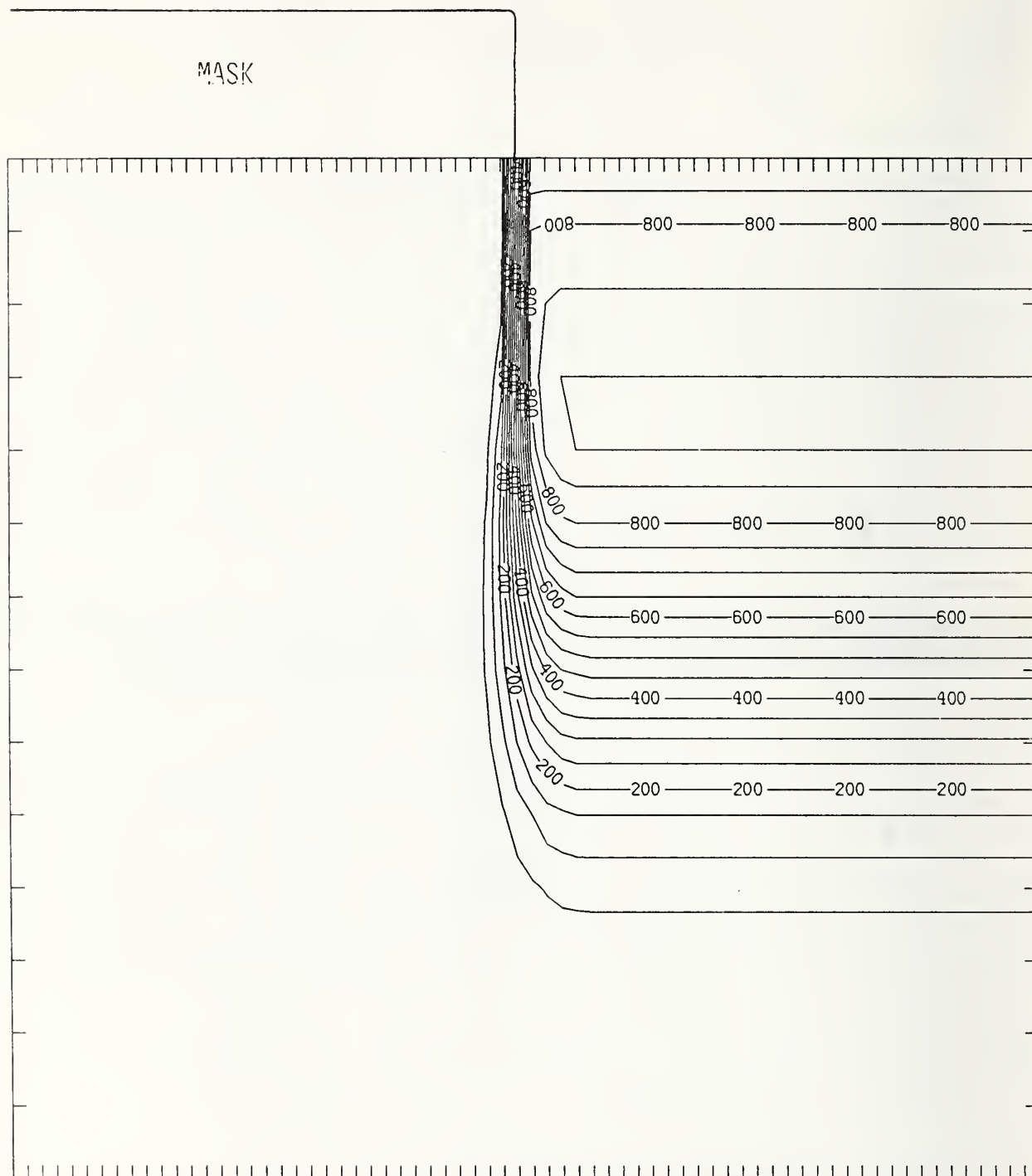
Figure S100-4 Two-dimensional distribution of Frenkel pairs created by 100 keV sulfur implanted past a mask edge. The length increment (distance between tick marks) is 0.02 \mu\text{m} and the scale factor is 1.
