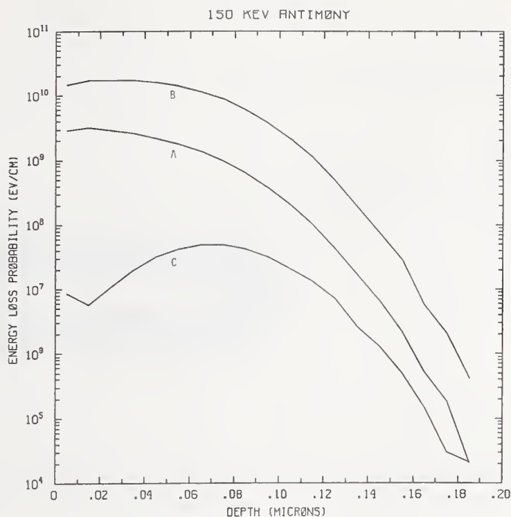
Figure Sb150-1 One-dimensional probability distributions for energy loss due to electronic excitation (A), displacement damage(B), and phonon excitation (C) for 150 keV antimony normally incident on a silicon target.
