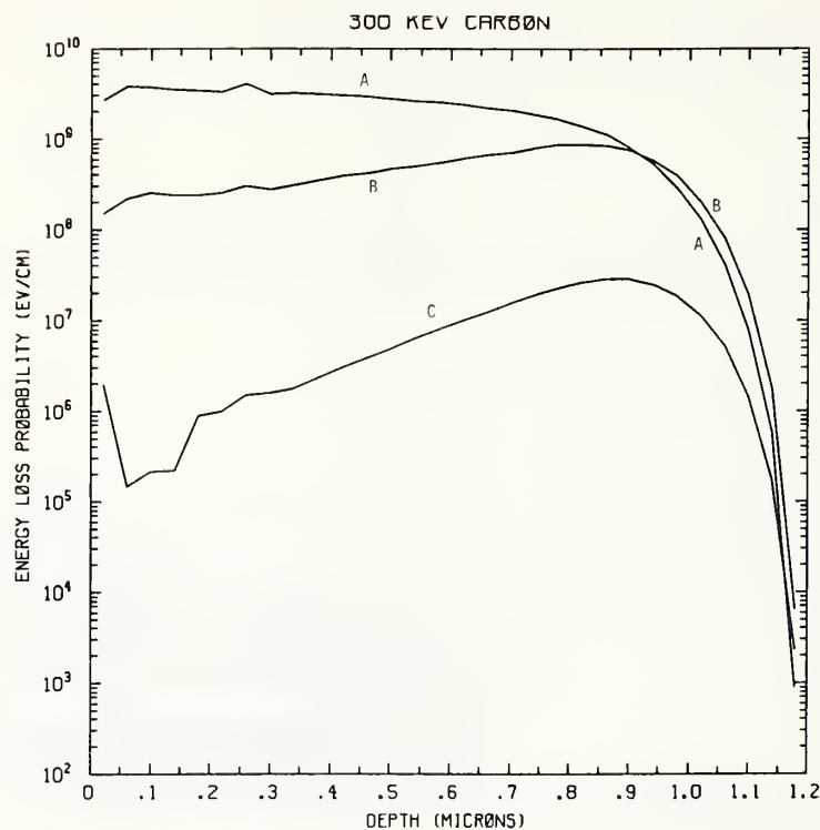
Figure C300-1 One-dimensional probability distributions for energy loss due to electronic excitation (A), displacement damage(B), and phonon excitation (C) for 300 keV carbon normally incident on a silicon target.
