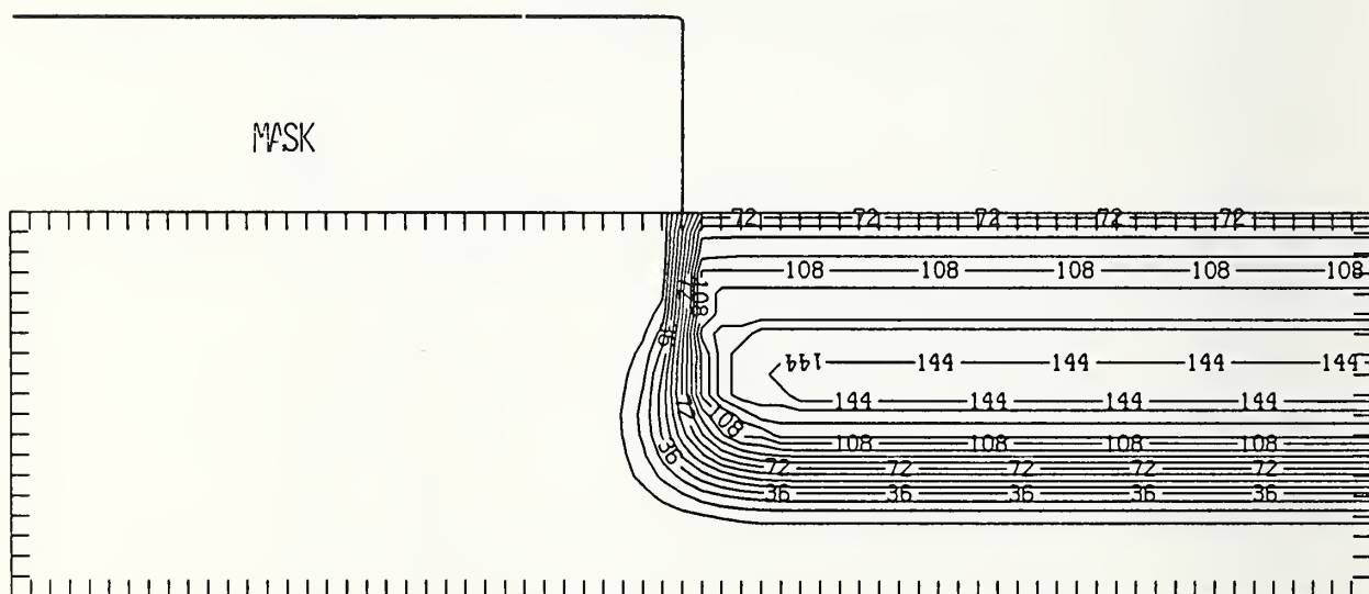
Figure P325-4 Two-dimensional distribution of Frenkel pairs created by 325 keV phosphorus implanted past a mask edge. The length increment (distance between tick marks) is 0.04 \mu\text{m} and the scale factor is 0.1.
