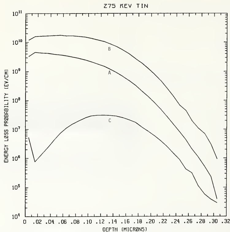
Figure Sn275-1 One-dimensional probability distributions for energy loss due to electronic excitation (A), displacement damage (B), and phonon excitation (C) for 275 keV tin normally incident on a silicon target.
