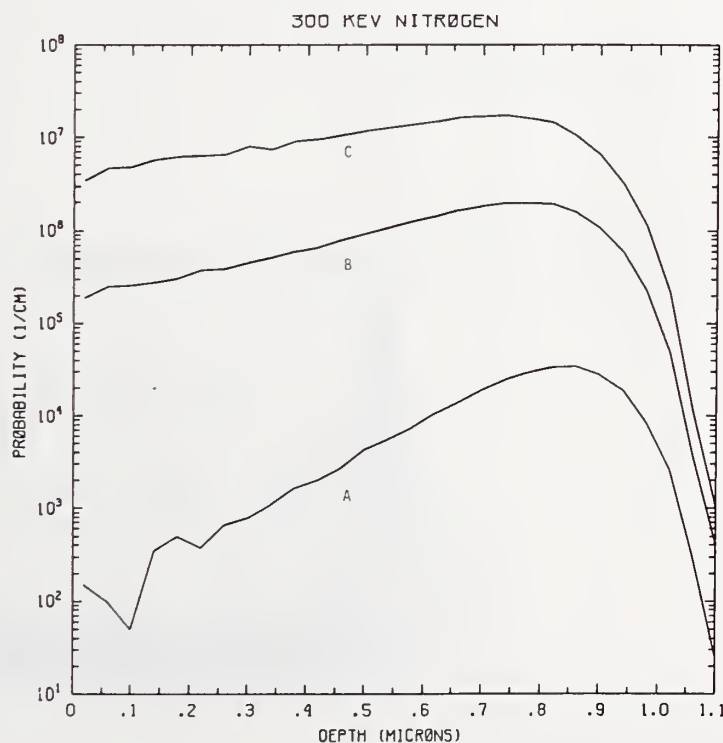
Figure N300-2 One-dimensional probability distributions for implanted nitrogen (A), primary silicon displacements (B), and Frenkel pairs (C) for 300 keV nitrogen normally incident on a silicon target.
