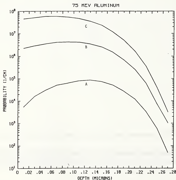
Figure Al75-2 One-dimensional probability distributions for implanted aluminum (A), primary silicon displacements (B), and Frenkel pairs (C) for 75 keV aluminum normally incident on a silicon target.
