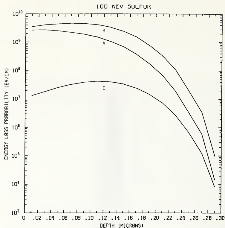
Figure S100-1 One-dimensional probability distributions for energy loss due to electronic excitation (A), displacement damage (B), and phonon excitation (C) for 100 keV sulfur normally incident on a silicon target.
