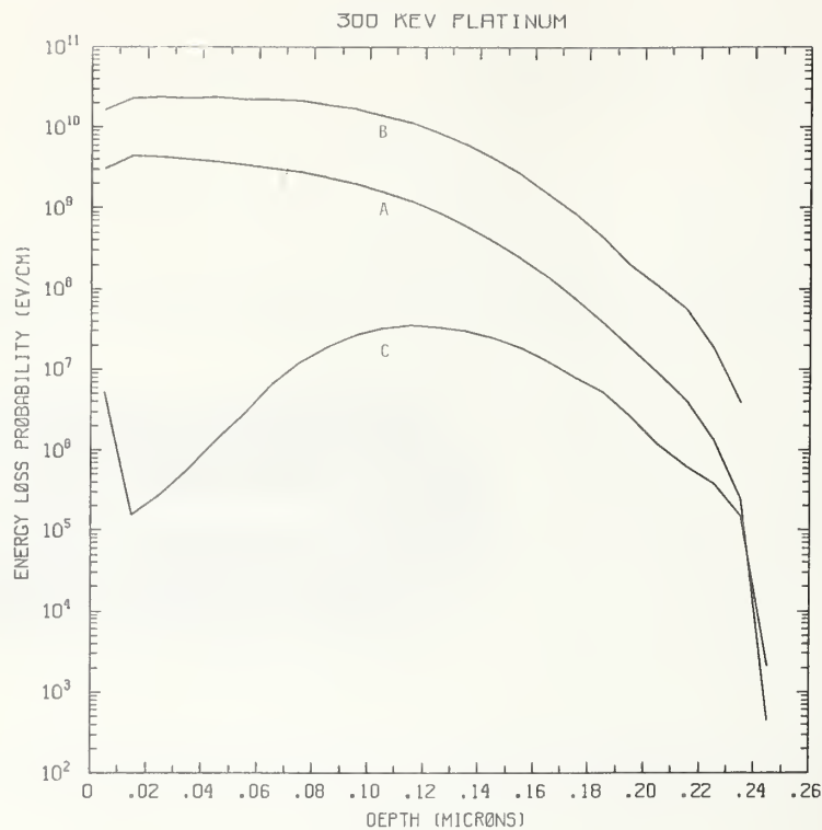
Figure Pt300-1 One-dimensional probability distributions for energy loss due to electronic excitation (A), displacement damage(B), and phonon excitation (C) for 300 keV platinum normally incident on a silicon target.
