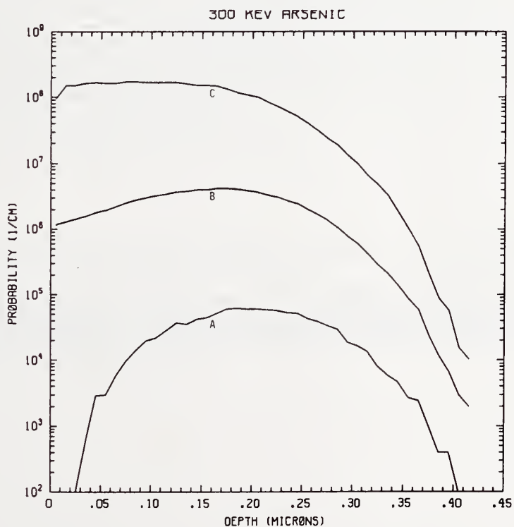
Figure As300-2 One-dimensional probability distributions for implanted arsenic (A), primary silicon displacements (B), and Frenkel pairs (C) for 300 keV arsenic normally incident on a silicon target.
