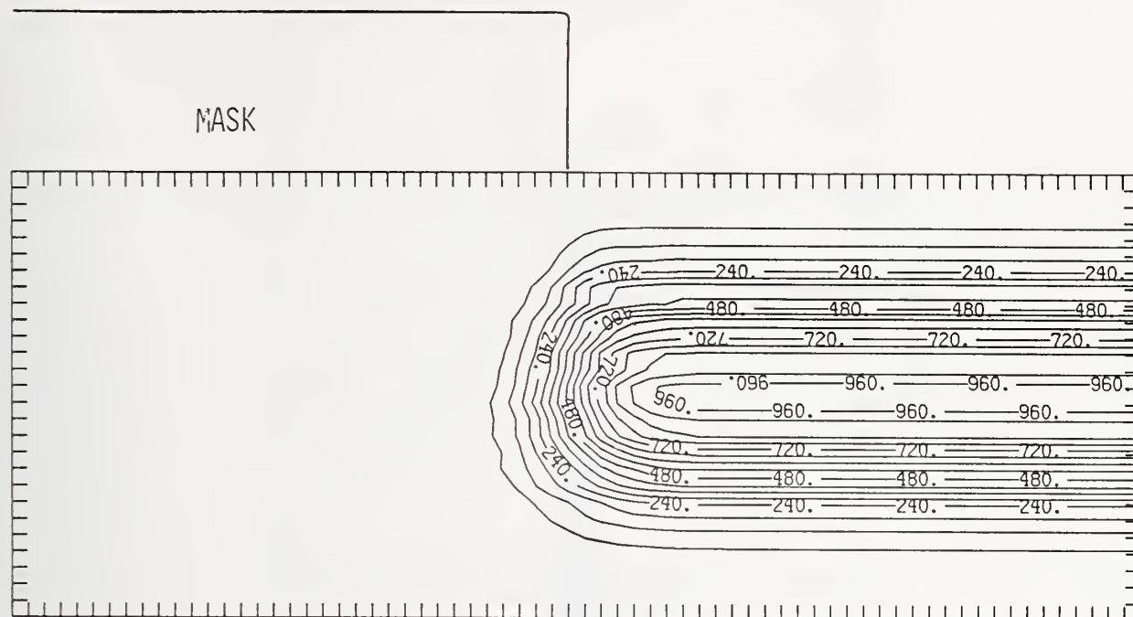
Figure Ge400-3 Two-dimensional distribution of 400 keV germanium implanted past a mask edge. The length increment (distance between tick marks) is 0.02\text{ }\mu\text{m} and the scale factor is 1000.
