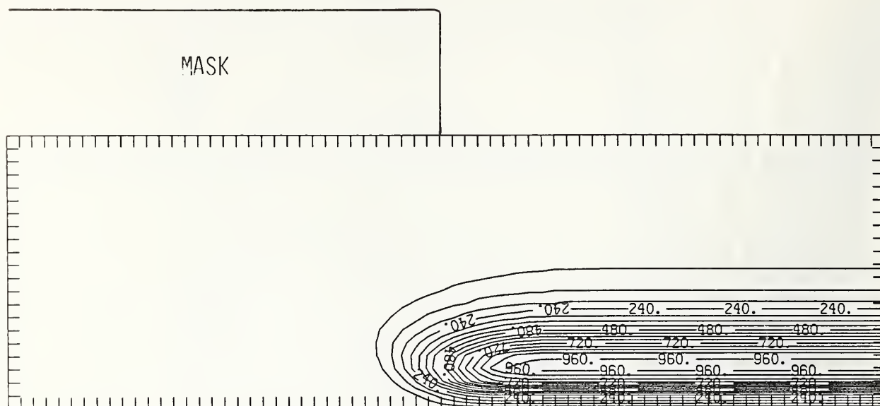
Figure B275-3 Two-dimensional distribution of 275 keV boron implanted past a mask edge. The length increment (distance between tick marks) is 0.04 \mu\text{m} and the scale factor is 1000.
