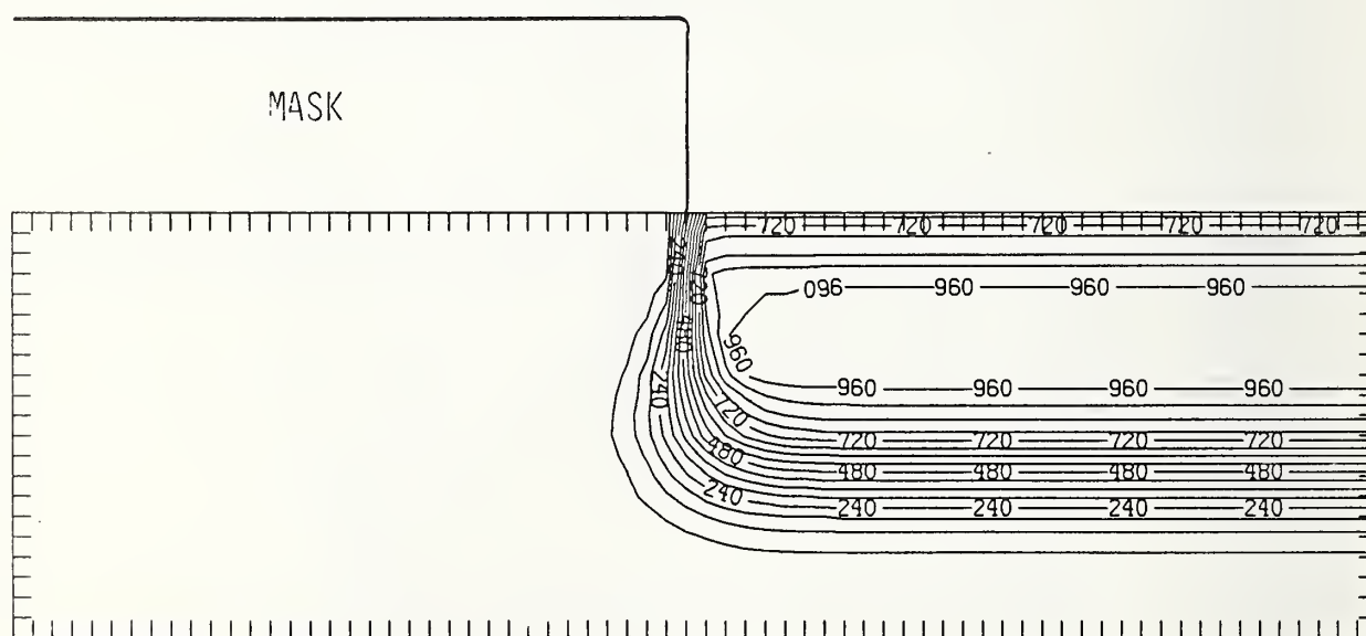
Figure Si150-4 Two-dimensional distribution of Frenkel pairs created by 150 keV silicon implanted past a mask edge. The length increment (distance between tick marks) is 0.02 \mu\text{m} and the scale factor is 1.
