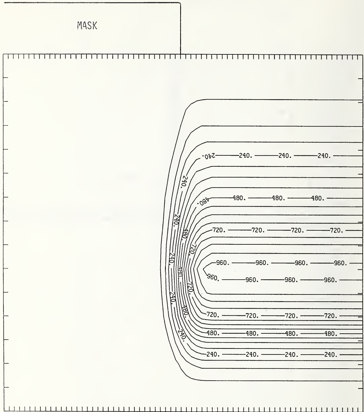
Figure Al225-3 Two-dimensional distribution of 225 keV aluminum implanted past a mask edge. The length increment (distance between tick marks) is 0.04 \mu\text{m} and the scale factor is 1000.
