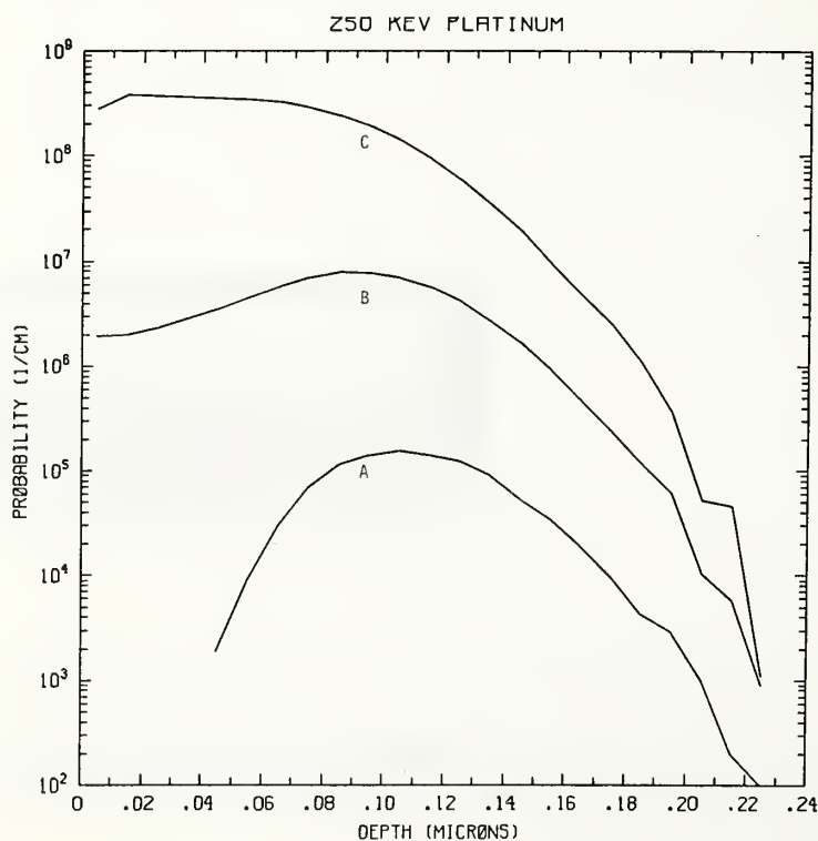
Figure Pt250-2 One-dimensional probability distributions for implanted platinum (A), primary silicon displacements (B), and Frenkel pairs (C) for 250 keV platinum normally incident on a silicon target.
