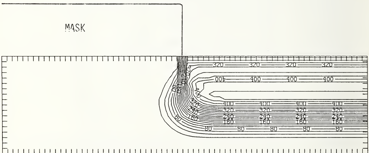
Figure O75-4 Two-dimensional distribution of Frenkel pairs created by 75 keV oxygen implanted past a mask edge. The length increment (distance between tick marks) is 0.02 \mu\text{m} and the scale factor is 1.
