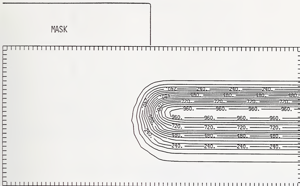
Figure Au175-3 Two-dimensional distribution of 175 keV gold implanted past a mask edge. The length increment (distance between tick marks) is 0.005 \mu\text{m} and the scale factor is 1000.
