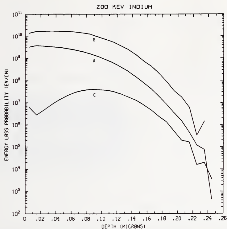
Figure In200-1 One-dimensional probability distributions for energy loss due to electronic excitation (A), displacement damage (B), and phonon excitation (C) for 200 keV indium normally incident on a silicon target.
