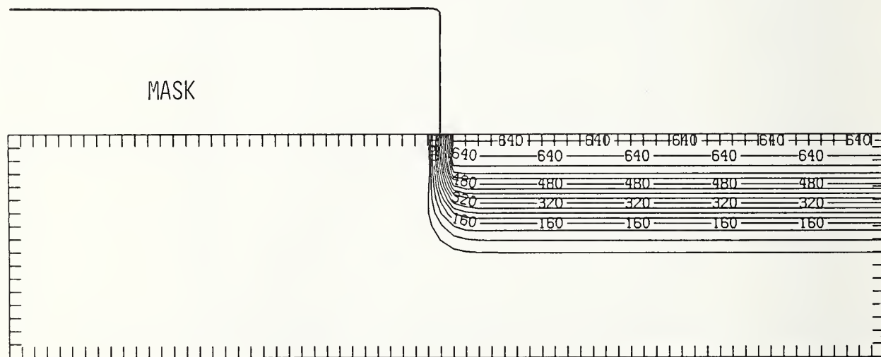
Figure In50-4 Two-dimensional distribution of Frenkel pairs created by 50 keV indium implanted past a mask edge. The length increment (distance between tick marks) is 0.005\ \mu\text{m} and the scale factor is 1.
