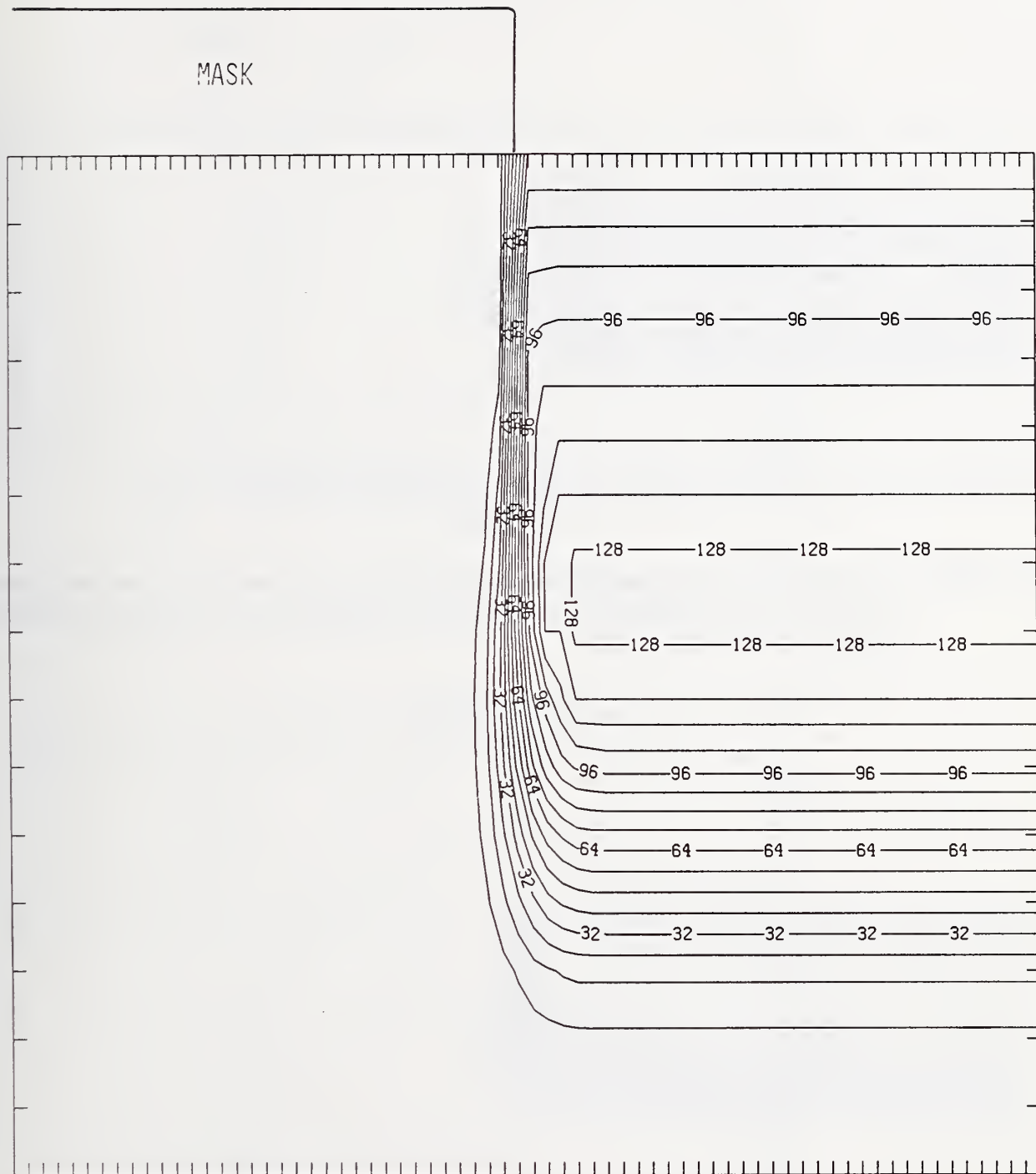
Figure Si250-4 Two-dimensional distribution of Frenkel pairs created by 250 keV silicon implanted past a mask edge. The length increment (distance between tick marks) is 0.04 \mu\text{m} and the scale factor is 0.1.
