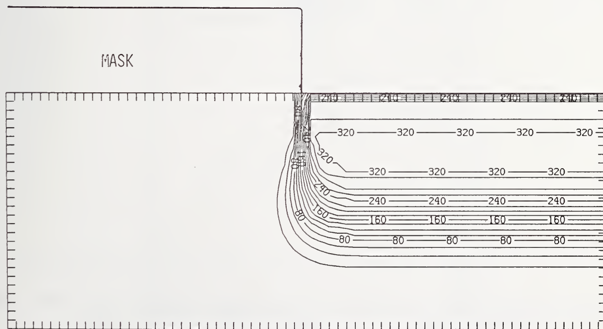
Figure Ge400-4 Two-dimensional distribution of Frenkel pairs created by 400 keV germanium implanted past a mask edge. The length increment (distance between tick marks) is 0.02\ \mu\text{m} and the scale factor is 0.1.
