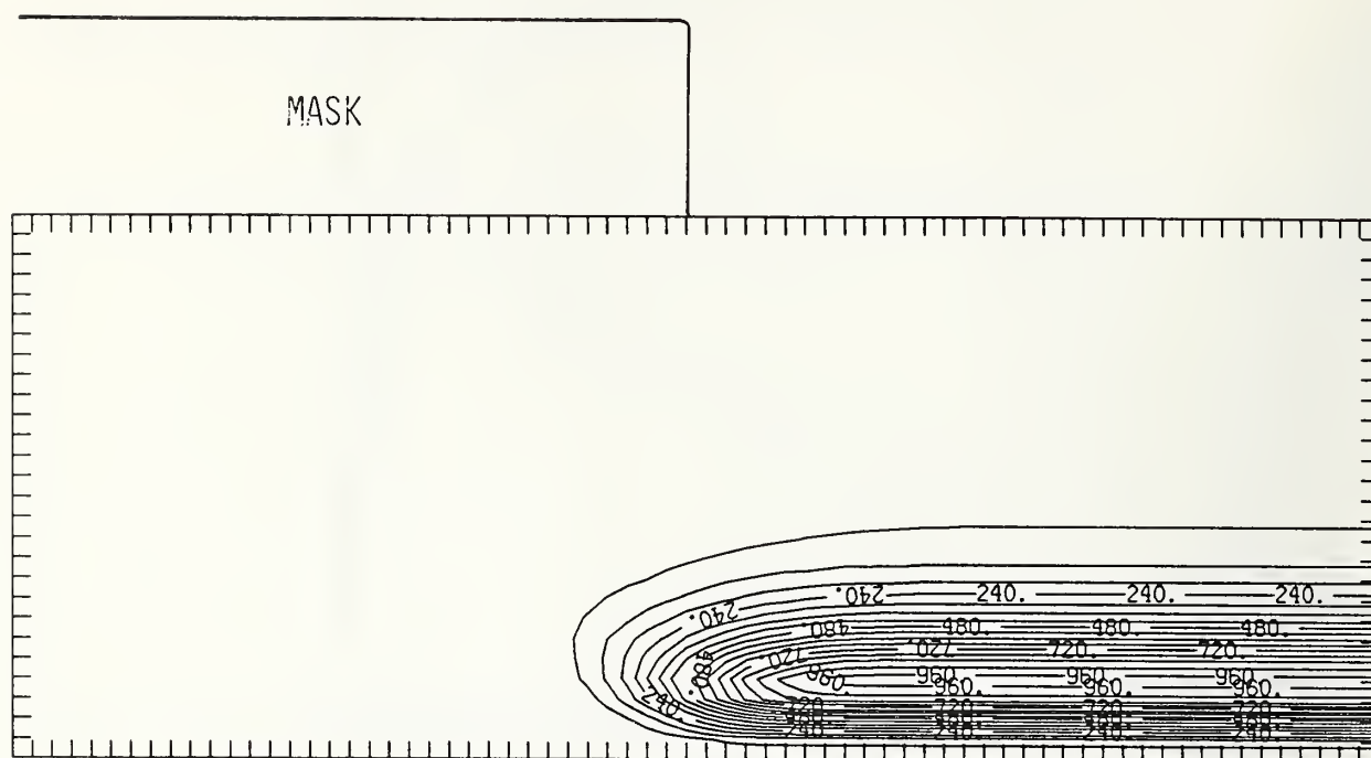
Figure B400-3 Two-dimensional distribution of 400 keV boron implanted past a mask edge. The length increment (distance between tick marks) is 0.04 \mu\text{m} and the scale factor is 1000.
