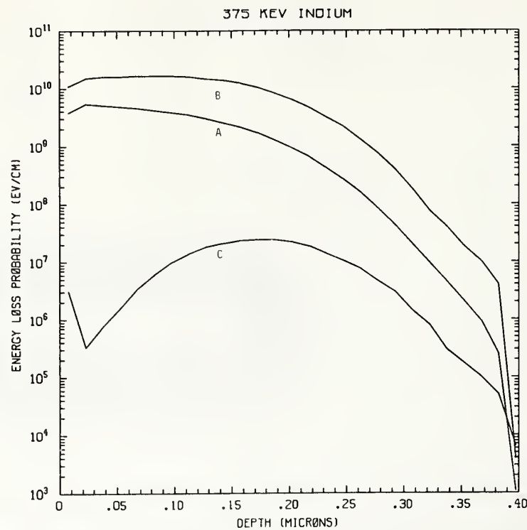
Figure In375-1 One-dimensional probability distributions for energy loss due to electronic excitation (A), displacement damage (B), and phonon excitation (C) for 375 keV indium normally incident on a silicon target.
