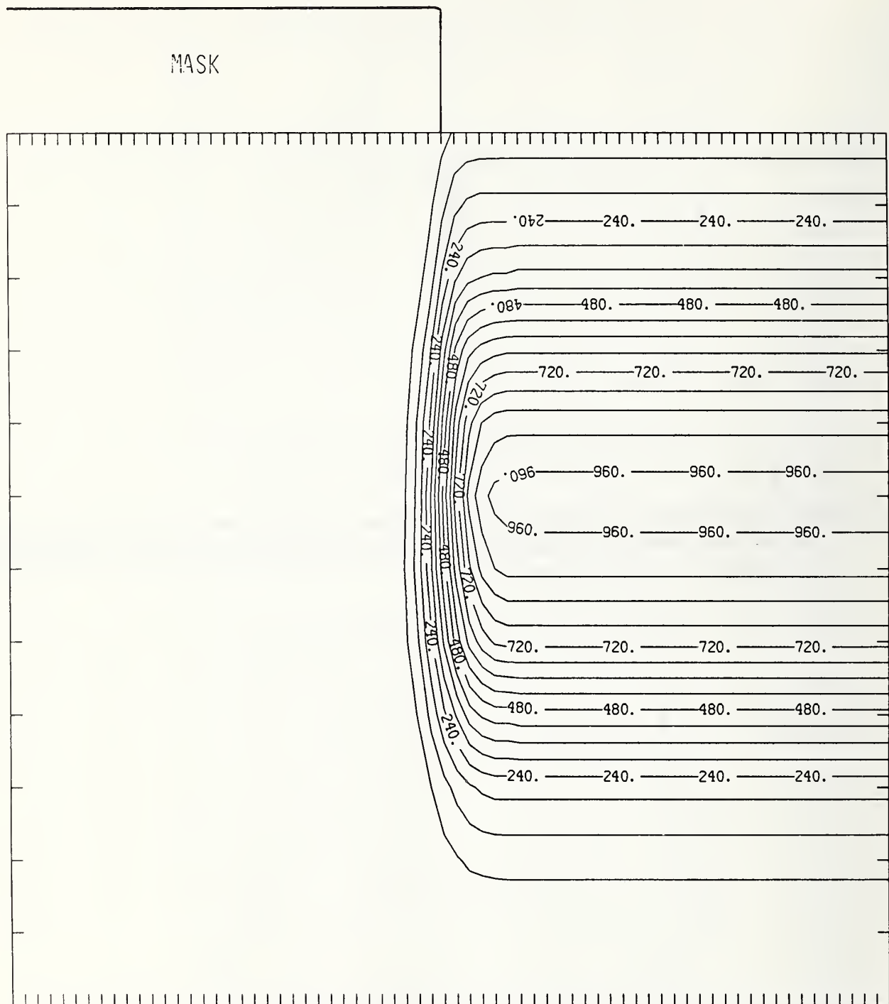
Figure Si75-3 Two-dimensional distribution of 75 keV silicon implanted past a mask edge. The length increment (distance between tick marks) is 0.02 \mu\text{m} and the scale factor is 1000.
