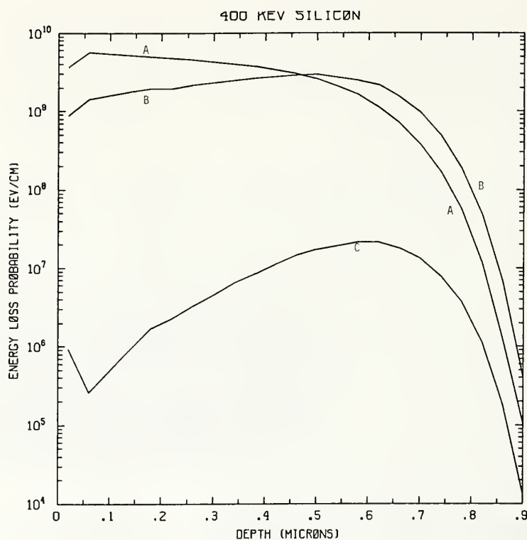
Figure Si400-1 One-dimensional probability distributions for energy loss due to electronic excitation (A), displacement damage (B), and phonon excitation (C) for 400 keV silicon normally incident on a silicon target.
