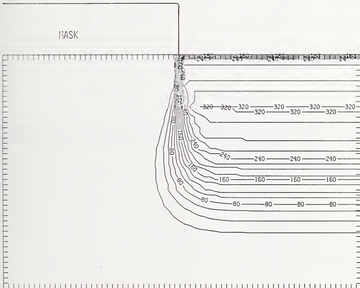
Figure As350-4 Two-dimensional distribution of Frenkel pairs created by 350 keV arsenic implanted past a mask edge. The length increment (distance between tick marks) is 0.01 \mu\text{m} and the scale factor is 0.1.
