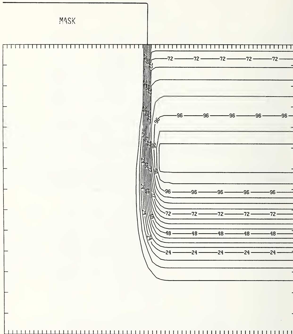
Figure Al200-4 Two-dimensional distribution of Frenkel pairs created by 200 keV aluminum implanted past a mask edge. The length increment (distance between tick marks) is 0.04 \mu\text{m} and the scale factor is 0.1.
