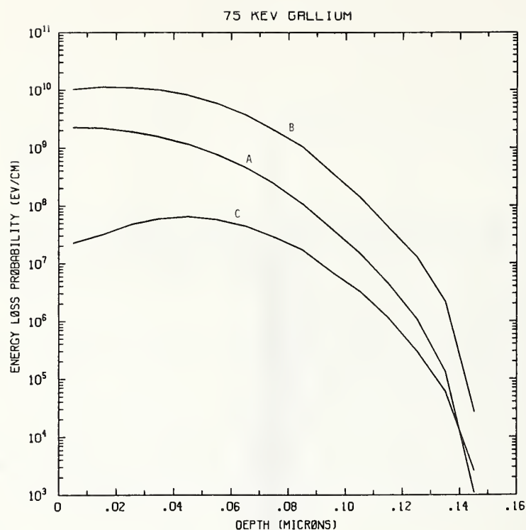
Figure Ga75-1 One-dimensional probability distributions for energy loss due to electronic excitation (A), displacement damage(B), and phonon excitation (C) for 75 keV gallium normally incident on a silicon target.
