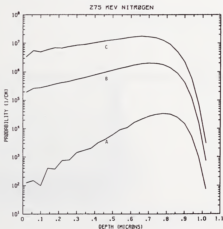
Figure N275-2 One-dimensional probability distributions for implanted nitrogen (A), primary silicon displacements (B), and Frenkel pairs (C) for 275 keV nitrogen normally incident on a silicon target.
