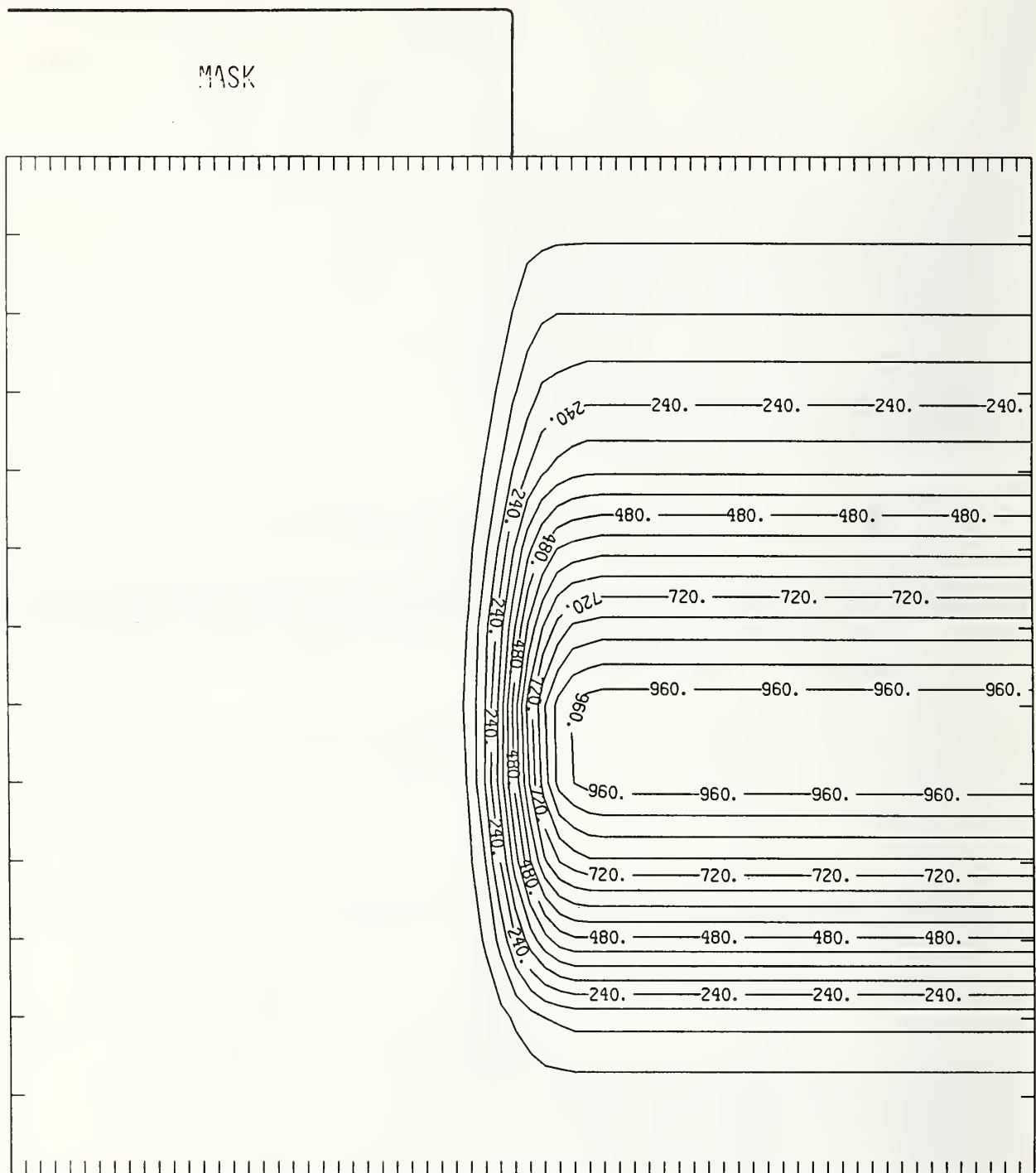
Figure Si200-3 Two-dimensional distribution of 200 keV silicon implanted past a mask edge. The length increment (distance between tick marks) is 0.04 \mu\text{m} and the scale factor is 1000.
