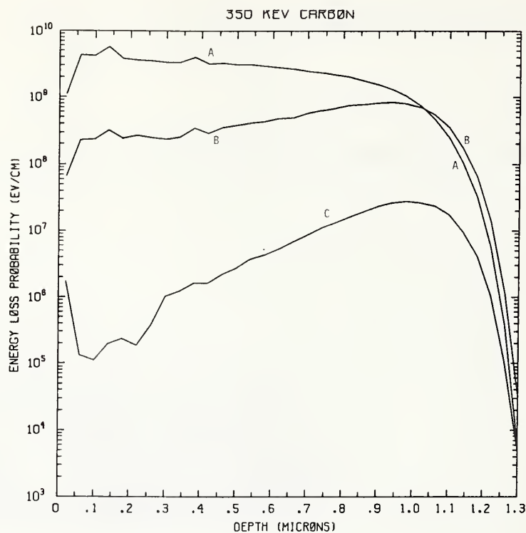
Figure C350-1 One-dimensional probability distributions for energy loss due to electronic excitation (A), displacement damage (B), and phonon excitation (C) for 350 keV carbon normally incident on a silicon target.
