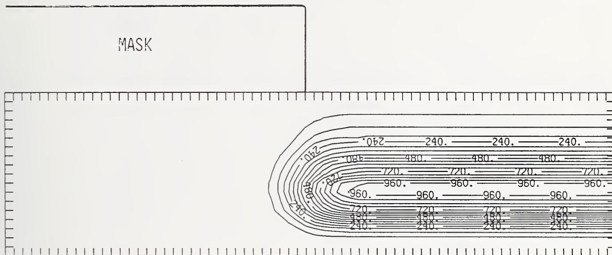
Figure S325-3 Two-dimensional distribution of 325 keV sulfur implanted past a mask edge. The length increment (distance between tick marks) is 0.04 \mu\text{m} and the scale factor is 1000.
