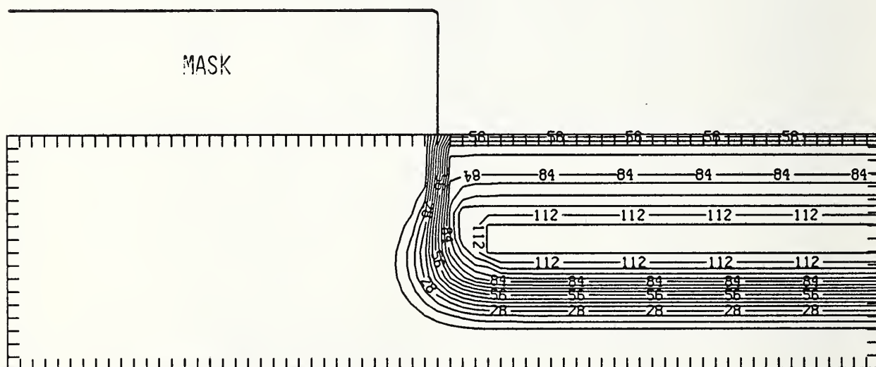
Figure Al275-4 Two-dimensional distribution of Frenkel pairs created by 275 keV aluminum implanted past a mask edge. The length increment (distance between tick marks) is 0.04 \mu\text{m} and the scale factor is 0.1.
