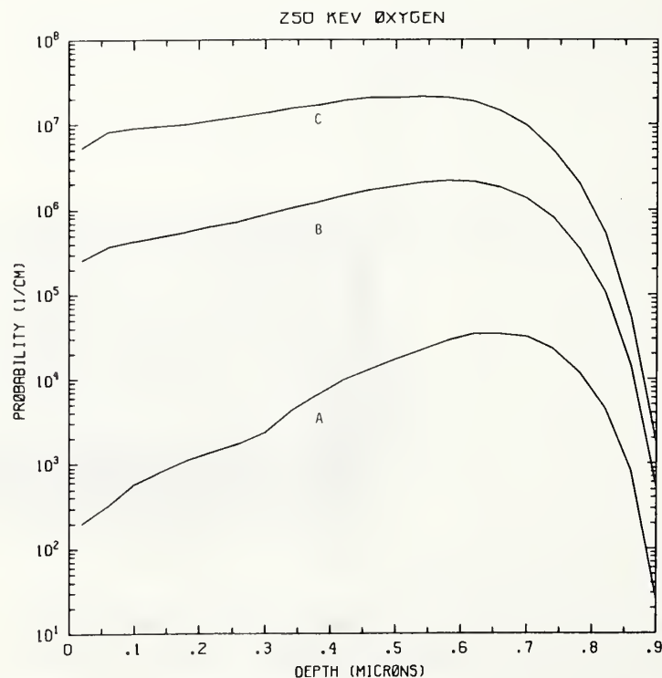
Figure O250-2 One-dimensional probability distributions for implanted oxygen (A), primary silicon displacements (B), and Frenkel pairs (C) for 250 keV oxygen normally incident on a silicon target.
