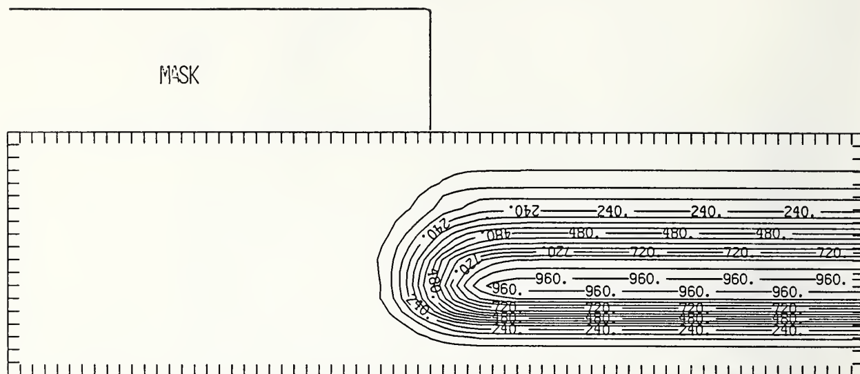
Figure P325-3 Two-dimensional distribution of 325 keV phosphorus implanted past a mask edge. The length increment (distance between tick marks) is 0.04 \mu\text{m} and the scale factor is 1000.
