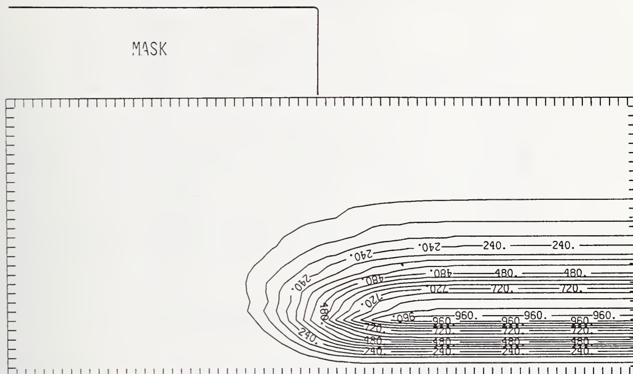
Figure B150-3 Two-dimensional distribution of 150 keV boron implanted past a mask edge. The length increment (distance between tick marks) is 0.02 \mu\text{m} and the scale factor is 1000.
