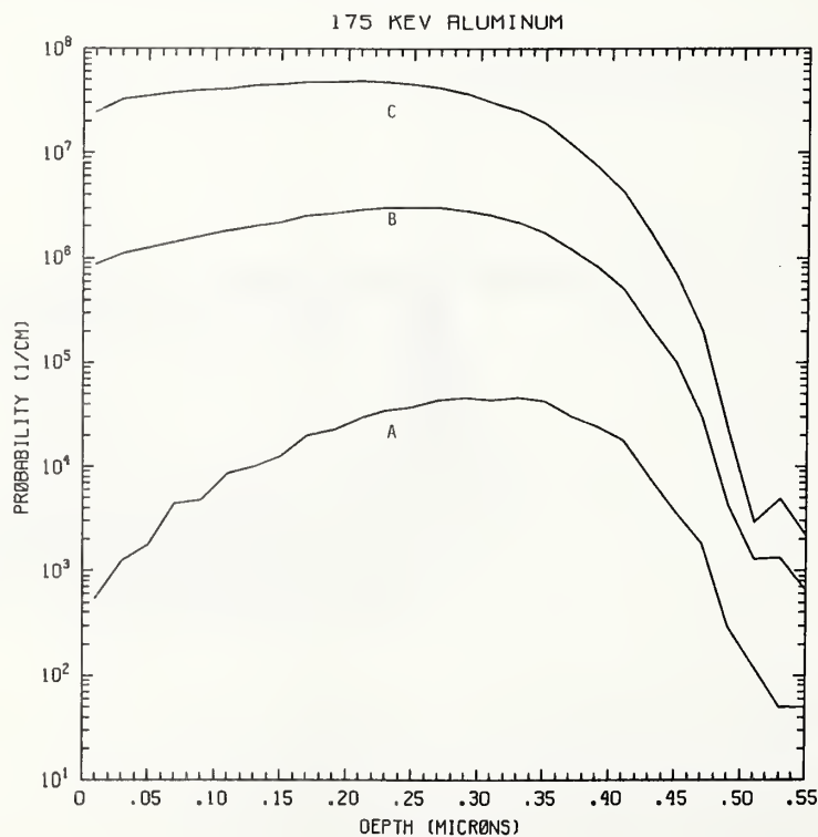
Figure Al175-2 One-dimensional probability distributions for implanted aluminum (A), primary silicon displacements (B), and Frenkel pairs (C) for 175 keV aluminum normally incident on a silicon target.
