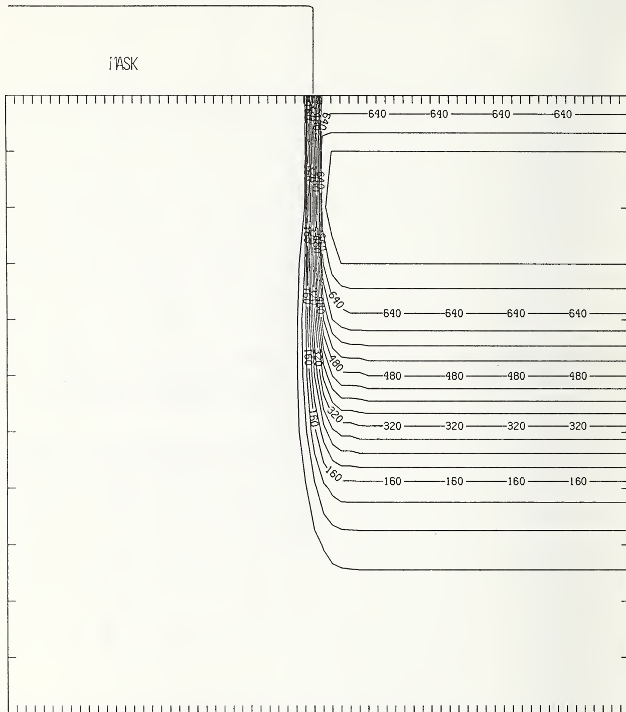
Figure P75-4 Two-dimensional distribution of Frenkel pairs created by 75 keV phosphorus implanted past a mask edge. The length increment (distance between tick marks) is 0.02 \mu\text{m} and the scale factor is 1.
