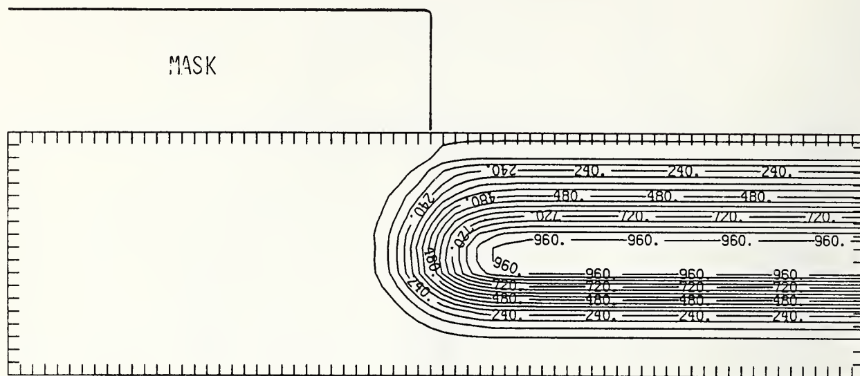
Figure Si125-3 Two-dimensional distribution of 125 keV silicon implanted past a mask edge. The length increment (distance between tick marks) is 0.02 \mu\text{m} and the scale factor is 1000.
