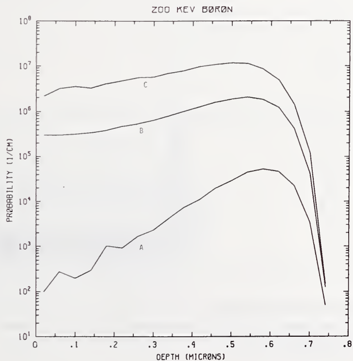
Figure B200-2 One-dimensional probability distributions for implanted boron (A), primary silicon displacements (B), and Frenkel pairs (C) for 200 keV boron normally incident on a silicon target.
