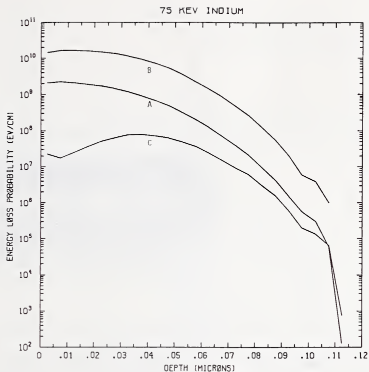
Figure In75-1 One-dimensional probability distributions for energy loss due to electronic excitation (A), displacement damage (B), and phonon excitation (C) for 75 keV indium normally incident on a silicon target.
