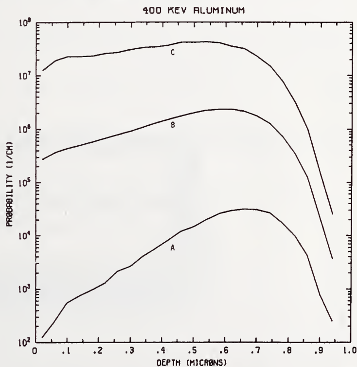
Figure Al400-2 One-dimensional probability distributions for implanted aluminum (A), primary silicon displacements (B), and Frenkel pairs (C) for 400 keV aluminum normally incident on a silicon target.
