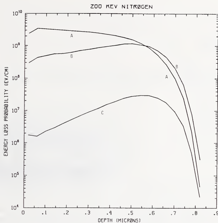
Figure N200-1 One-dimensional probability distributions for energy loss due to electronic excitation (A), displacement damage (B), and phonon excitation (C) for 200 keV nitrogen normally incident on a silicon target.
