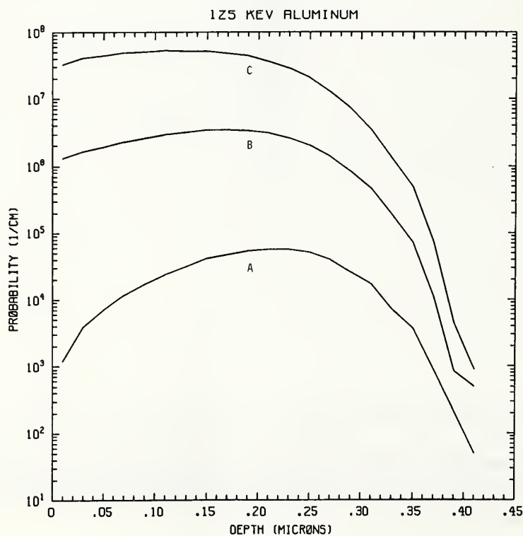
Figure A1125-2 One-dimensional probability distributions for implanted aluminum (A), primary silicon displacements (B), and Frenkel pairs (C) for 125 keV aluminum normally incident on a silicon target.
