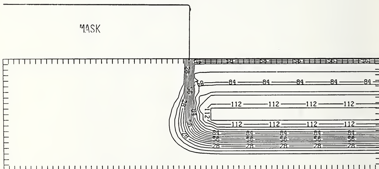
Figure Al325-4 Two-dimensional distribution of Frenkel pairs created by 325 keV aluminum implanted past a mask edge. The length increment (distance between tick marks) is 0.04 \mu\text{m} and the scale factor is 0.1.
