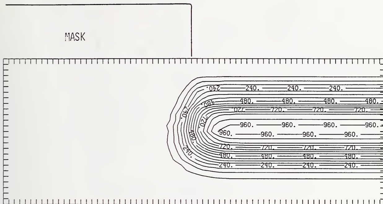
Figure Ge375-3 Two-dimensional distribution of 375 keV germanium implanted past a mask edge. The length increment (distance between tick marks) is 0.02 \mu\text{m} and the scale factor is 1000.
