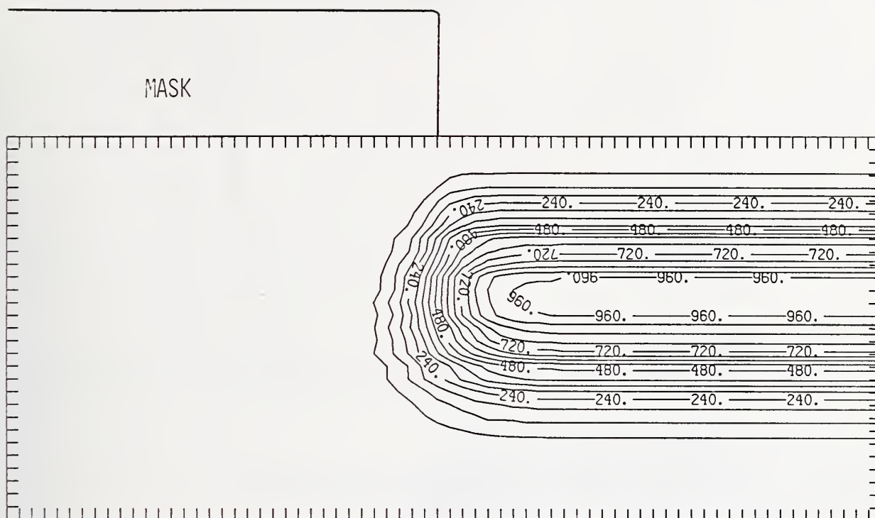
Figure As200-3 Two-dimensional distribution of 200 keV arsenic implanted past a mask edge. The length increment (distance between tick marks) is 0.01 \mu\text{m} and the scale factor is 1000.
