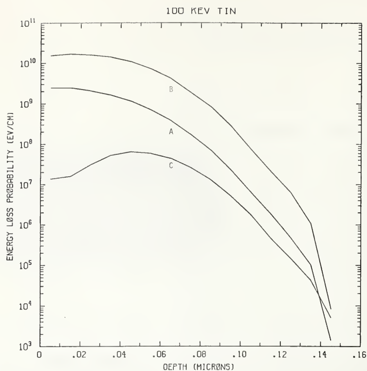
Figure Sn100-1 One-dimensional probability distributions for energy loss due to electronic excitation (A), displacement damage (B), and phonon excitation (C) for 100 keV tin normally incident on a silicon target.
