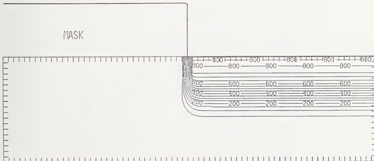
Figure Pt75-4 Two-dimensional distribution of Frenkel pairs created by 75 keV platinum implanted past a mask edge. The length increment (distance between tick marks) is 0.005\ \mu\text{m} and the scale factor is 1.
