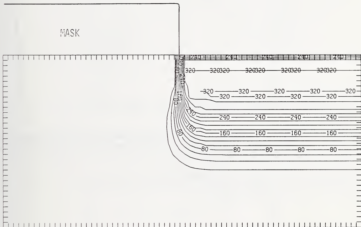
Figure Sb325-4 Two-dimensional distribution of Frenkel pairs created by 325 keV antimony implanted past a mask edge. The length increment (distance between tick marks) is 0.01 \mu\text{m} and the scale factor is 0.1.
