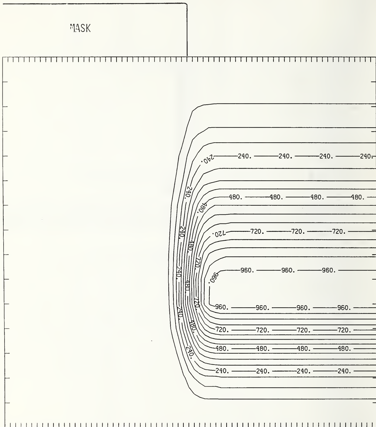
Figure S275-3 Two-dimensional distribution of 275 keV sulfur implanted past a mask edge. The length increment (distance between tick marks) is 0.04 \mu\text{m} and the scale factor is 1000.
