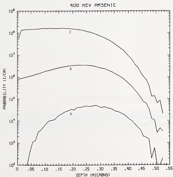
Figure As400-2 One-dimensional probability distributions for implanted arsenic (A), primary silicon displacements (B), and Frenkel pairs (C) for 400 keV arsenic normally incident on a silicon target.
