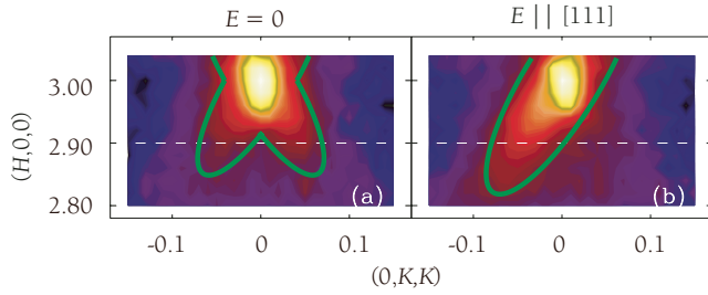
FIGURE 1: Contour plots (log-scale) of the neutron diffuse scattering intensity measured at 300 K ( < T_c ) in the (HKK) reciprocal scattering plane close to the (300) Bragg peak. The panels show data taken after the sample was (a) zero-field cooled (ZFC) and (b) field-cooled (FC) below T_c for electric field E \parallel [111] . The solid green lines are guides to the eye to emphasize the (a) symmetric and (b) asymmetric shapes of the diffuse scattering.
