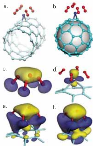
FIGURE 2: The symmetric and the most energetically the most stable configurations of four H 2 molecules absorbed on a (a) Ti-coated nanotube and (b) C 60 . (c) The antibonding orbital of the four H 2 complex; (d)-(f) Isosurfaces of the bonding orbital at three different values, indicating the involvement of H-antibonding, Ti d-orbitals, and C π-orbitals in the bonding mechanism.
