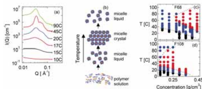
FIGURE 1: (a) SANS intensity of 0.21 \text{g/cm}^3 F108 Pluronic solution at several temperatures. (b) Schematic pictures of the polymer structure implied by the SANS. (c) and (d) Phase diagrams for F68 and F108 Pluronic solutions as determined by SANS. Three phases are identified: polymers dissolved in solution (black), micelles with liquid-like order (blue), and micelles with crystalline order (red).
