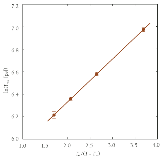
FIGURE 1: The temperature dependence of the residence time for the translational diffusion component of “slow” (inner layer) surface water in \text{ZrO}_2 fitted with a VFT law, \tau = \tau_0 \exp(DT_0/(T-T_0)) , and plotted as a function of T_0/(T-T_0) , with T_0 = 189 K.
