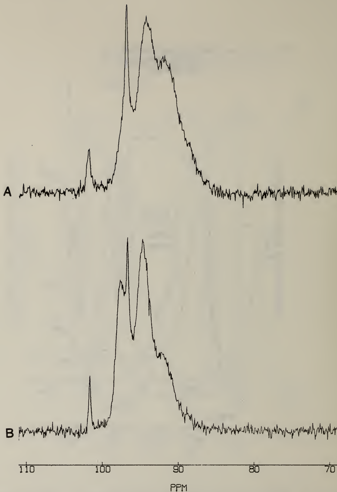
Figure 10. ^{119}\text{Sn} NMR at 74.6 MHz of OMPs in benzene. (A) OMP-2N; (B) OMP-8N. In each spectrum the sharp peak at about 97 ppm arises from unreacted TBTM.
