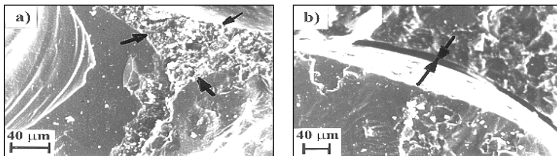
Figure 13. SEM micrographs showing examples of PC microstructure with dry (a) and wet (b) aggregate, which had caused different levels of adhesion.
