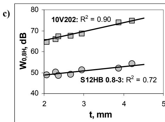
Figure 26. Amplification coefficient W_{0,8H} plotted against the estimated thickness t_{U-E} for epoxy floor systems tested with transducers: a) S12HB0.8-3 and b) 10V202; c) amplification coefficient W_{0,8H} vs. "true" thickness for both transducers after 28 d of floor hardening.
