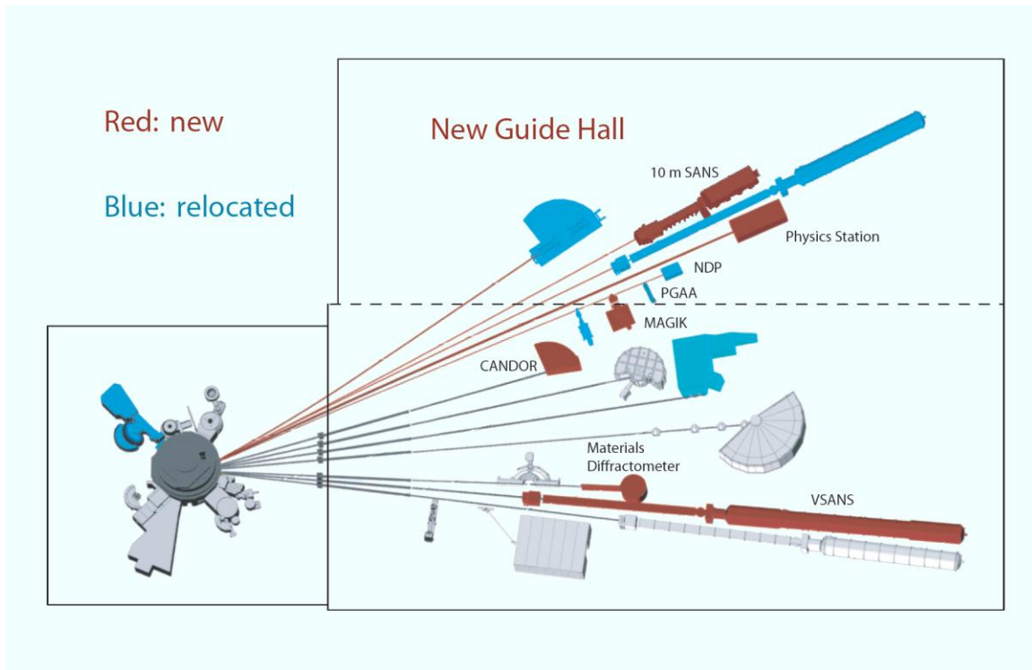
Schematic array of the cold neutron instruments expected to be operational in the expanded NCNR guide hall at the end of 2014.
