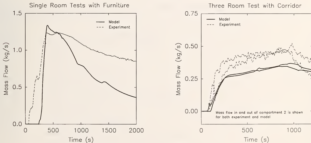
Figure 26. Comparison of measured and predicted mass flow through vents for several tests. (Numbers indicate comparable rooms in the test structure.)
