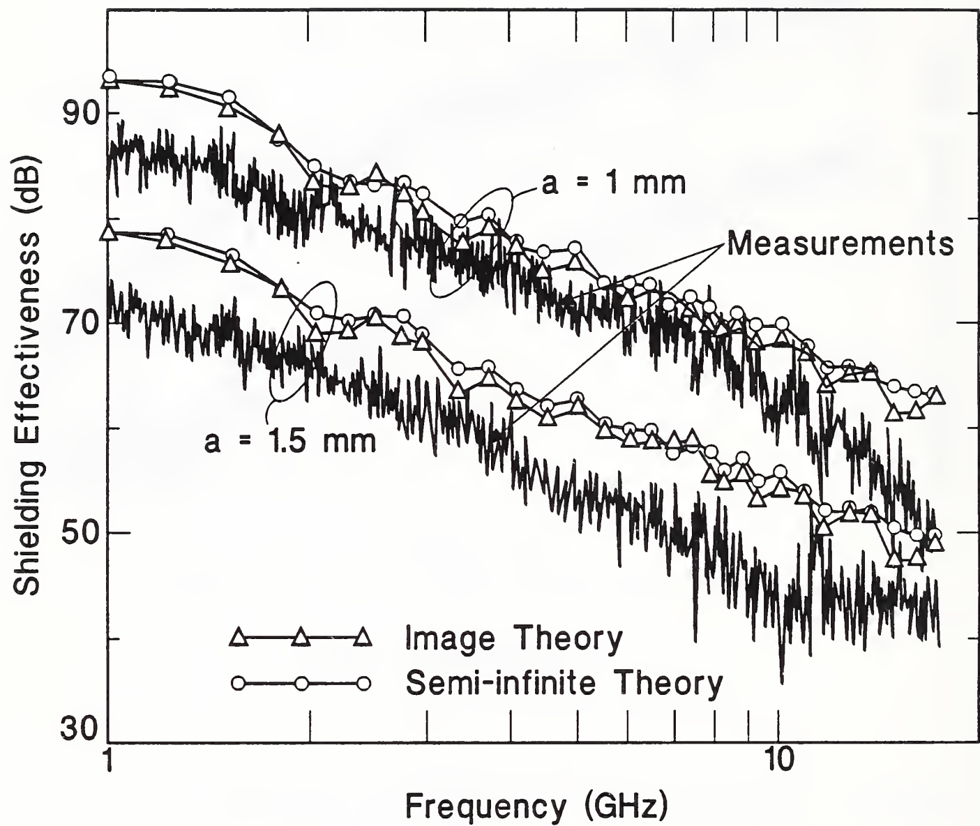
Figure 5. Semi-infinite theory, image theory, and measurements for shielding effectiveness of a coaxial air line. Both theories are modified to include wall thickness.
