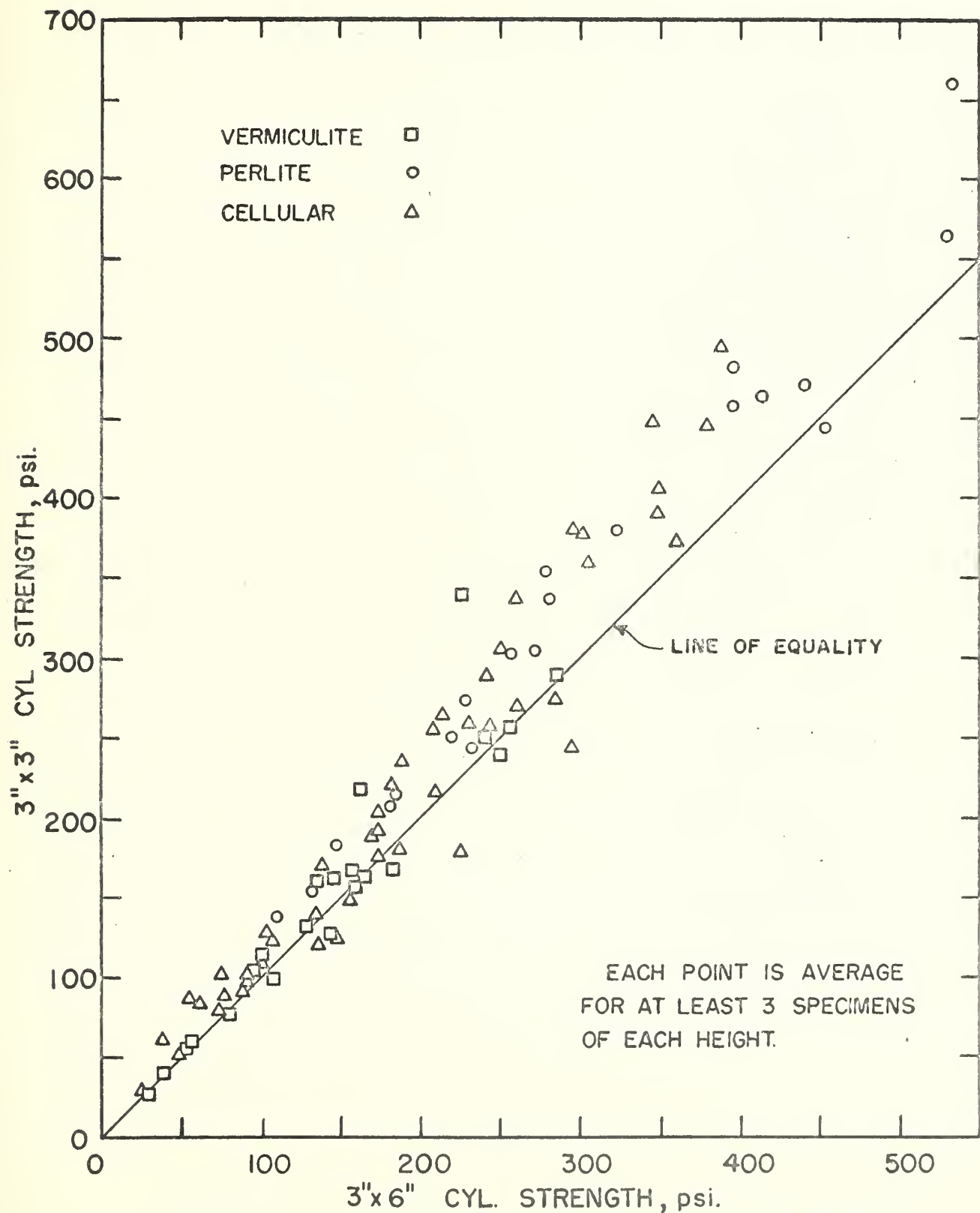
EFFECT OF HEIGHT OF SPECIMEN ON COMPRESSIVE STRENGTH OF INSULATING CONCRETE
