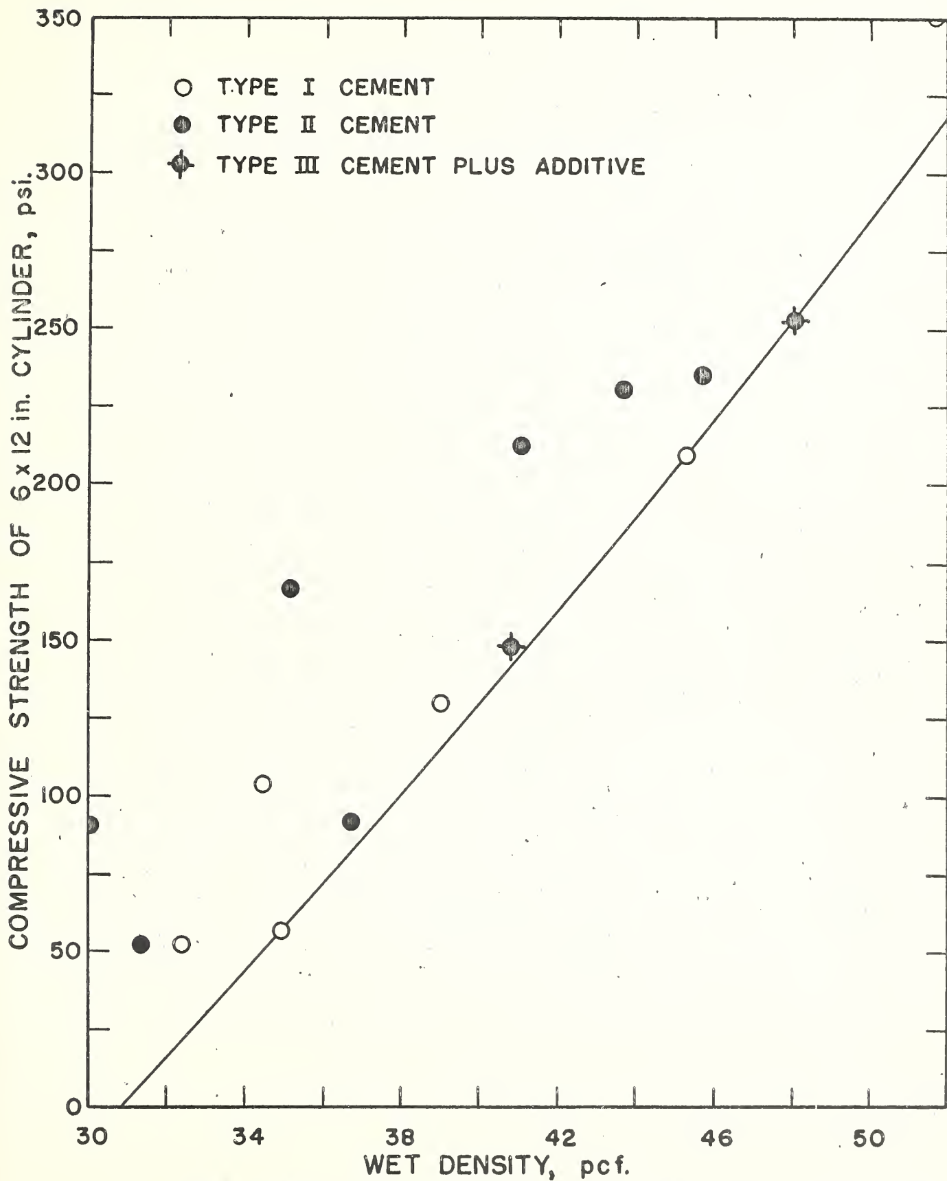
WET DENSITY VS. STRENGTH OF CELLULAR CONCRETES
