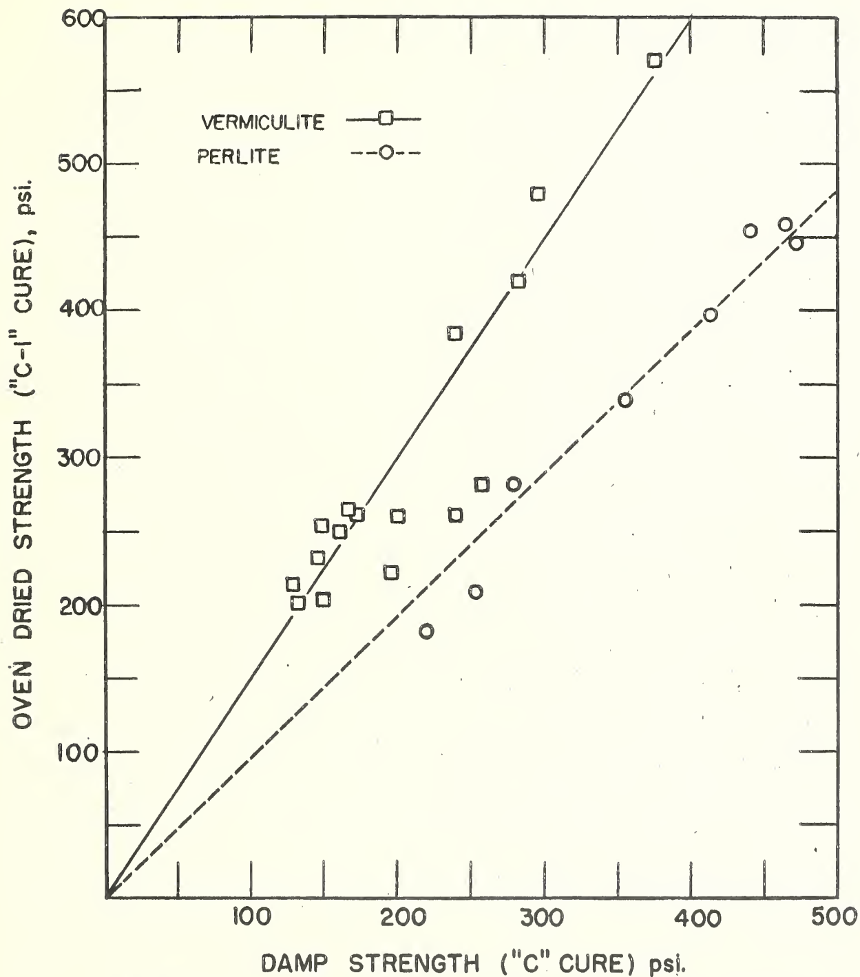
EFFECT OF OVEN DRYING ON STRENGTH OF MOIST CURED SPECIMENS OF INSULATING CONCRETE
