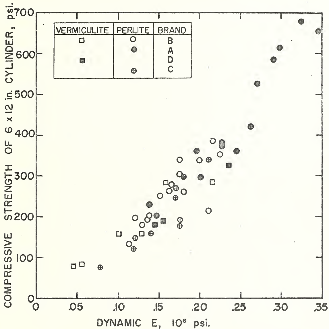
RELATION BETWEEN DYNAMIC E AND COMPRESSIVE STRENGTH
