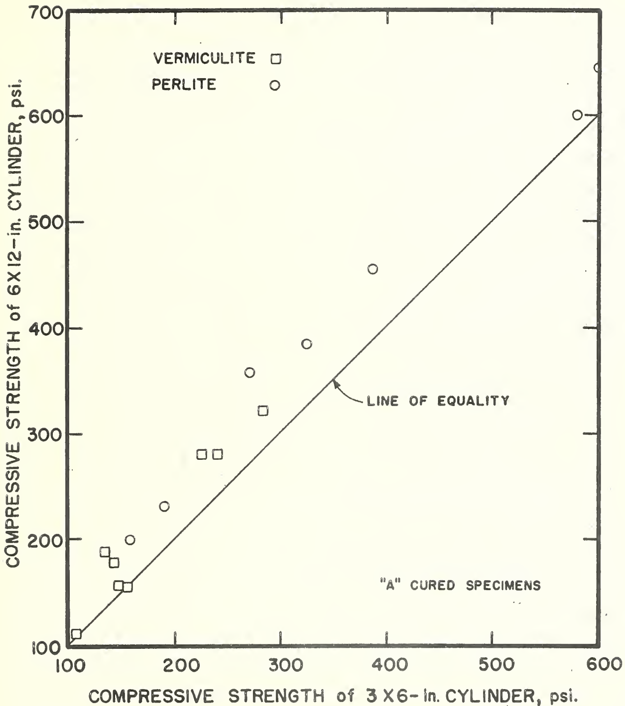
6-X 12-in VS 3-X 6-in. CYLINDER STRENGTH
