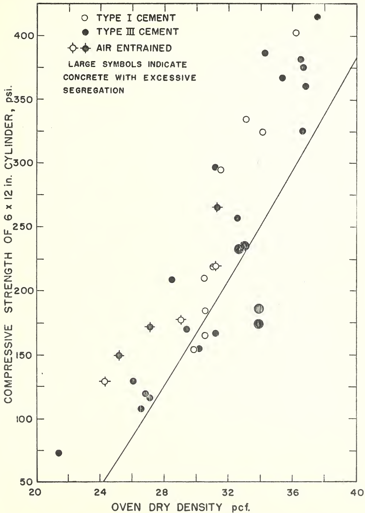
OVEN DRY DENSITY VS. STRENGTH — PERLITE C
