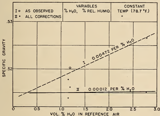
FIGURE 30.—Humidity coefficient of the Sigma recorder No. 7 determined at constant temperature ( 78.7^{\circ}\text{F} ) with test mixture 2; \circ as observed, and \bullet after the application of all corrections.
