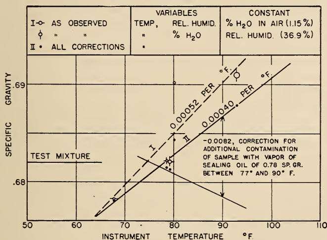
FIGURE 25.—Temperature coefficients of the Anubis recording gas gravimeter determined with test mixture 2, as observed (—○— at constant percentage of water vapor in the reference air (1.15 percent); ○ at constant relative humidity of the reference air (36.9 percent)), and ● after the application of all corrections.
