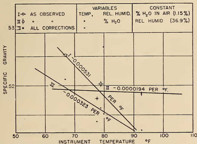
FIGURE 29.—Temperature coefficients of the Sigma recorder No. 7 determined with test mixture 2, as observed (○ at constant percentage of water vapor in the reference air (1.15 percent); ○ at constant relative humidity of the reference air (36.9 percent)), and ● after the application of all corrections.
