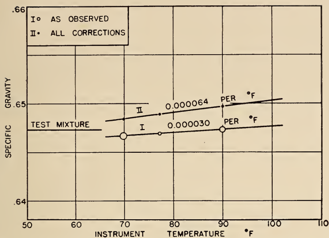
FIGURE 11.—Temperature coefficient of the Ac-Me Junior specific gravity balance No. 4041 determined with test mixture I, as observed and after the application of corrections for the temperature of the mercury in the manometer and for carbon dioxide in the reference air.
