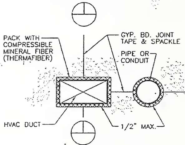
ELEVATION DETAILS OF FIRESTOPPING OF TYP. OPENING IN RATED WALL ABOVE CEILING
