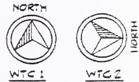
TYPICAL TENANT FLOOR PLAN ZONES FOR FLOOR NATURAL FREQUENCY MEASUREMENT
