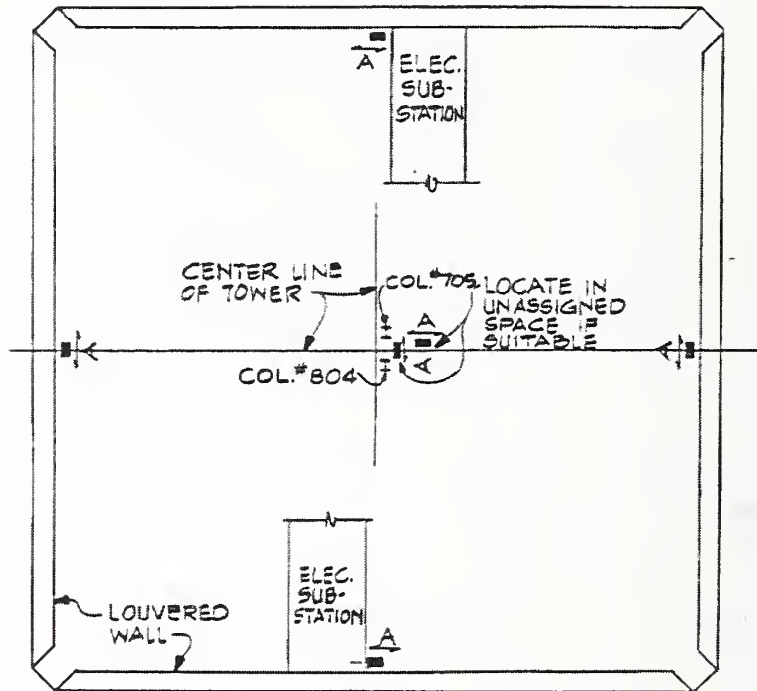
75 TH FLOOR PLAN MECHANICAL EQUIPMENT ROOM 2 WTC
