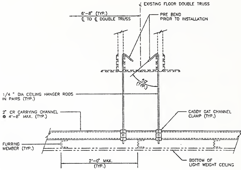
LIGHT WEIGHT CEILING SUPPORT SYSTEM FOR FLOORS W/DOUBLE TRUSSES
