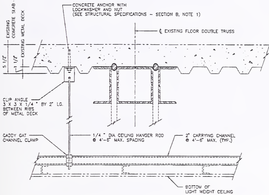
SECTION S-1
