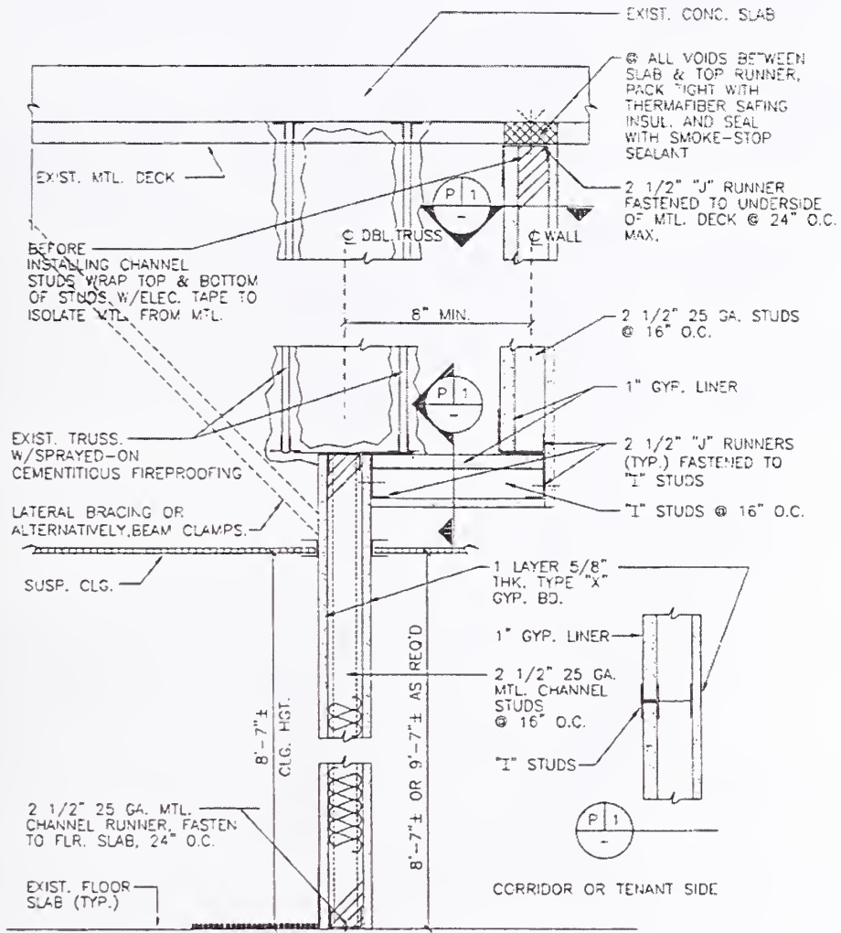
⊙ TYP. 1-HR PARTITION W/OFFSET 0 1' 2' SCALE IN FEET
