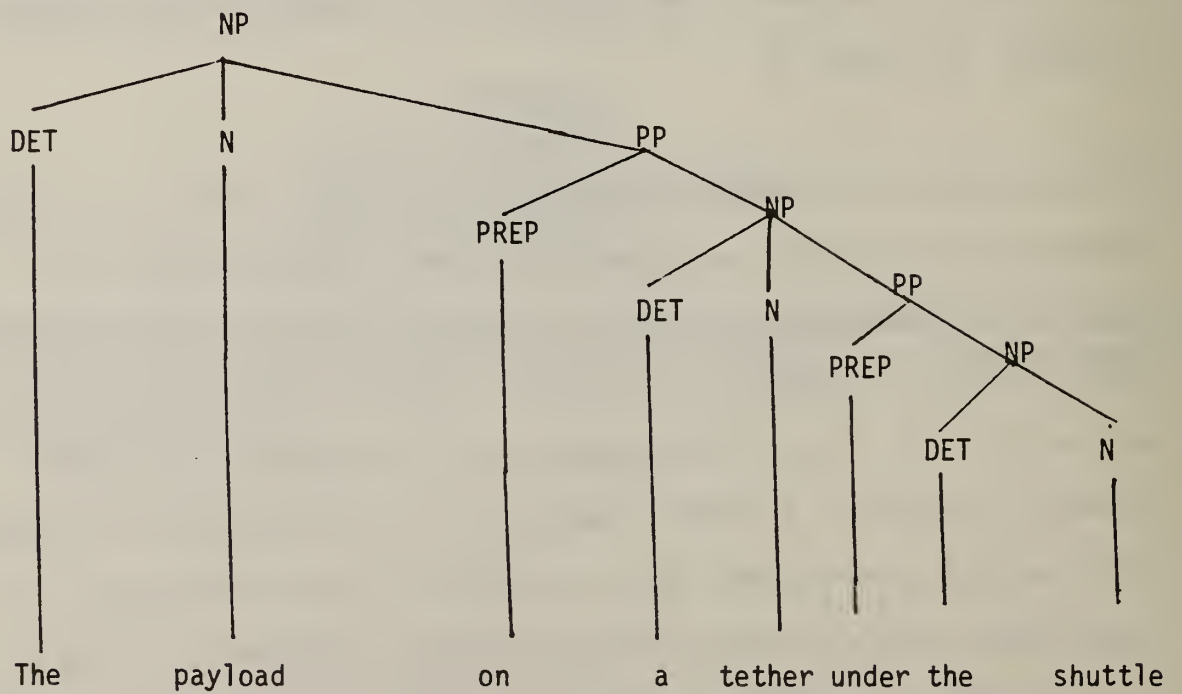
Figure 2b. Parse Tree Representation of the Noun Phrase Surface Structure.
