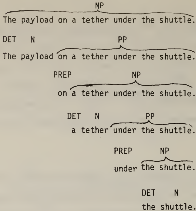
Figure 2a. Example Noun Phrase Decomposition
