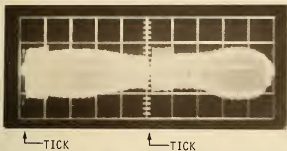
FIGURE 5.9 OSCILLOSCOPE DISPLAY OF WWV TICK AT A SWEEP RATE OF 0.2 SECOND/DIVISION.
