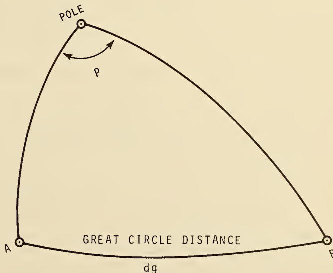
FIGURE 5.24. DIAGRAM FOR GREAT CIRCLE DISTANCE CALCULATIONS.
