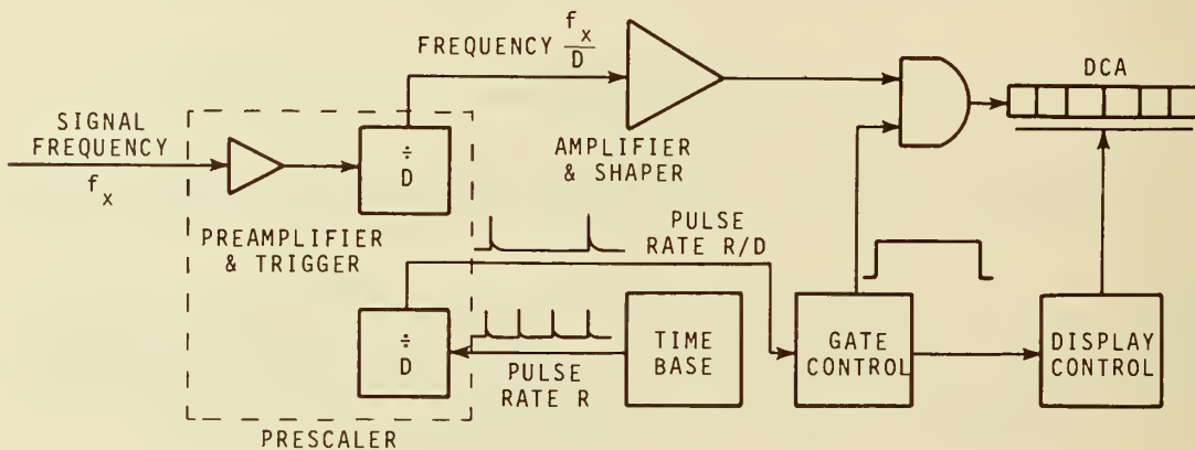
FIGURE 4.4. PRESCALER-COUNTER COMBINATION.
