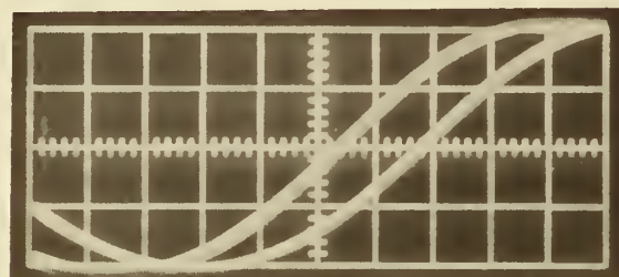
FIGURE 5.23. OSCILLOSCOPE DISPLAY USING PATTERN DRIFT METHOD.
