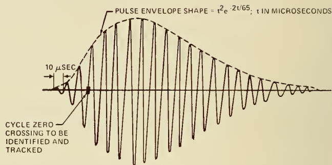
FIGURE 9.2. THE 100 kHz LORAN-C PULSE.
