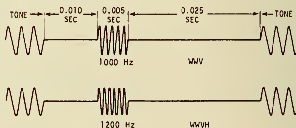
FIGURE 5.1. FORMAT OF WWV/WWVH SECONDS PULSES.
