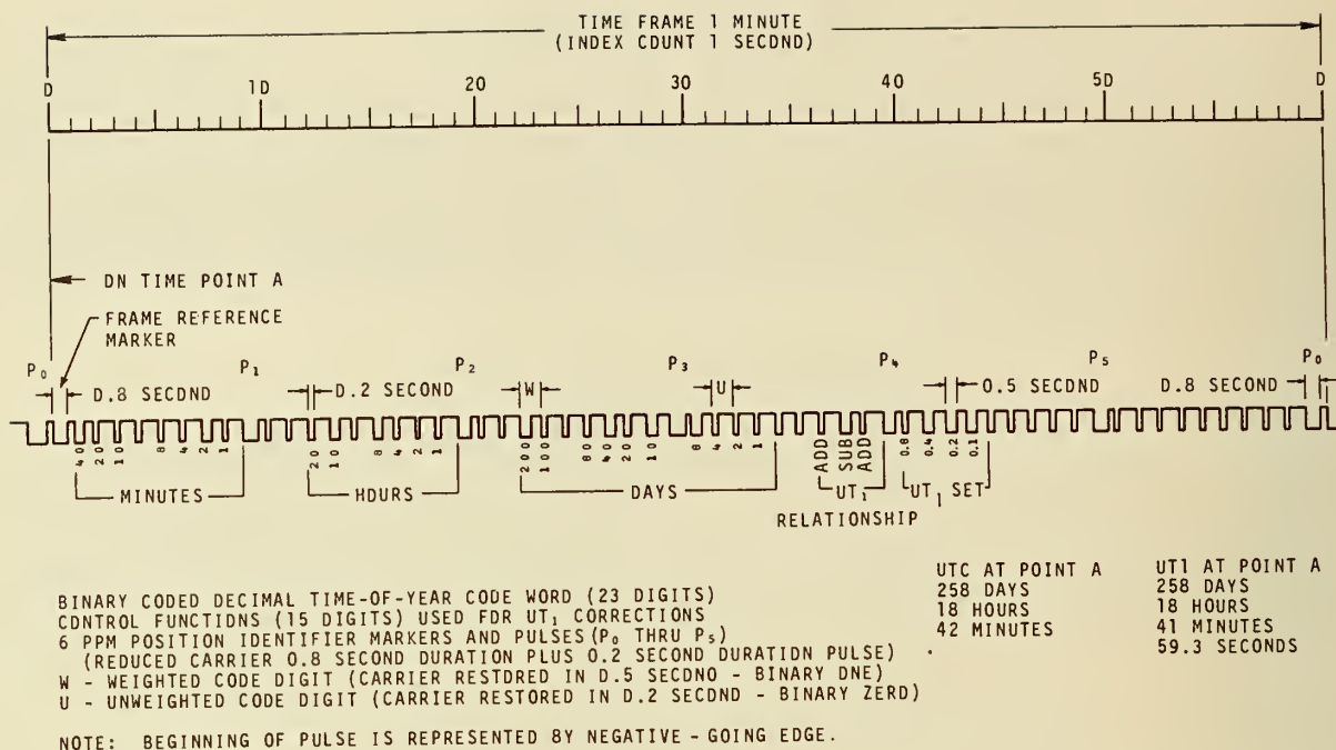
FIGURE 6.11. WWVB TIME CODE FORMAT.
