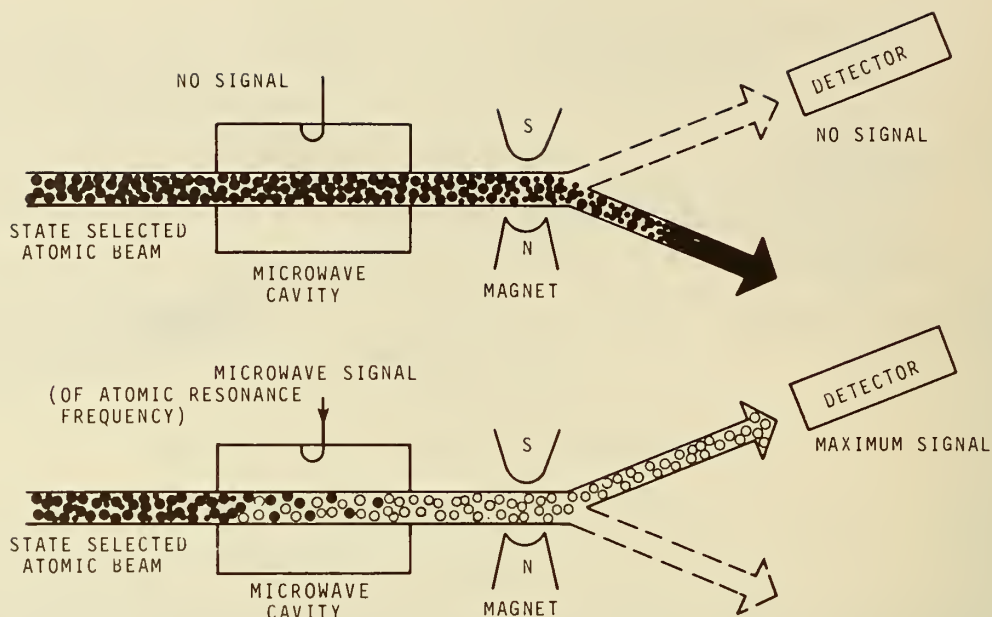
FIGURE 10.17. ATOM DETECTION.
