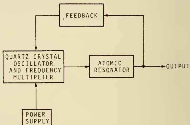
FIGURE 10.20. ATOMIC FREQUENCY OSCILLATOR.
