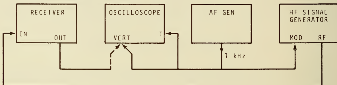
FIGURE 5.6. EQUIPMENT SETUP FOR RECEIVER TIME DELAY MEASUREMENTS.
