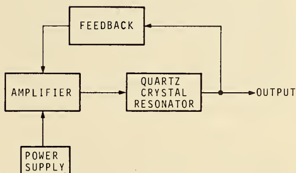
FIGURE 10.12. QUARTZ CRYSTAL OSCILLATOR.
