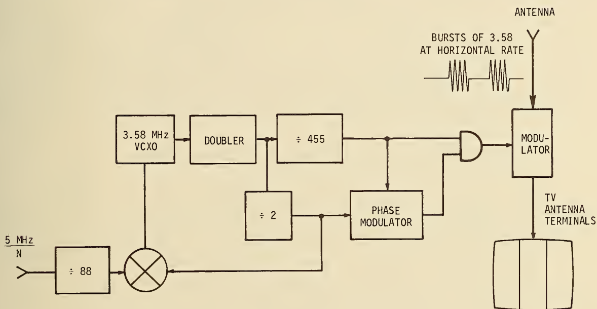
FIGURE 7.3. BLOCK DIAGRAM OF COLOR BAR COMPARATOR.
