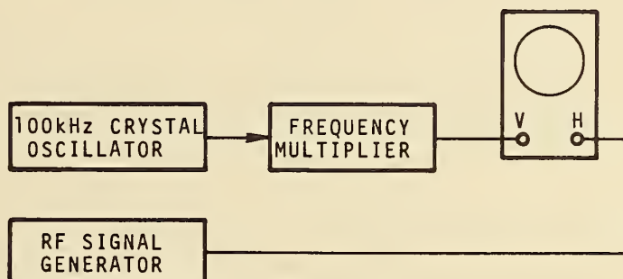
FIGURE 4.33. ARRANGEMENT FOR CALIBRATING A SIGNAL GENERATOR.
