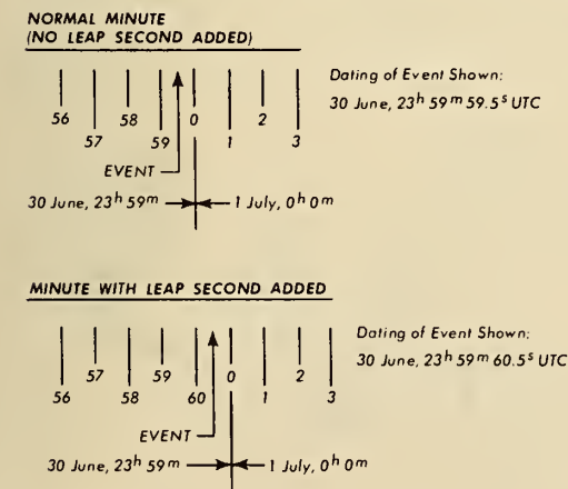
FIGURE 2.4. DATING OF EVENTS IN THE VICINITY OF A LEAP SECOND.
