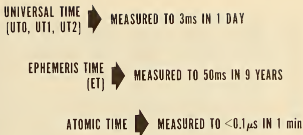
FIGURE 2.3. CLASSES OF TIME SCALES & ACCURACIES.
