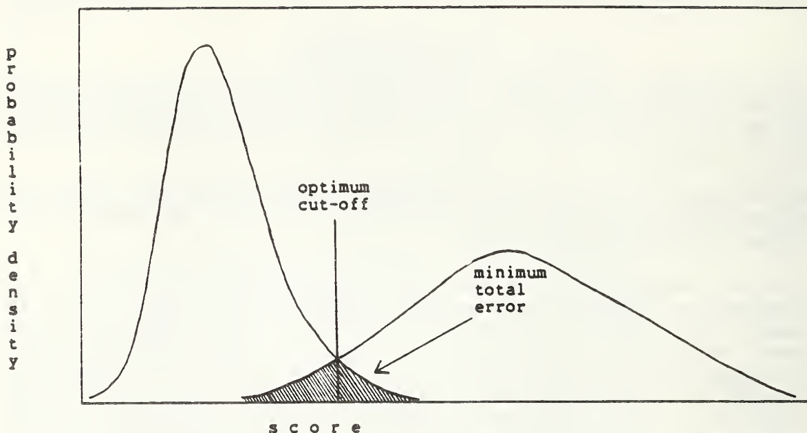
Figure 19. Theoretical match and mismatch score distributions showing the relationship of the optimum cutoff point to the density functions, and with the minimum total error area shaded in.
