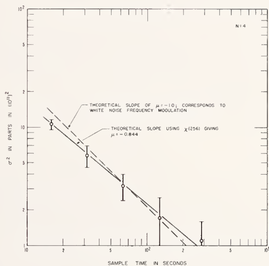
Fig. 5. Cesium beam (NBS III), N^{15}H_3 maser (2) comparison; standard deviation of the frequency fluctuations as a function of sampling time.
