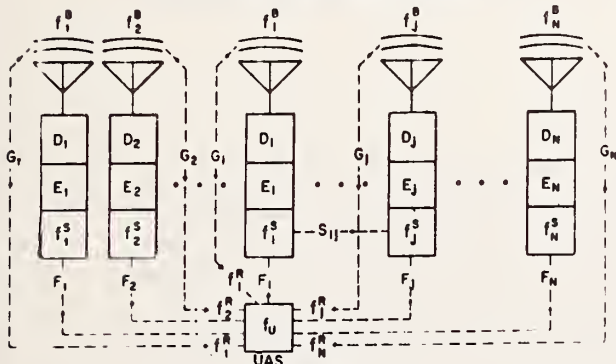
Figure 6: The coordinate time system resembles an electrical network. Ideal values of emitted frequencies f_j^B , are indicated, as are ideal values f_j^R , of received frequencies, and the rates f_j^S of the standards, and f_u of the system unified mean standard. Not shown are the observed emitted frequencies f_j^E , and actually received frequencies f_j^A . The measured or inferred rate intercomparison of the i^{\text{th}} and j^{\text{th}} local standards is indicated by the fractional frequency difference S_{ij} .
