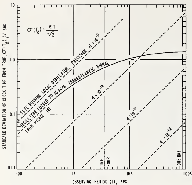
FIGURE 6. Clock-time deviations from original setting as a function of observing period. ( 6 Pierce 1957).
