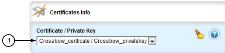
Figure 2-57 Certificates Info
