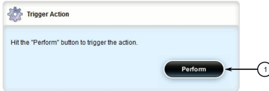
Figure 2-58 Trigger Action
