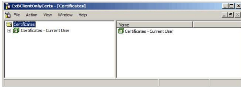
Figure 2-48 CxBClientOnlyCerts Snap-In
