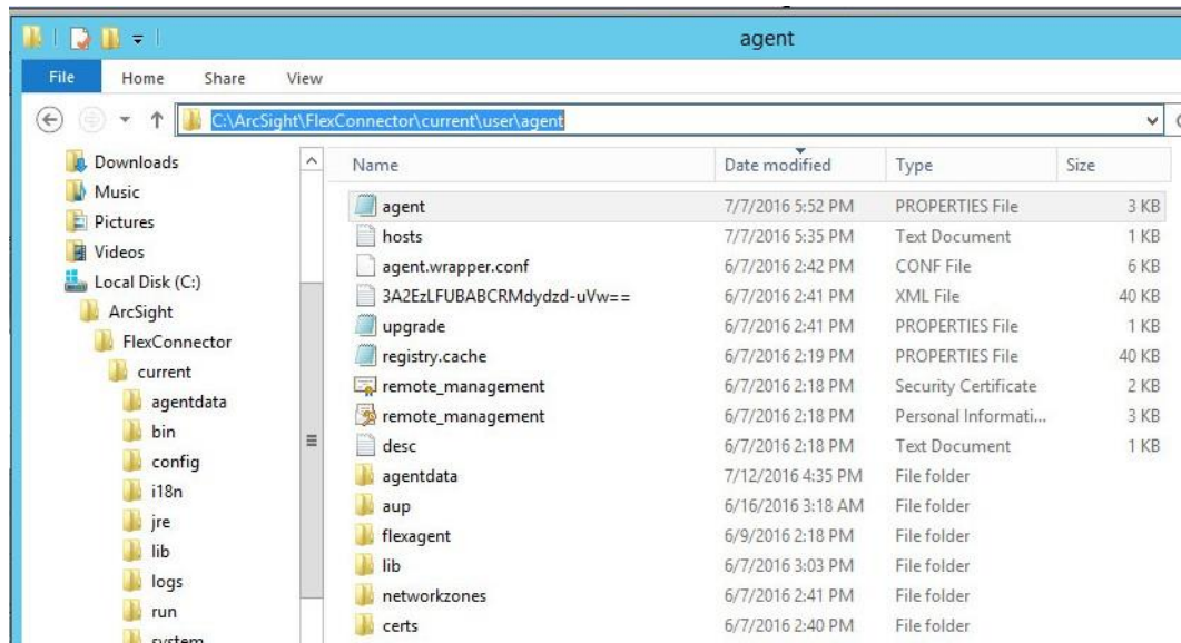
Figure 2-91 Example String/URL
