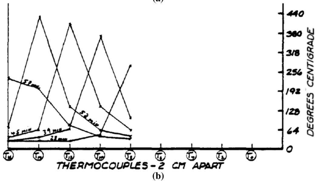
Figure 11. Thermocouple temperatures located on the contact line between the bottom surface of a covered 160 mm cigarette and the substrate of duck dyed blue fabric over polyurethane for (a) temperature versus time and (b) temperature versus thermocouple location. [30]
