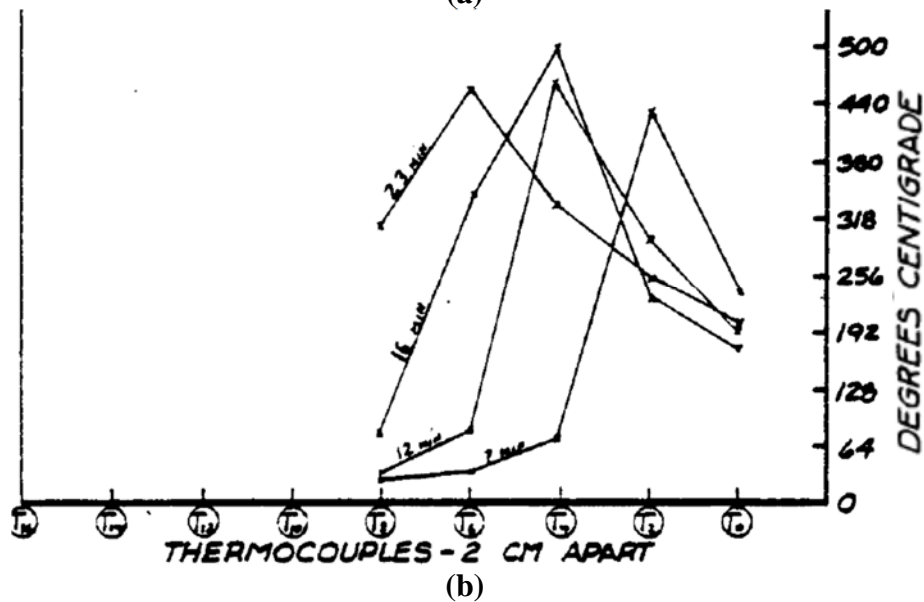
Figure 10. Thermocouple temperatures located on the contact line between the bottom surface of a covered 80 mm cigarette and the substrate of greige duck fabric over polyurethane for (a) temperature versus time and (b) temperature versus thermocouple location. [30]
