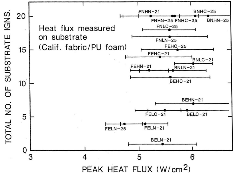
Figure 16. Number of substrate ignitions versus average peak heat flux estimates for various cigarettes on a one-cushion mock-up. [10]
