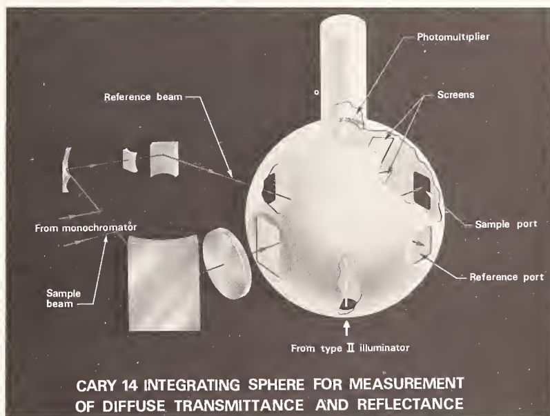
PLATE I. Layout of the optical configuration of the Cary 1411 sphere attachment.
