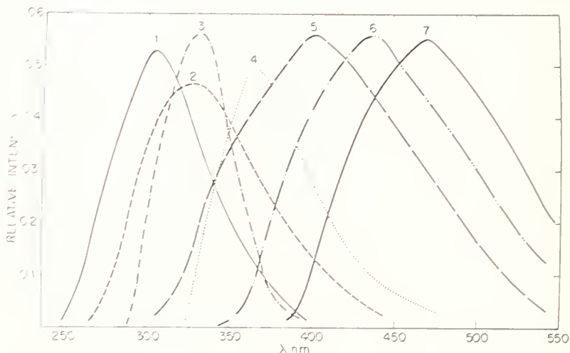
FIGURE 17. Matrix effects on position of emission band of Tl^+ , Ce^{3+} , Pb^{2+} , and Cu^+ . I. Phosphate: Tl^+ ; II. Borax: Tl^+ ; III. Phosphate: Ce^{3+} ; IV. Borax: Ce^{3+} ; V. Borax: Pb^{2+} ; VI. Germanate: Pb^{2+} ; VII Phosphate: Cu^+ .
