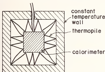
FIGURE 6. Conduction calorimeter.
