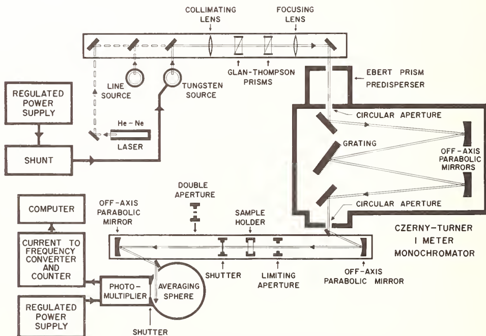
FIGURE 1. High-accuracy spectrophotometer.
