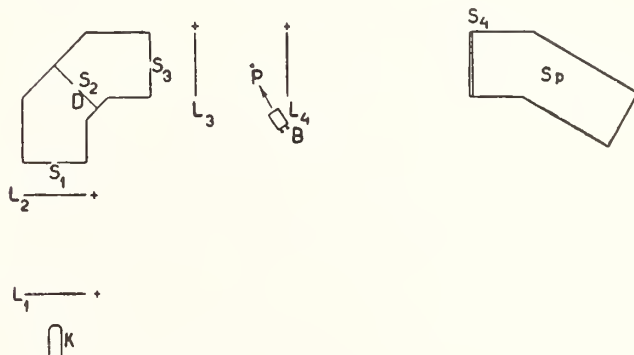
FIGURE 9. Krijgsman's arrangement [32] for the absolute calibration of an arbitrary source K. D, double monochromator with slits S_1 , S_2 , S_3 ; P, image of K; Sp, spectrograph with horizontal slit S_4 .
