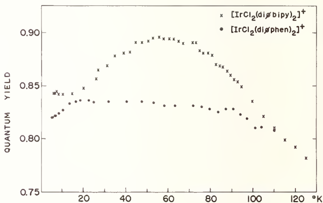
FIGURE 5. Temperature dependence of quantum yields. X, cis -dichlorobis(4,4'-diphenyl-2,2'-bipyridine)iridium(III) chloride. O, cis -dichlorobis(4,7-diphenyl-1,10-phenanthroline)iridium(III) chloride. Both molecules were dissolved in poly(methylmethacrylate) and irradiated with \sim 365 nm radiation.
