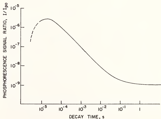
FIGURE 9. Plot of phosphorescence signal ratio (ratio of integrated intensity I to the steady state integrated intensity I_{p0} ) versus sample phosphorescence decay time \tau [60] for case of pulsed source gated detector (see text for values of t_f , t_p , and t_d ).
