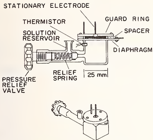
FIGURE 10. Flash calorimeter.
