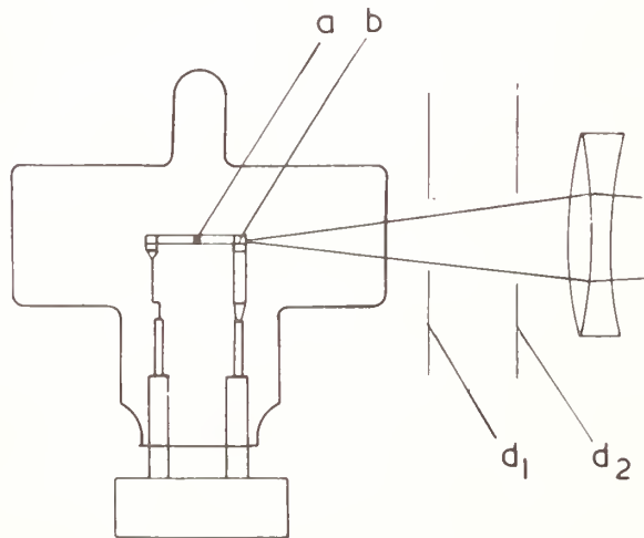
FIGURE 4. Quinn-Barber black-body radiator [16]. a, tungsten tube with tungsten wires; b, exit diaphragm, \phi = 1 \text{ mm} ; d_1, d_2 diaphragms for eliminating stray light.
