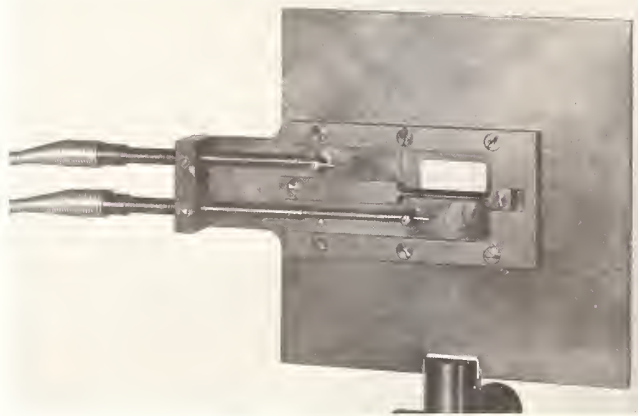
PLATE 7. NPL double-aperture device for linearity testing: detail of the side facing the detector system showing the mechanism and use of bevelling where possible.
