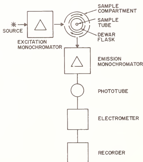
FIGURE 1. Block diagram of typical commercial analytical spectrofluorimeter with phosphoscope attachment.
