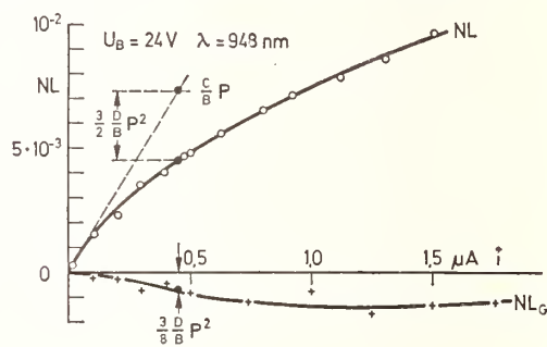
FIGURE 14. Jung's measurements of the nonlinearity of a silicon diode. NL for measurements by the dynamic method. NL_G for measurements with equalization of average current on the receptor. (Courtesy, Z. Angew. Physik.)
