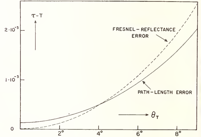
FIGURE 9. Maximal path-length error (for \tau_i = 0.37 and \theta_0 = 0.05 rad) and maximal Fresnel-reflectance error (for \tau_i = 1.00 and P polarization) versus tilt angle \theta_T , as computed from eqs (15) and (16) with n = 1.5 , n' = 1 .
