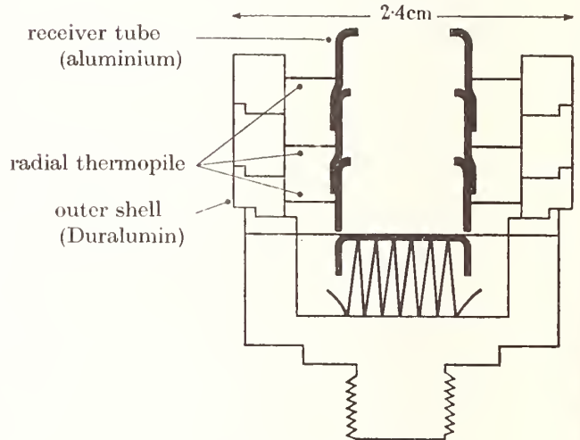
FIGURE 8. Gillham radiometer in a cavity [26].
