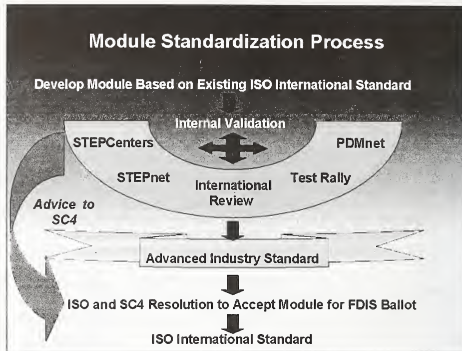
Figure 10-2: Modularization
