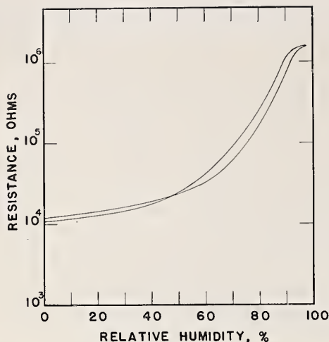
FIGURE 17. Calibration curve for a typical carbon film sensor at temperatures between 0° and 40° C.
