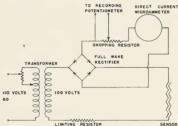
FIGURE 22. Alternating current measuring circuit.
