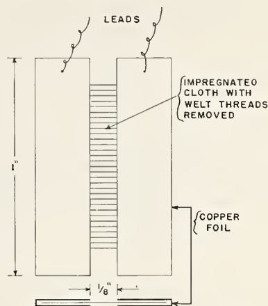
FIGURE 6. Ogden and Rees version of the Gregory hygrometer. Cotton fabric impregnated with one percent lithium chloride solution. Copper foil electrodes.
