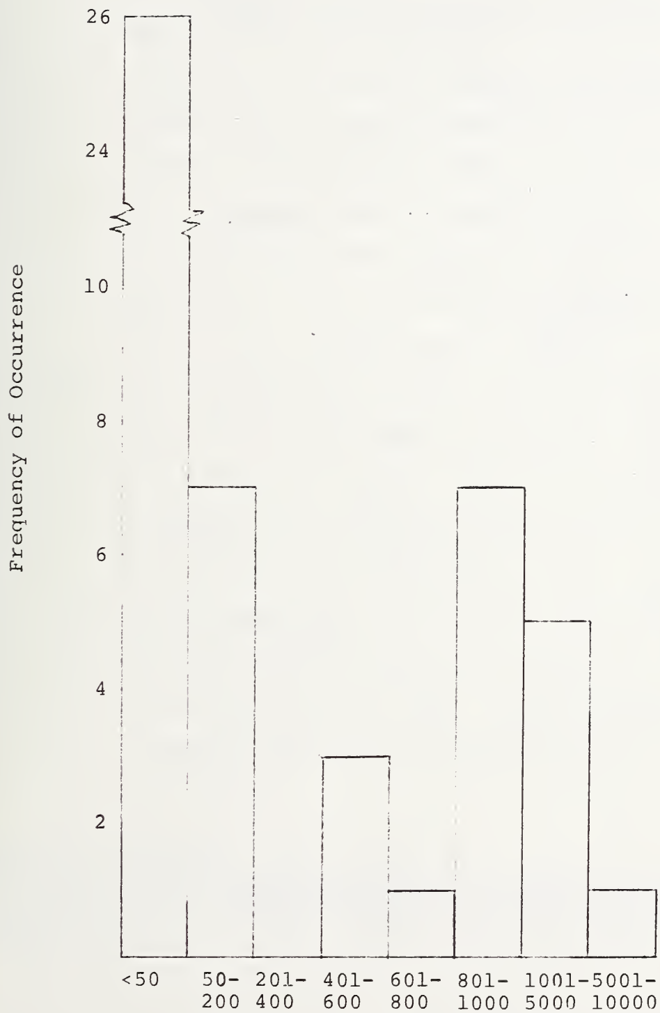
Figure A.2 Frequency of Collision Versus Dollar Damage to Building
