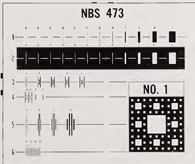
The next NBS photomask reference standard will be NBS 473, shown here. It will include calibrated linewidths as narrow as 0.5 micrometer (instead of 0.9 micrometer) and as wide as 30 micrometers (instead of 10 micrometers). The wider lines are used to calibrate oversized photomasks used in some facilities.
