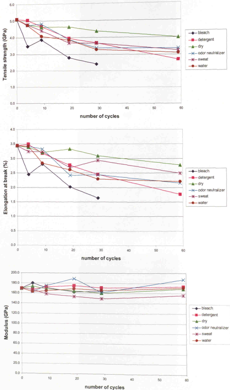
Figure 10: Evolution of the tensile strength, elongation at break, and modulus of PBO yarns as a function of artificial perspiration and cleaning chemical immersion. Standard uncertainty of these measurements is typically \pm 5\% .
