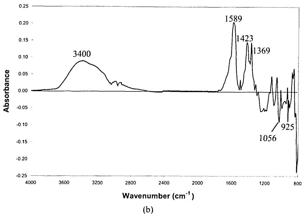
Figure 18: (a) Spectrum of unexposed PBO yarns, and (b) Difference spectrum of PBO yarns following 29 cycles of bleach solution exposure, referenced to spectrum of unexposed yarn.
