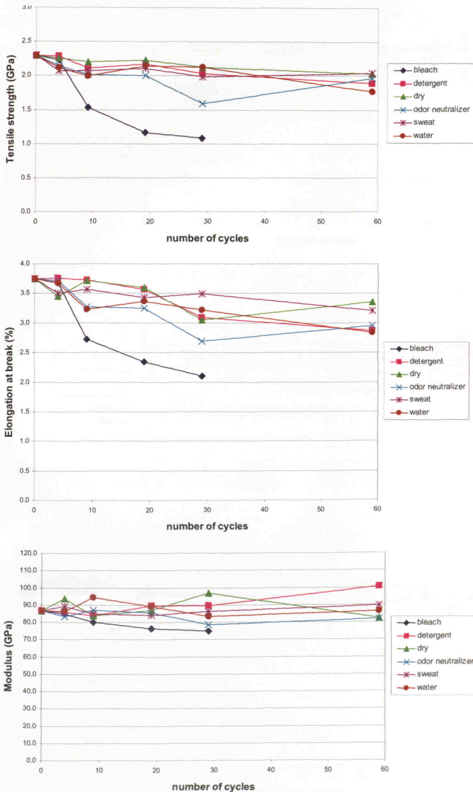
Figure 8: Evolution of the tensile strength, elongation at break, and modulus of yarns extracted from WRT aramid fabric as a function of artificial perspiration and cleaning chemical immersion. Standard uncertainty of these measurements is typically \pm 5\% .
