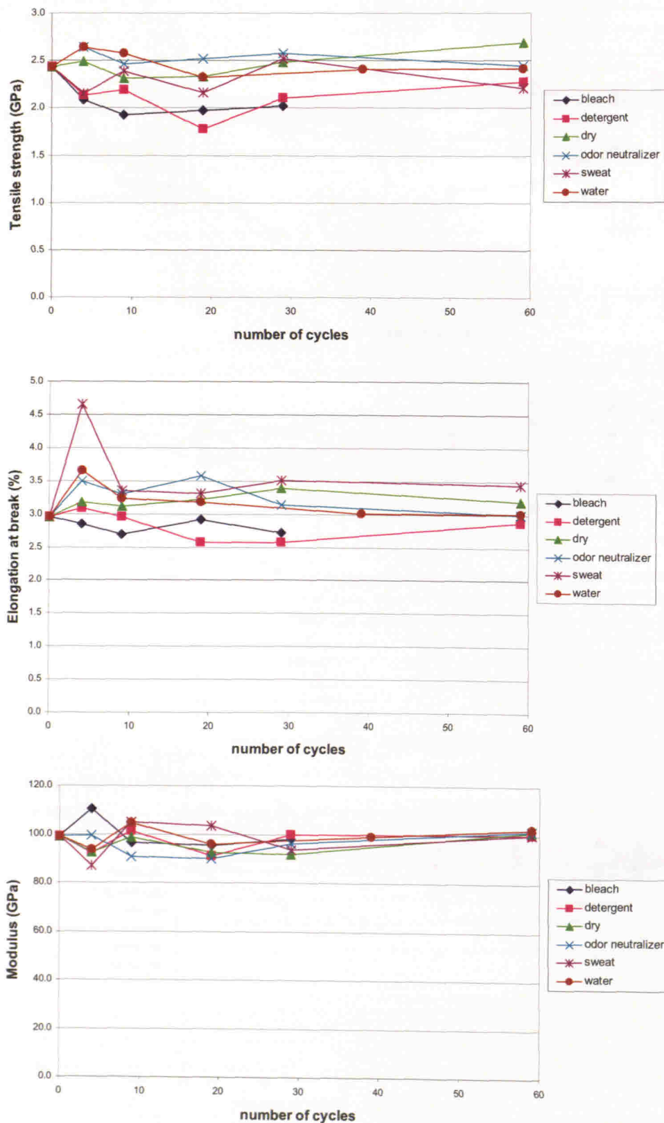
Figure 9: Evolution of the tensile strength, elongation at break, and modulus of UHMWPE yarns as a function of artificial perspiration and cleaning chemical immersion. Standard uncertainty of these measurements is typically \pm 5\% .
