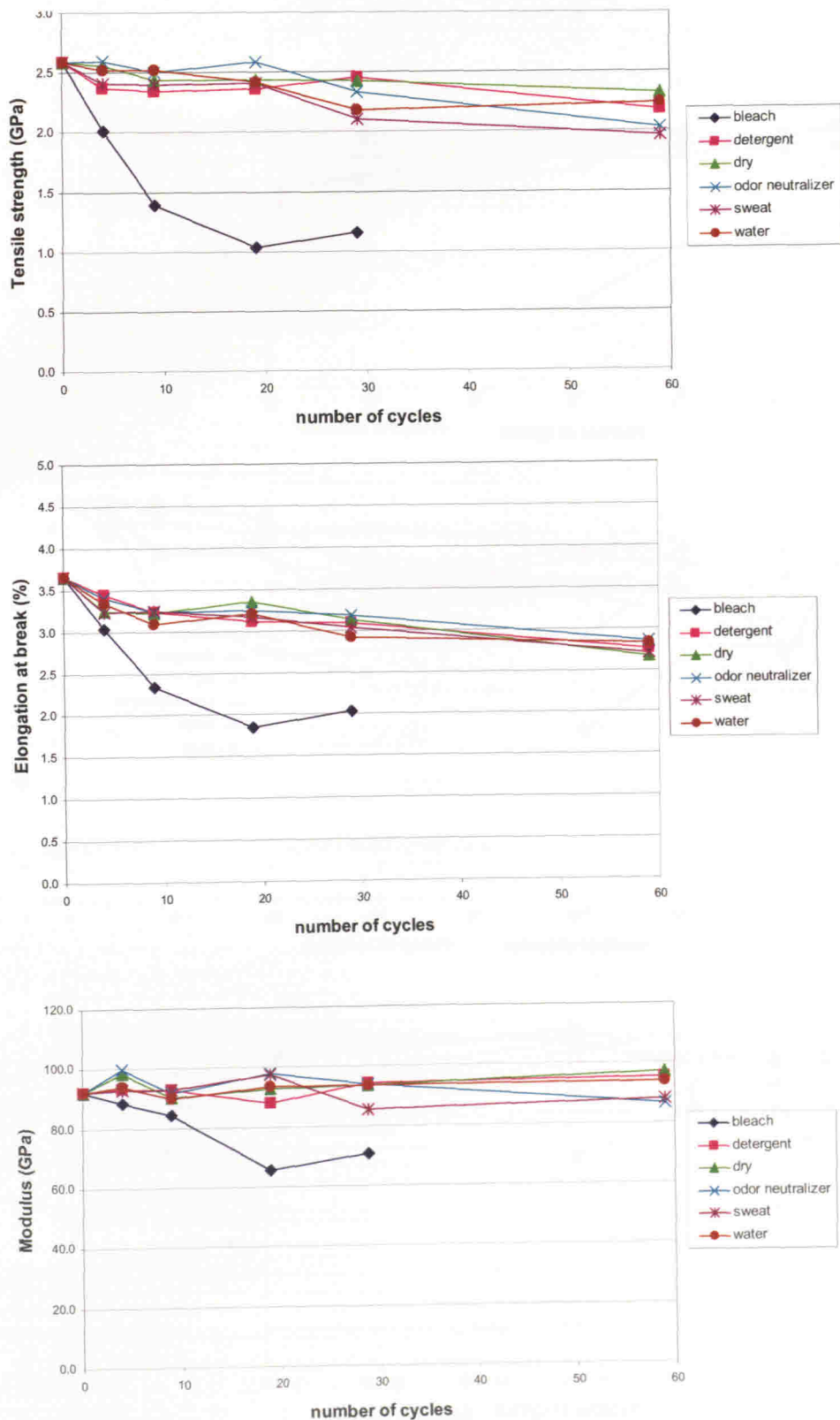
Figure 6: Evolution of the tensile strength, elongation at break, and modulus of aramid yarn as a function of artificial perspiration and cleaning chemical immersion. Standard uncertainty of these measurements is typically \pm 5\% .
