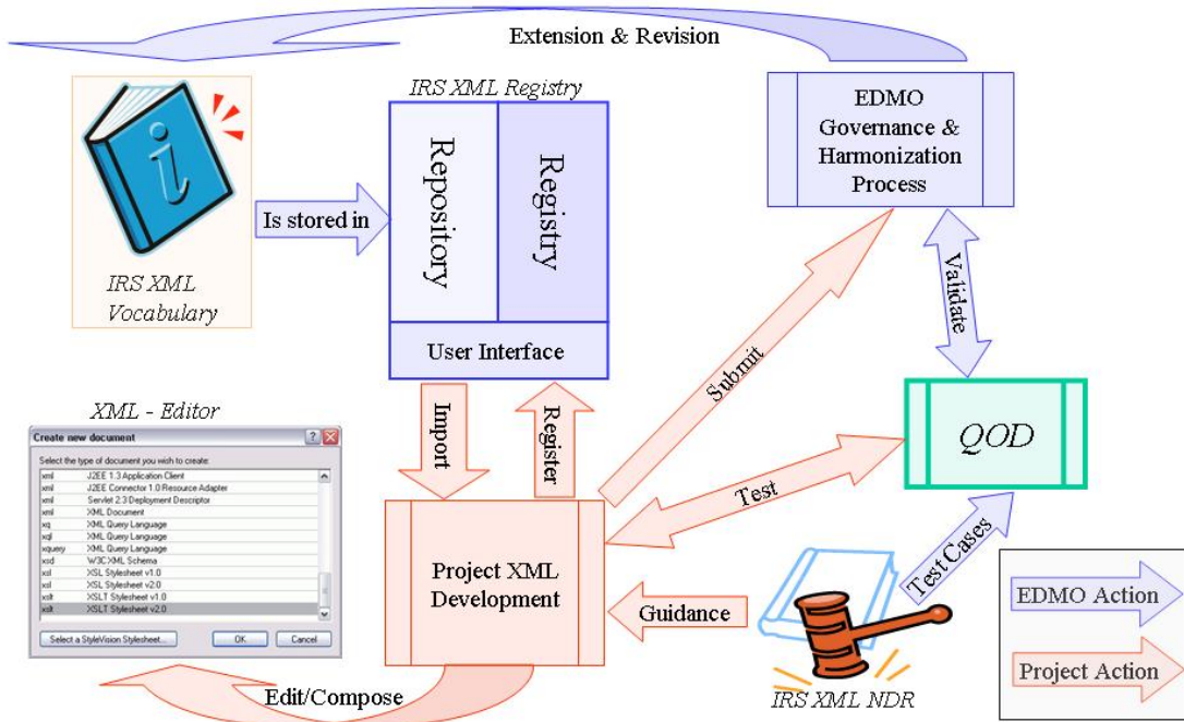
Figure 11: IRS XML Framework for Design 32
