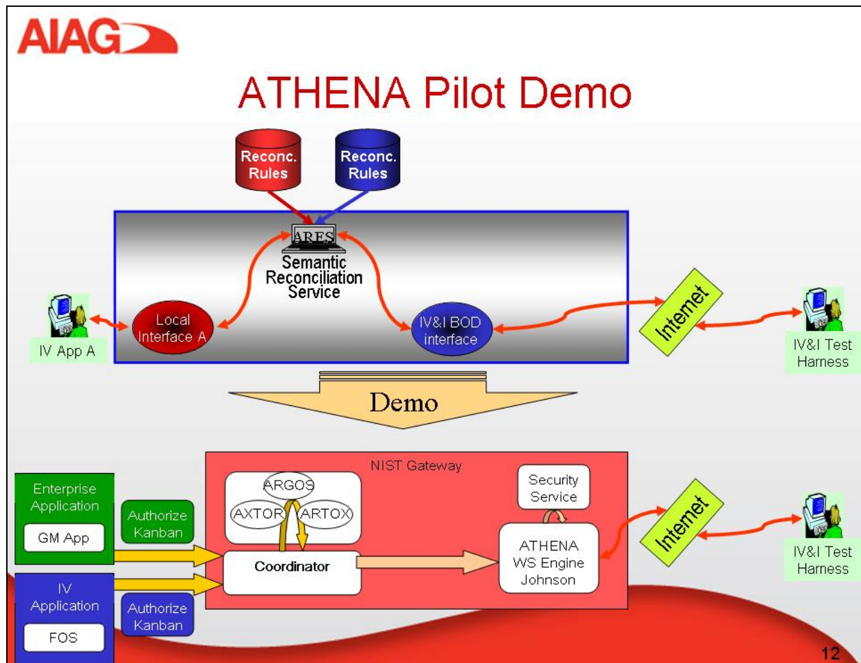
Figure 6: ATHENA Demonstration Pilot Using B2B Testbed 28
