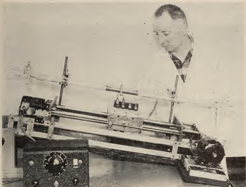
The automatic zone melter recently constructed at the Bureau provides a simple, inexpensive device for obtaining extremely high purity in semiconducting materials. It will also blend evenly, specific amounts of two metals to obtain a desired alloy.
