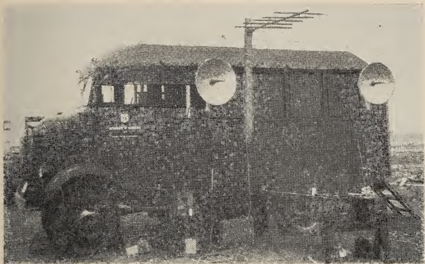
Control truck used to redetermine the speed of light by a radio-interferometer method (p. 107). The value of 299795.1 \pm 3.1 km/sec derived from these measurements is in close agreement with another value obtained independently by the molecular constants method (p. 107).
