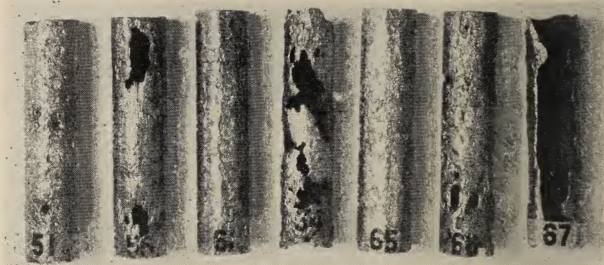
Results of an NBS study shows how some soils damaged unprotected steel pipe specimens during 14 years' exposure. Underground and other types of corrosion cost the United States billions of dollars annually (p. 70).
