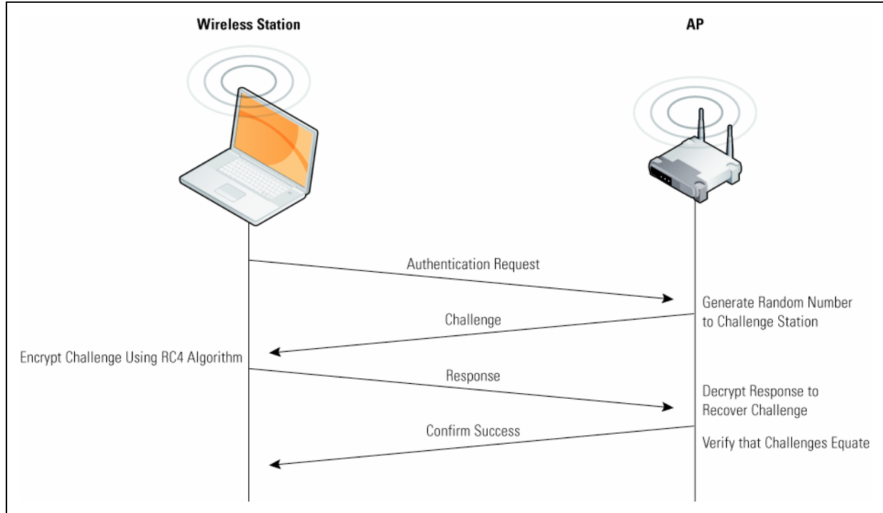
Figure 4-6. Shared Key Authentication Message Flow
