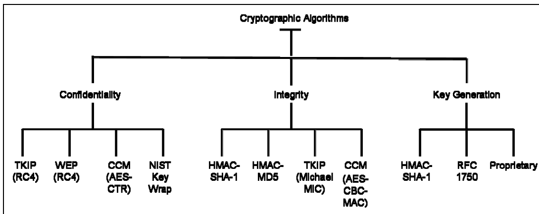
Figure 4-3. Cryptographic Algorithms Used in IEEE 802.11 26
