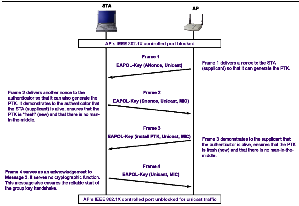
Figure 5-14. 4-Way Handshake
