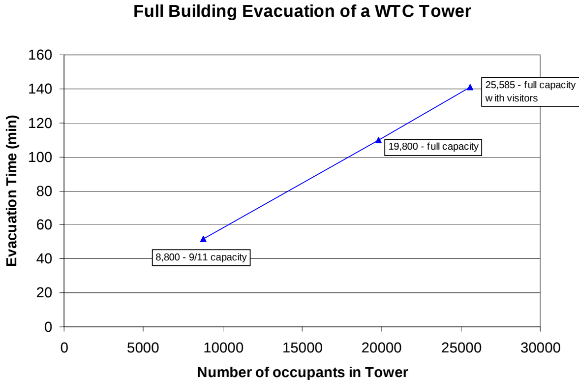
Figure 10–9. Simulation of full building evacuation of a WTC tower with different occupant loads.
