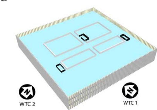
Floor 42 Stairs A and C transferred outside the core.
