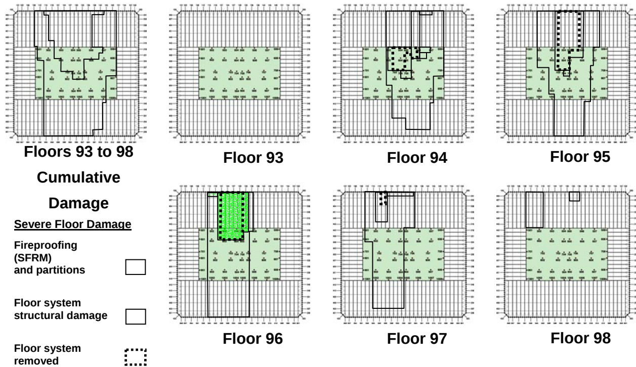
Figure 5-3. Calculated damage to floors 93 through 98 in WTC 1.
