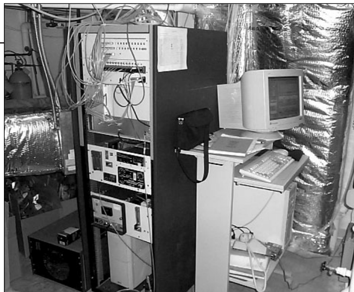
Automated tracer gas system for measuring building air change rates.
