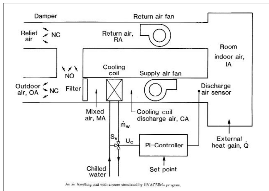
An air-handling unit with a room simulated by HVACSIM+ program.
