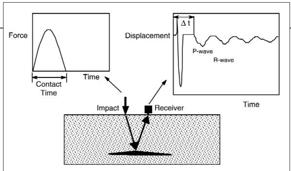
The impact-echo method: mechanical impact is used to generate stress waves and a receiver next to the impact point measures the resulting surface motion. Analysis of the measured surface motion permits detection of subsurface defect.
