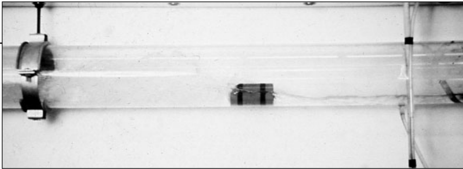
Horizontal solid waste drain transport for surge flow discharge
