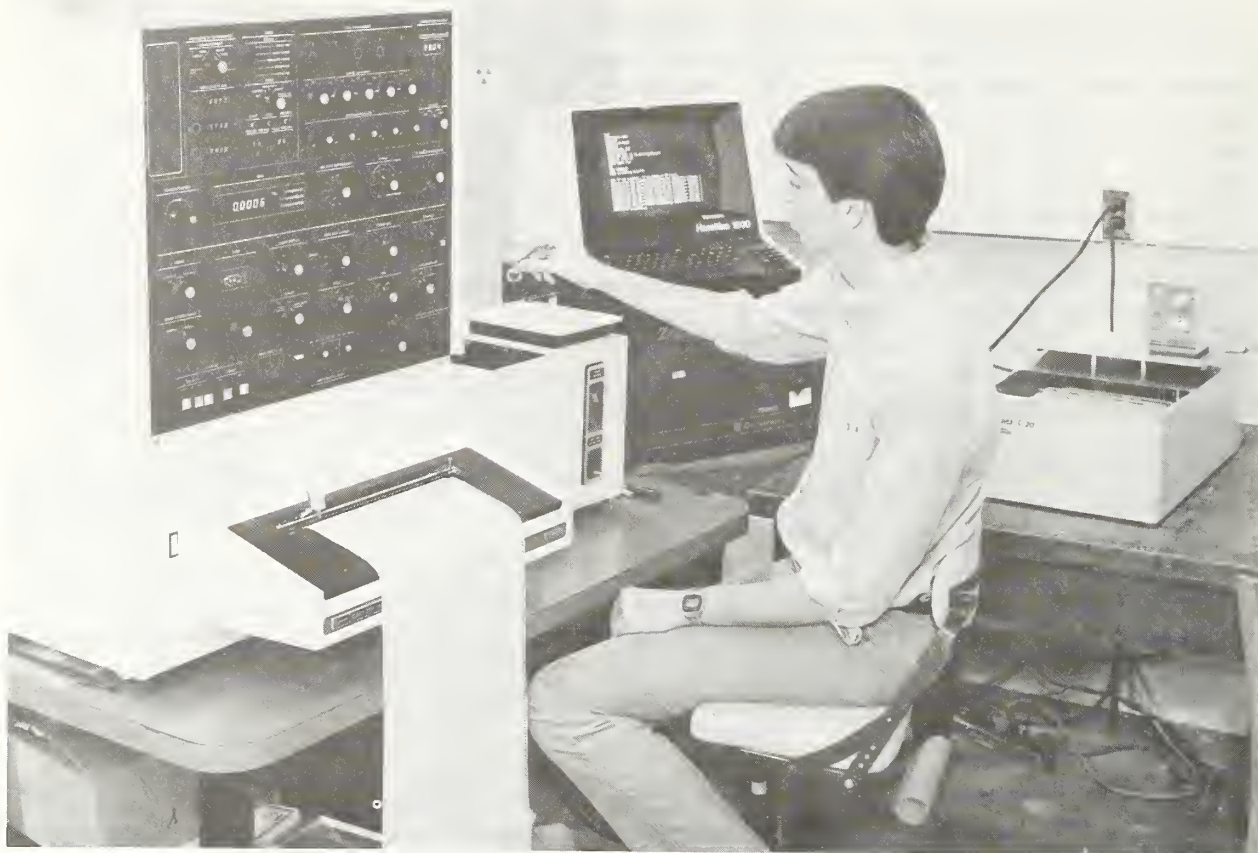
Figure 8. Spectrophotometry
