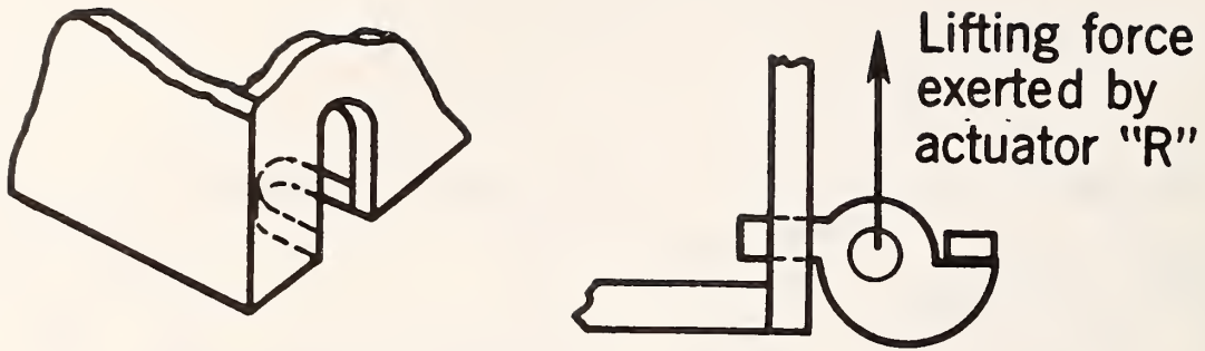
Figure 11. Detail of one of the two slots cut in the cube wall to engage the "R" lifting pawl needed for single actuator rotators (type B) of the cube.
