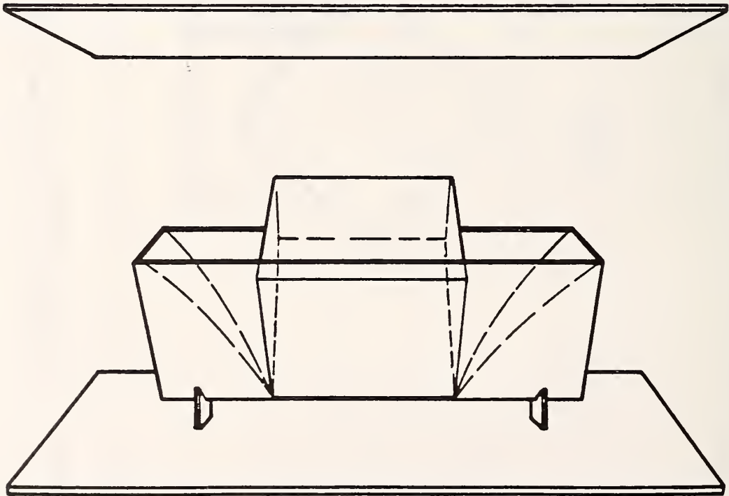
Figure 5. Two views of the dielectric positioner for use inside a TEM cell.
