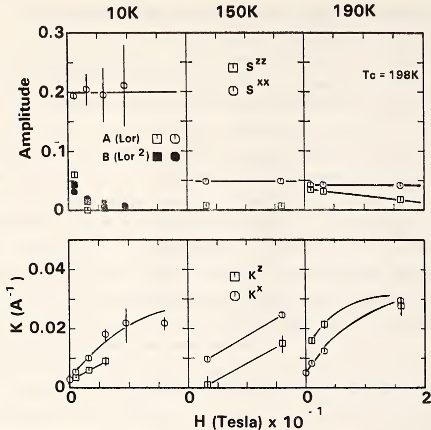
Figure 1. Parameters determined from the fits to the SANS data using the form of the scattering function in eqs (1) and (2) in the text.
