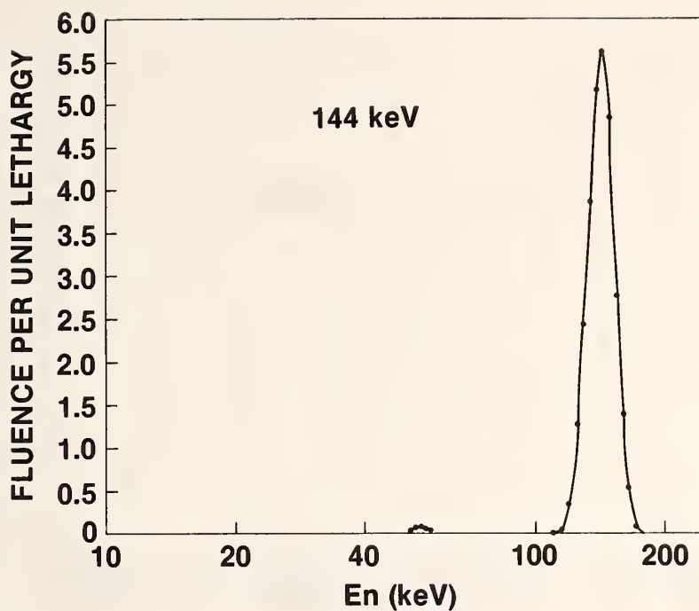
Figure 1. 144 keV Fluence spectrum
