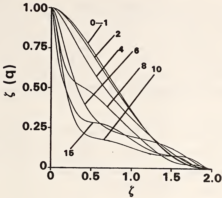
Figure 1. The function q(\xi) for several values of the phaseshift \nu .
