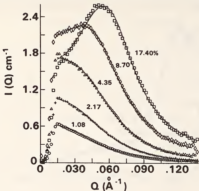
Figure 1. Differential scattering cross section, I(Q) , for various concentrations of BSA in 0.03 M k Acetate. Solid lines are computer-fitted spectra (see text).
