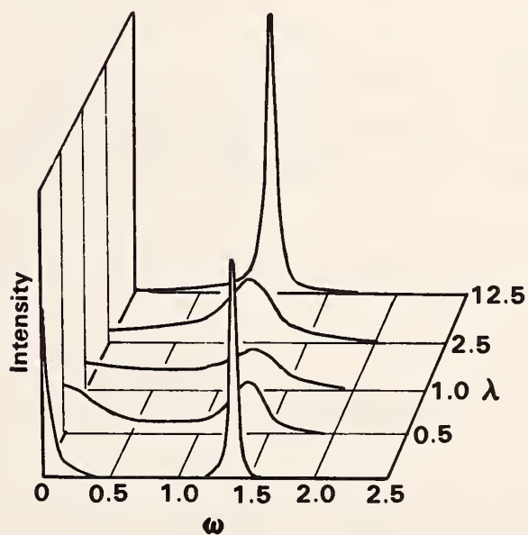
Figure 2. Neutron scattering intensity obtained from (4).
