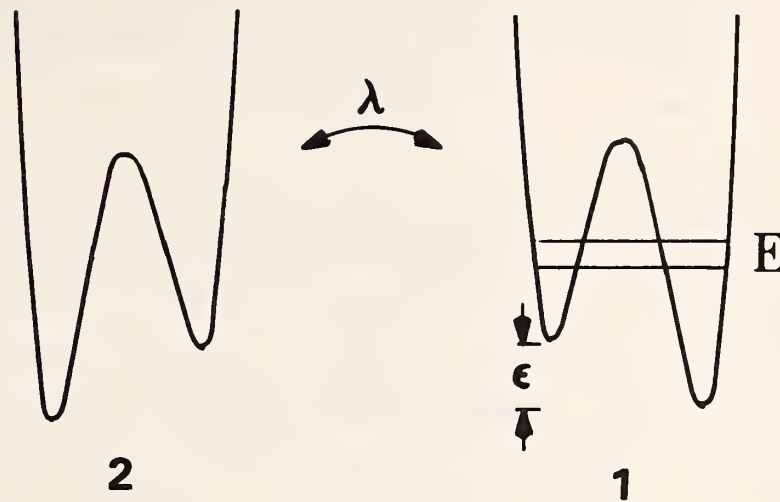
Figure 1. Stochastic states, /1/ and /2/, representing neighboring self-trapped configurations of a double-well defect vibrational potential. The model assumes random potential well flips at a rate \lambda .
