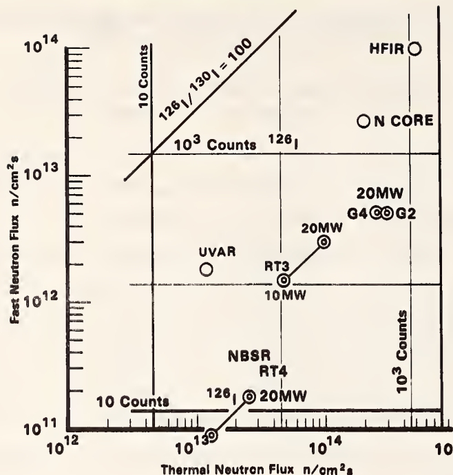
Figure 1. All double circles are NBS Reactor; single circles are other reactors. UVAR - University of Virginia Reactor N - Hanford N reactor, core position HFIR - High Flux Isotope Reactor, ORNL Conditions of calculation are: 10^8 atoms ^{129}\text{I} , 1 \mu\text{g} ^{127}\text{I} , 12 hour irradiation, 6 hour delay, 16 hour count, and \epsilon=0.03 count/disintegration.
