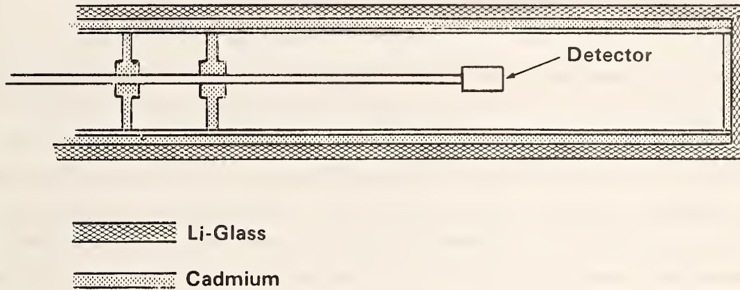
Figure 1. Assembly sketch of Neutron Driven Gamma-Ray Source (NDGS). The assembly as shown is placed in the NBSR thermal column cavity.
