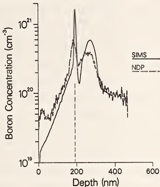
Figure 3. SIMS (solid line) and NDP (dashed line) data for the annealed sample normalized to a total B concentration of 8.4 \times 10^{15} \text{ cm}^{-2} .
