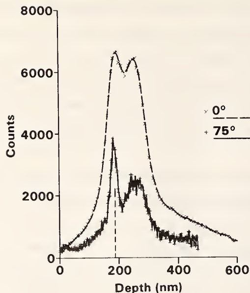
Figure 2. Neutron depth profiles of the sample from figure 1 measured after annealing at 1000°C for 30 minutes in dry nitrogen. The upper dashed curves (x) was recorded for normal emergence ( \theta=0^\circ ) and the lower solid curve (+) for grazing emergence ( \theta=75^\circ ) of the alpha particles.
