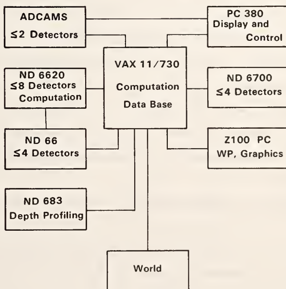
Figure 1. Nuclear Methods Group data acquisition and computation system.
