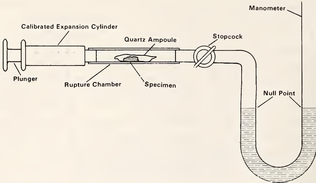
Figure 4. Pressure measurement system.
