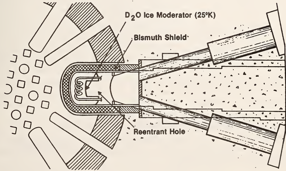
Figure 2. Cold neutron source.
