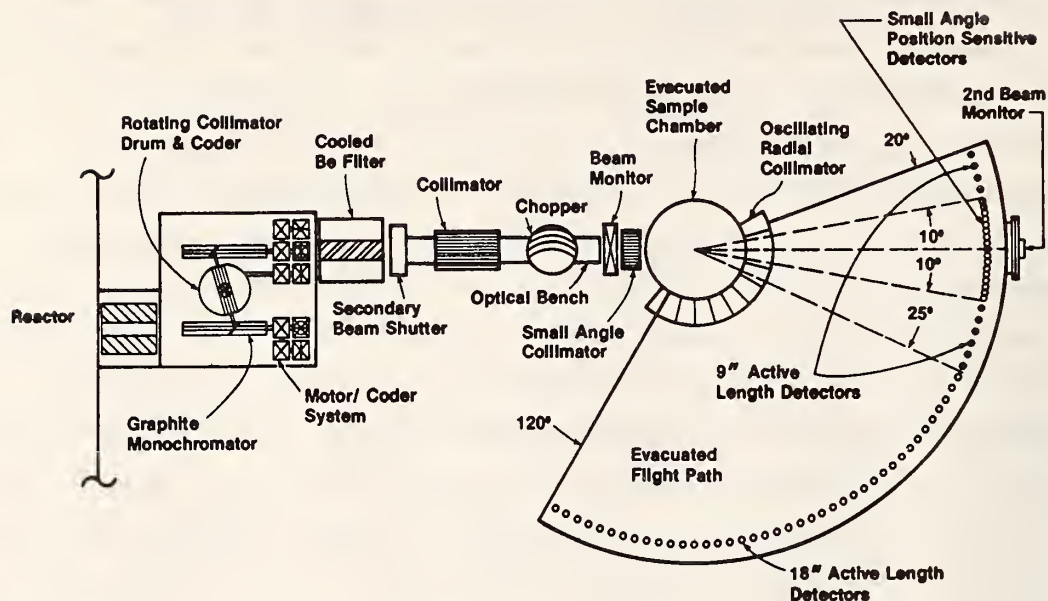
Figure 1. The NBS neutron time-of-flight spectrometer.
