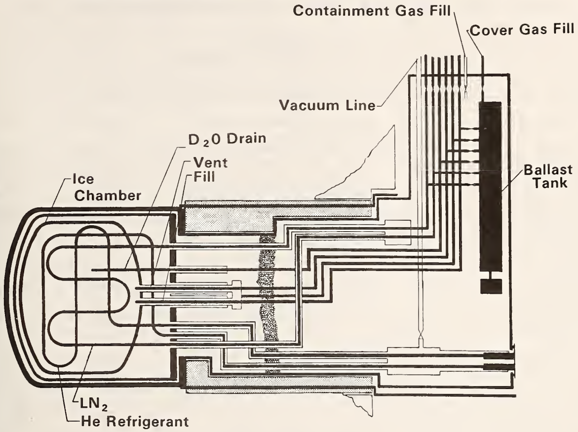
Figure 1. Schematic illustration of cold source facility.
