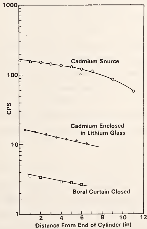
Figure 2. Fission rate transverses taken along the axis of the axis of the NDGS with a U-238 fission chamber.
