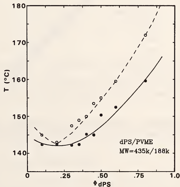
Figure 1. Phase diagram of d PS/PVME blend with MW=435k/188k. Solid circles and open circles are cloud points and spinodal points respectively.
