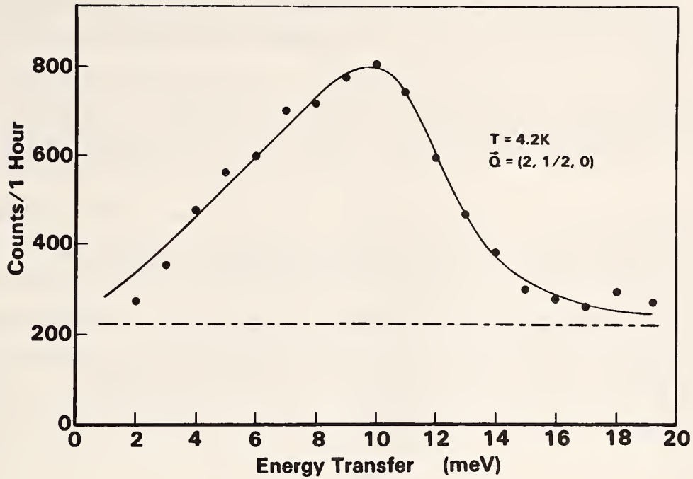
Figure 1. The spectrum of inelastic neutron scattering in \text{Dc}_{0.35}\text{Mn}_{0.65}\text{Te} at 4.2 for \vec{Q} = (2\pi/a)(2, 1/2, 0) . The solid curve is the best fit of the theoretical spectrum (corrected for instrumental resolution), corresponding to J_{\text{NN}} = 12.8\text{K} . The dashed line is the background.
