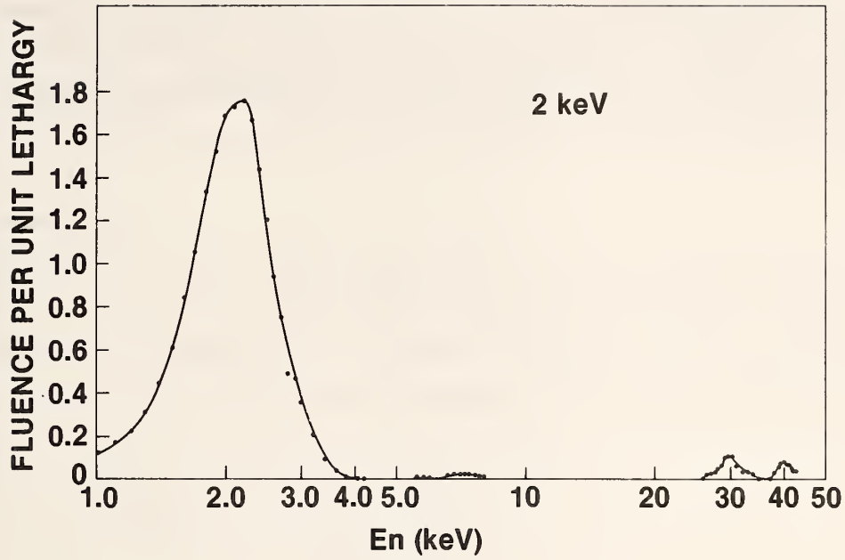
Figure 5. 2 keV Fluence spectrum
