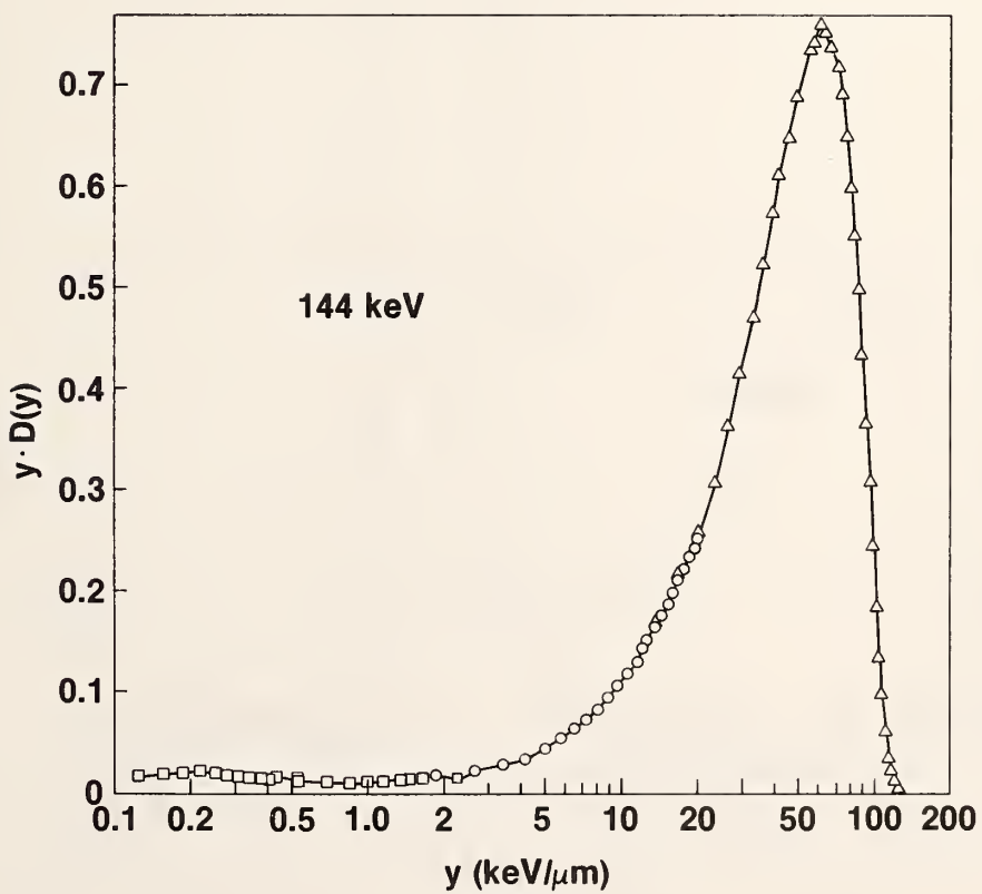
Figure 2. 144 keV Microdosimetric spectrum
