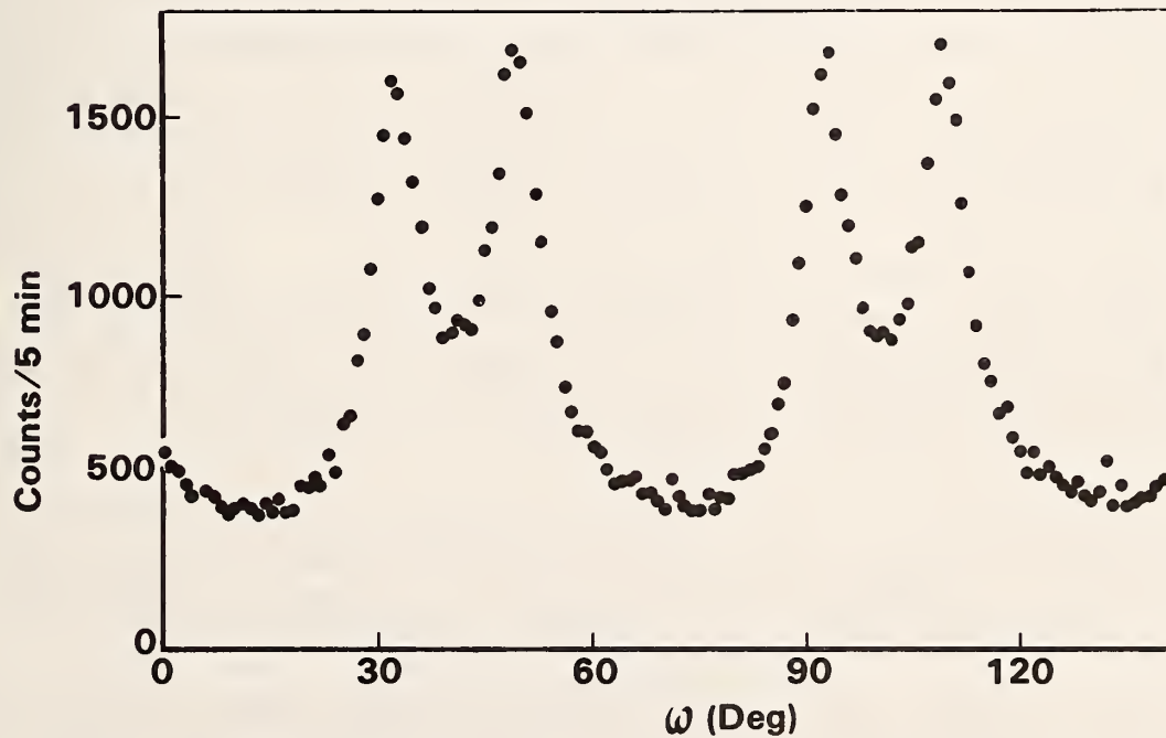
Figure 2. Extended \omega -scan in \text{Zn}_{0.45}\text{Mn}_{0.55}\text{Se} showing several diffuse magnetic peaks at symmetry equivalent positions.
