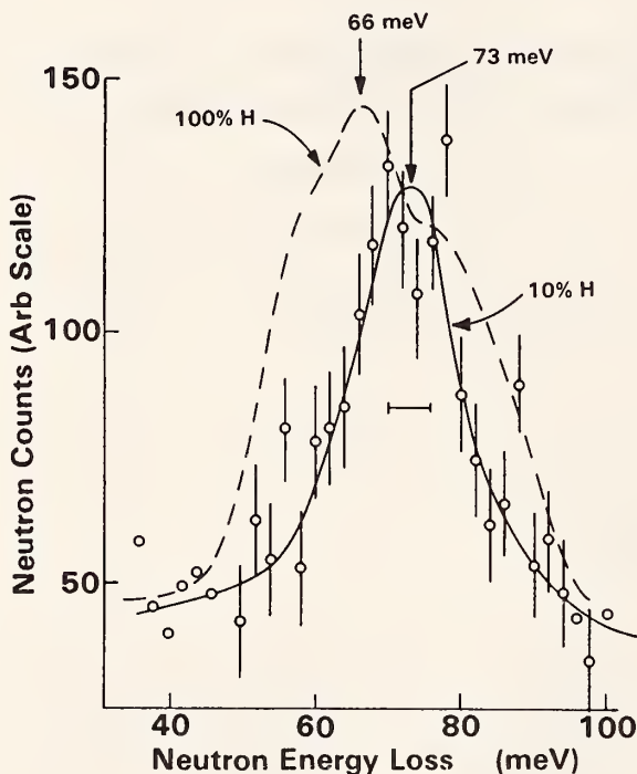
Figure 1. Neutron energy loss spectra between 34 and 100 meV at 80° K for a saturation coverage of H isotopes on cleaned Pt block. Results for 100% H are shown by the dashed lines. The energy resolution (FWHM) is indicated by the horizontal bar.
