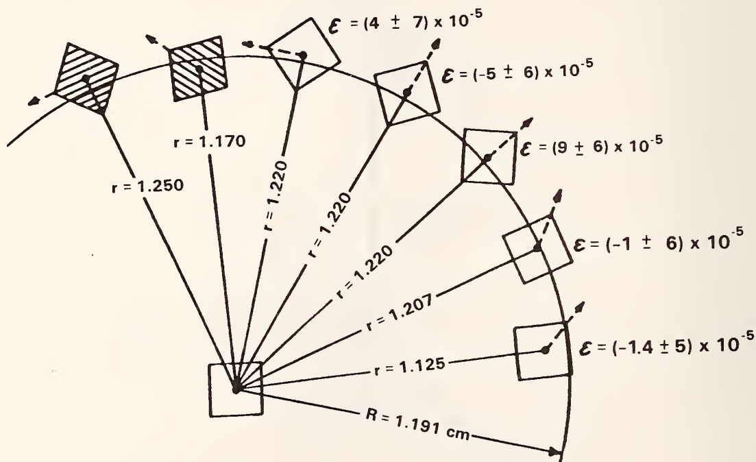
Figure 3. Cross-sections of \Delta V , drawn to scale relative to the sample cross-section, for copper powder (open squares) and production-type DU (cross-hatched parallelograms) near-surface measurements. The arrows indicate the \vec{k} -direction for each measurement. Measured strains, \epsilon , are shown for the copper powder.
