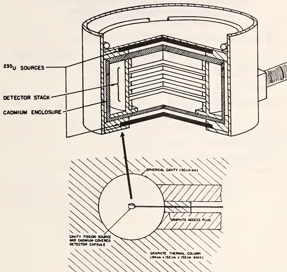
Figure 1. The NBS Cavity Fission Source
