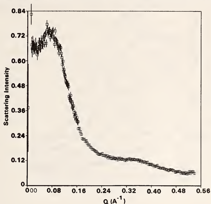
Figure 1. Small angle neutron scattering pattern from a cured epoxy. The multi-peaked structure in the pattern is due to the formation of a semi-regular network of chemical crosslinks. For the measurement the crosslinking agent was deuterated to enhance scattering contrast with the matrix.
