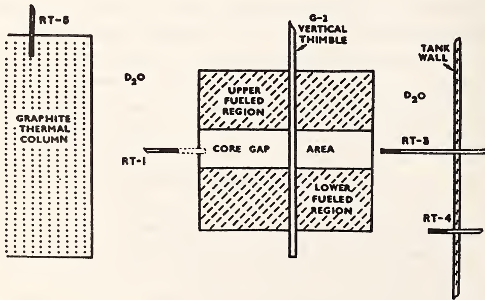
Figure 1. NBSR irradiation facilities at 20 MW.
