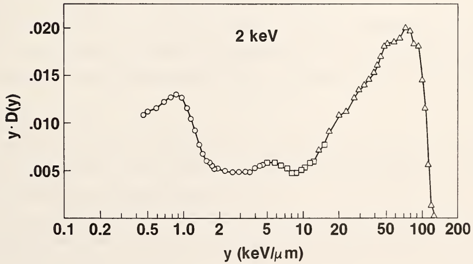
Figure 6. 2 keV Microdosimetric spectrum
