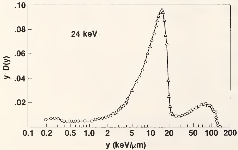
Figure 4. 24 keV Microdosimetric spectrum
