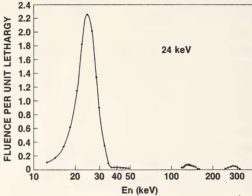
Figure 3. 24 keV Fluence spectrum
