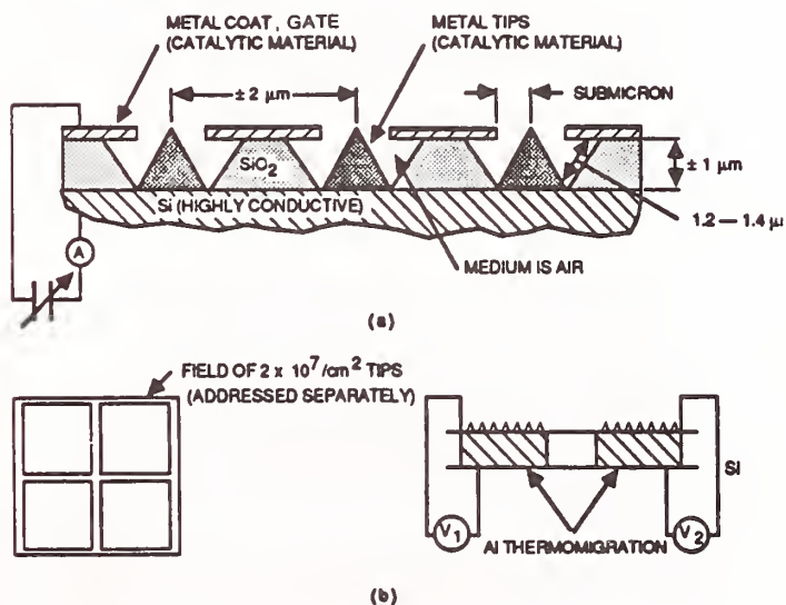
Fig. 2 Submicron gas sensor
