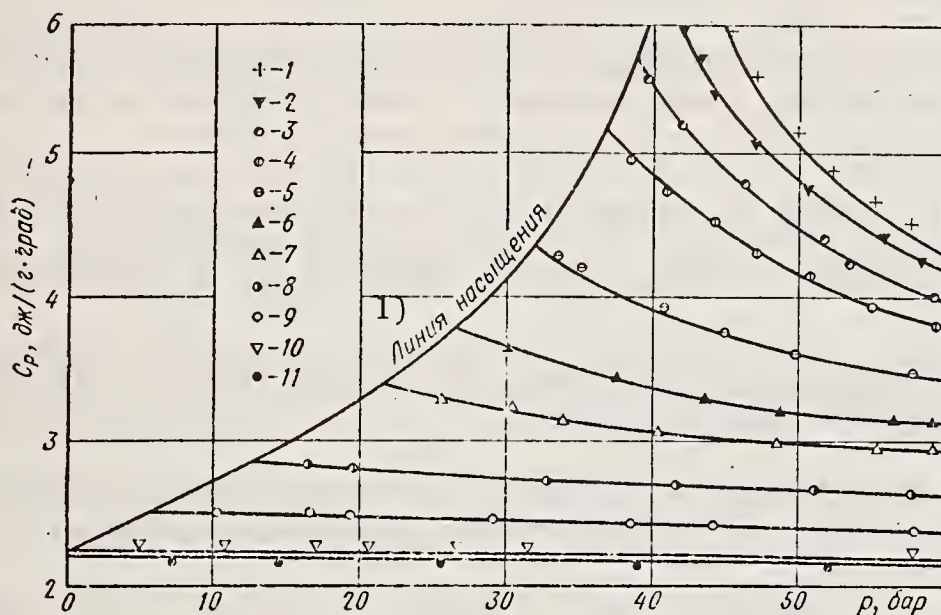
Figure 13. Experimental data on isobaric heat capacity of liquid propylene at T equal to: 1 -- 360.35; 2 -- 358.65; 3 -- 355.15; 4 -- 352.55; 5 -- 344.64; 6 -- 335.15; 7 -- 325.65; 8 -- 301.65; 9 -- 274.57; 10 -- 197.55; 11 -- 164.65°K.
