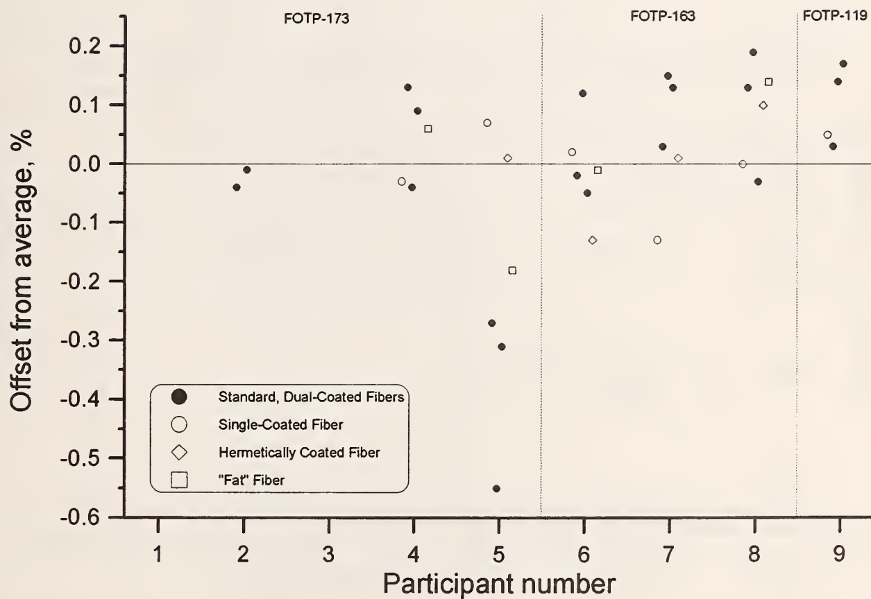
Figure 9. Offsets of participants' fiber coating outer layer noncircularity measurements from average values. Up to six points plotted, for each participant, represent the six fibers in the measurement sample. Filled symbols denote standard 250 \mu\text{m} dual-coated fibers. Open symbols denote non-standard fibers: single-coated, hermetically coated, and "fat" (nominally 500 \mu\text{m} ). Participants are grouped according to their measurement methods, identified by TIA Fiber Optic Test Procedure (FOTP) numbers.
