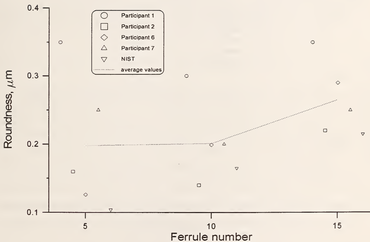
Figure 22. Ferrule roundness measurements on three ferrule specimens. Dotted line connects average values.
