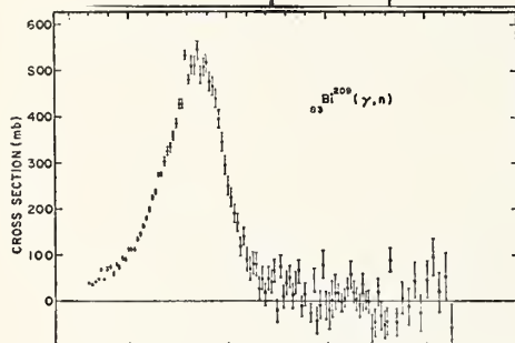
FIG. 4. Top figure shows data points for \sigma[(\gamma, n) + (\gamma, np)] for Bi^{209} , obtained from single-neutron counting data. Center figure shows data for \sigma(\gamma, 2n) obtained from double-neutron counting data. Data points for the compound nucleus formation cross section of Bi^{209} , i.e., \sigma[(\gamma, n) + (\gamma, np)] + \sigma(\gamma, 2n) are shown in the bottom figure. Solid curve is a plot of a Lorentz line having the parameters given in Table II. The data are uncertain below 8 MeV owing to low beam intensities encountered.
