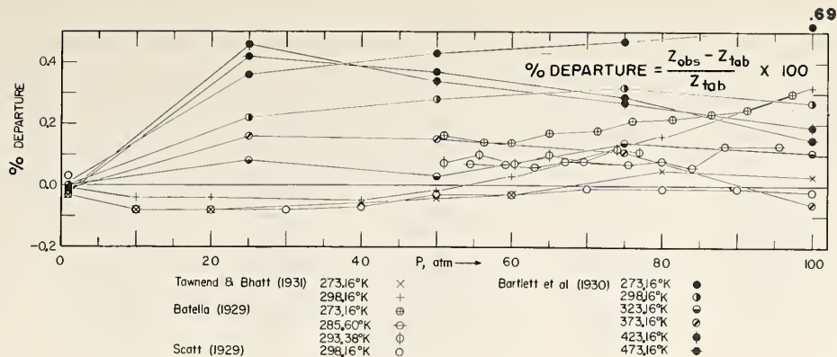
Figure 5a. Departures of experimental compressibility factors from the the tabulated values for carbon monoxide (table 5-1)
