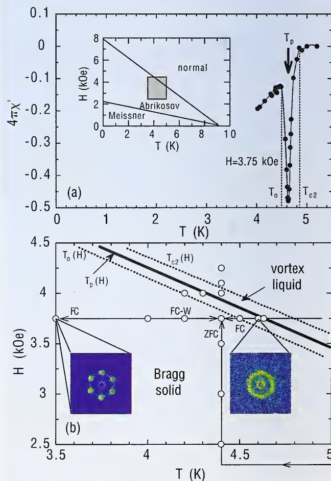
FIGURE 1. Peak effect and (H-T) phase diagram of Nb. a) ac magnetic susceptibility for H_{ac} = 3.75 kOe (field-cooled). H_{ac} = 3.3 Oe and 1 kHz. Inset: global H - T phase diagram for the Nb crystal used in this study. (b) Expanded view of the H - T phase diagram (shaded box in a). Two observed SANS images of the field-cooled vortex states are shown.
