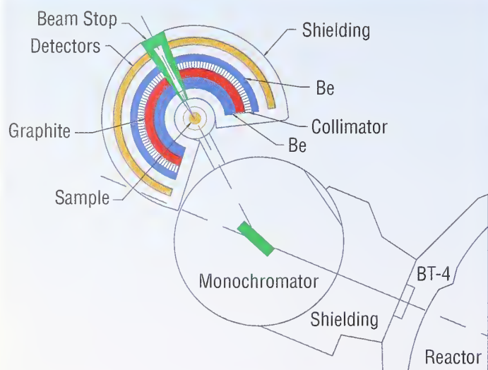
FIGURE 1. Schematic diagram of the final configuration of FANS. Presently installed phase I includes the filters to the right of the beam.
