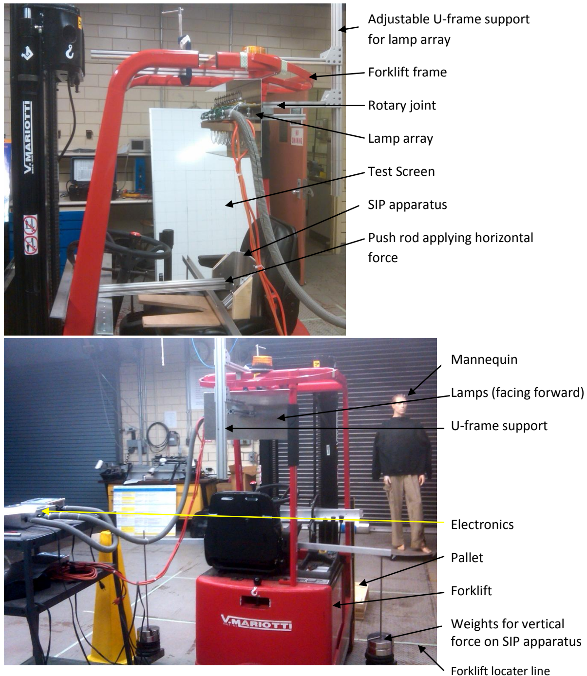
Figure 7 – Experimental setup showing all components.
