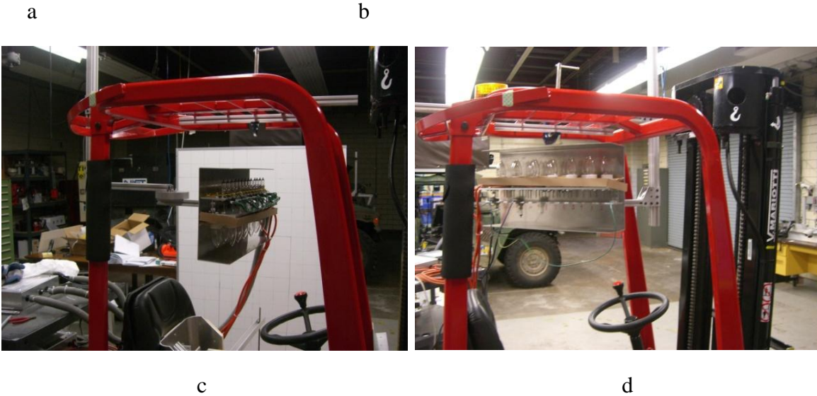
Figure 19. (a) Top view of lamps test angles as specified by ISO/DIS 13564-1, (b) Lamps rotary joint, (c) Lamps facing forward, (d) Lamps facing to the rear of the forklift.
