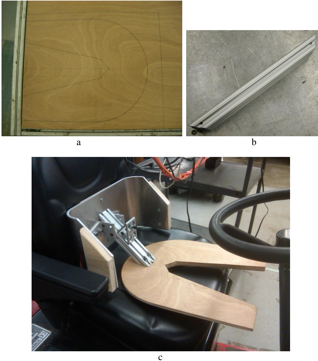
Figure 17. (a) SIP Apparatus: (a) base drawn on a piece of wood (b) joining bar for base to back, (c) fully assembled apparatus on a forklift seat.
