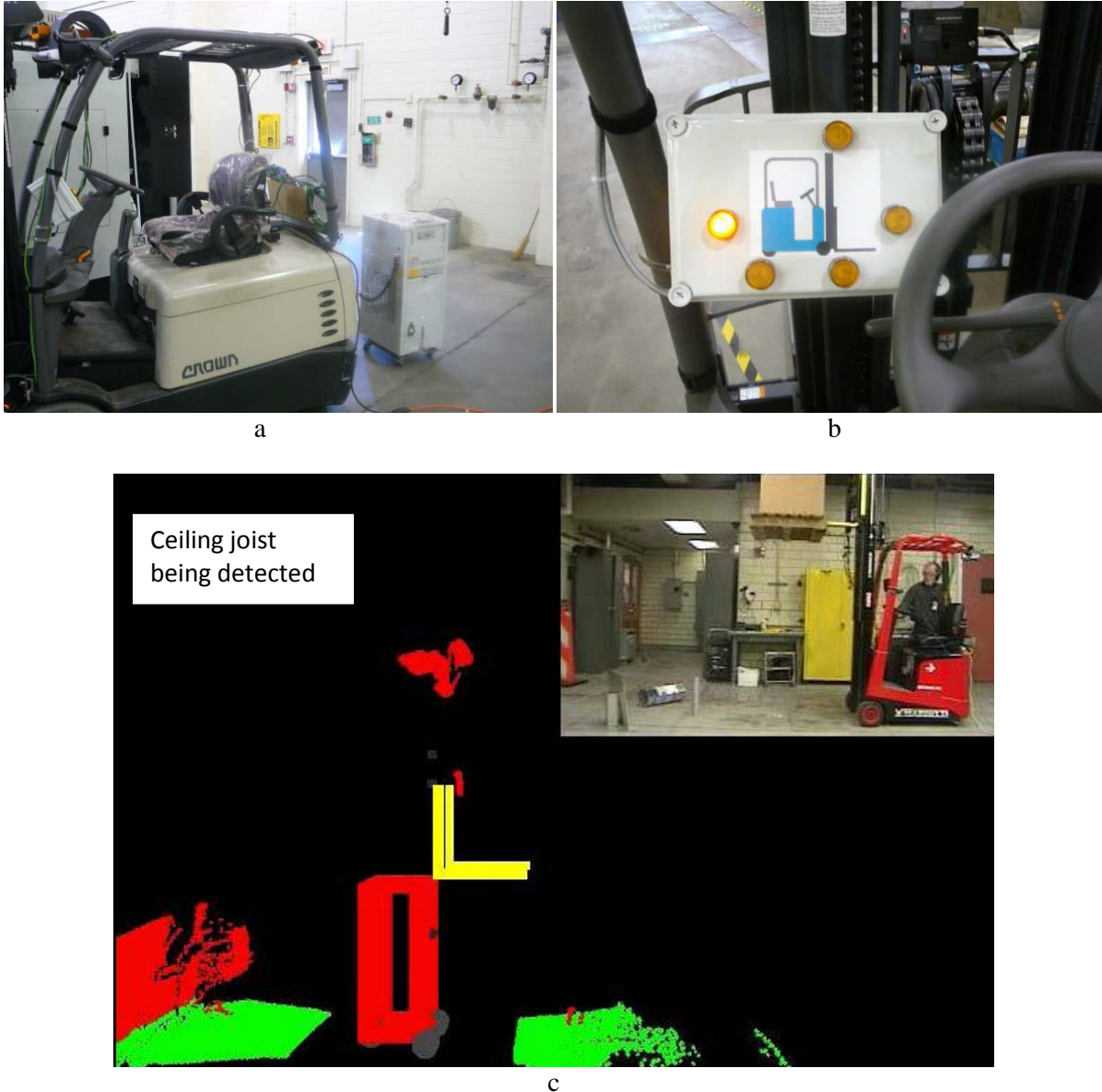
Figure 21. 3D imagers mounted on a forklift and integrated with simple operator alerts – (a) obstacle is behind the forklift and (b) the alert indicates the obstacle, (c) high lift obstacle detect sensor mounted to forks frame (upper right photo) capturing data of ceiling joists (lower left).
