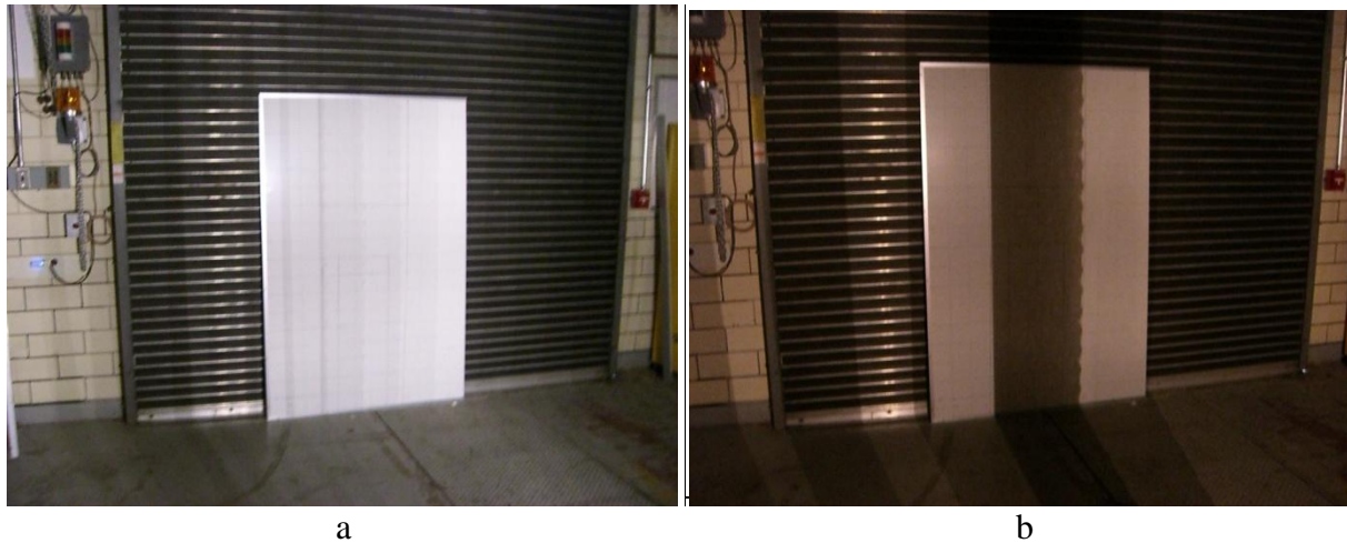
Figure 9. (a) Shadows of test1, (b) Shadow of test 1 with just two lamps separated by 75 mm turned on
