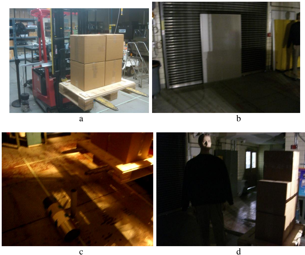
Figure 15. (a) Forklift carrying a pallet of boxes for visibility tests with resulting shadows shown on: (b) the test body, (c) ANSI/ITSDF B56.5 standard test pieces, and (d) a mannequin.
