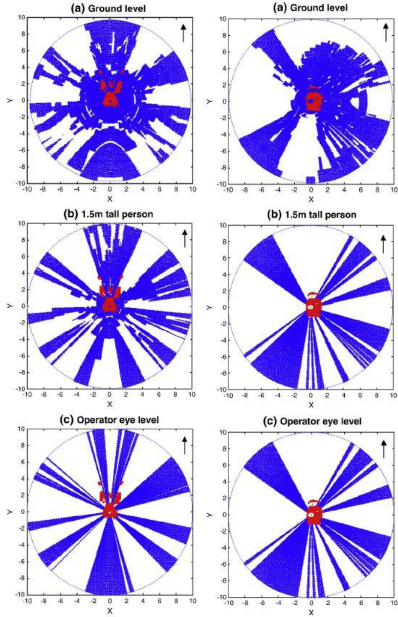
Figure 22. GaTech automatic detection of blind spots for construction dozer (left column) and pickup truck (right column) [12]
