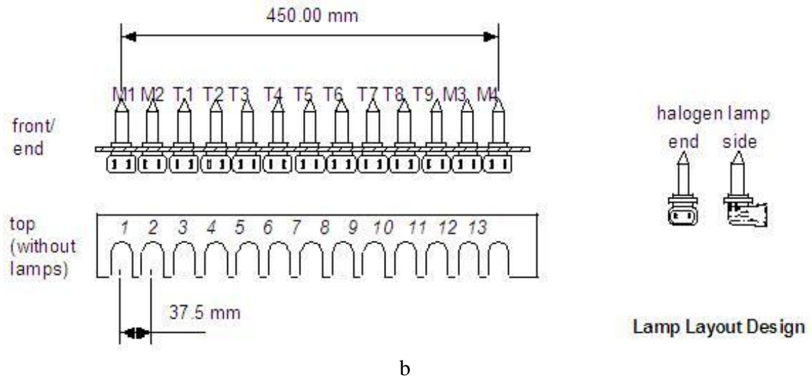
Figure 2. (a) Light source arrays, including: halogen (top row) and incandescent (bottom row); (b) Halogen lamp layout design.
