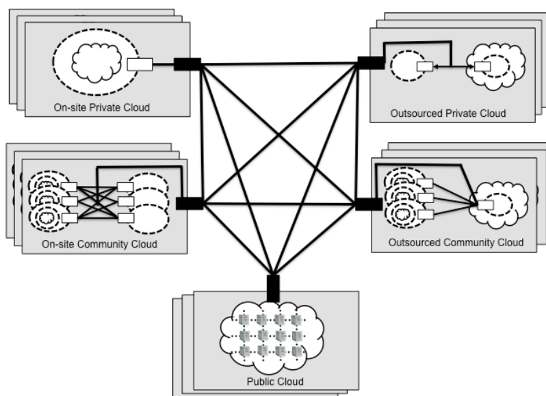
Figure 7: Hybrid Cloud
