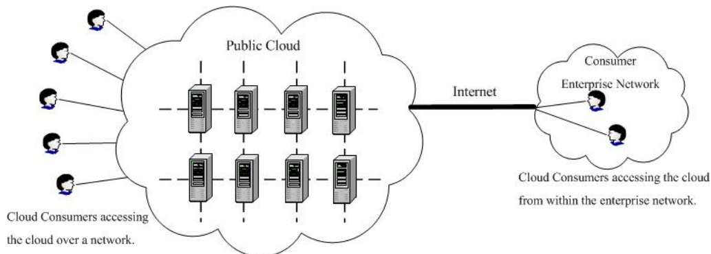
Figure 6: Public Cloud
