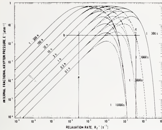
Fig. 4. Test line and example of test range for radioisotope method. Reject leak size of 5 \times 10^{-8} atm·cm 3 /s of air with V = 0.01 cm 3 , P_{E^*} = 5 atm of Kr-N 2 mixture, S = 200 \mu Ci/atm·cm 3 , K = 10^4 min -1 · \mu Ci -1 , and a minimum detectable count rate of 2500 min -1 for a signal-to-noise ratio of 5. Line (a) represents R_r^* of 2.94 \times 10^{-6} s -1 for Kr 85 , R^*/(P_0 V P_{E^*} S K) = E^* = 2.5 \times 10^{-2} atm -1 is test line (b). The intersection of (a) and (b) sets T = 2.4 h. At the intersection of (b) and the t = 1000 s, line (c) represents R_r^* = 3.7 \times 10^{-3} s -1 which leads to L_{air} = 6.3 \times 10^{-5} atm·cm 3 /s.
