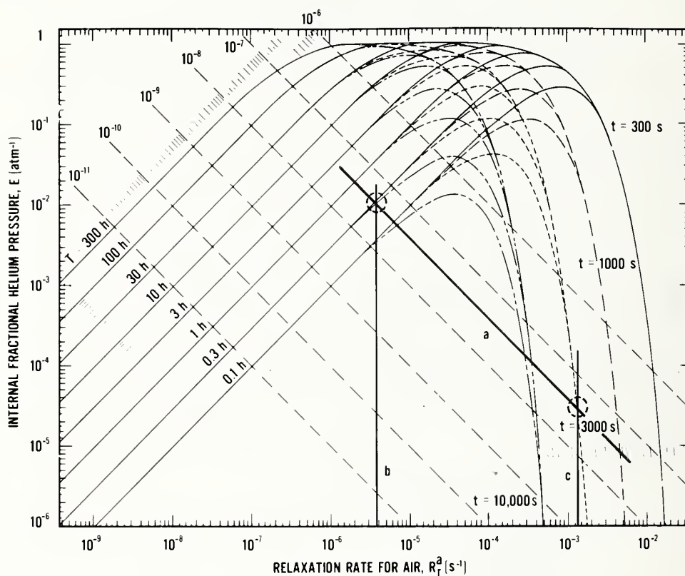
Figure 2. The graphical procedure for determining leak size with the helium test method from the leak detector indicated response for given conditions of P_E , T , t , and V . See example 1 of Section II. a - test line. b - first solution for R_r^a and hence the smaller possible value for L_a . c - second solution for R_r^a and hence the larger possible value for L_a .
