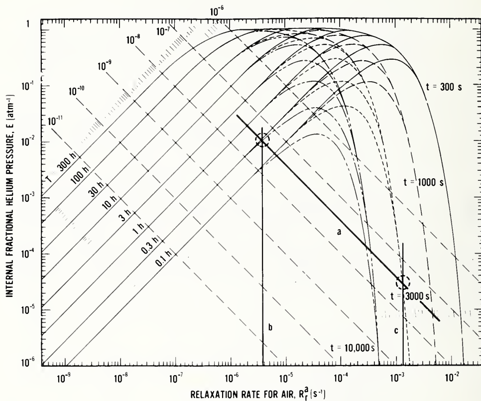
Figure 2. The graphical procedure for determining leak size with the helium test method from the leak detector indicated response for given conditions of P_E , T , t , and V . See example 1 of Section II. a - test line. b - first solution for R_r^a and hence the smaller possible value for L_a . c - second solution for R_r^a and hence the larger possible value for L_a .
