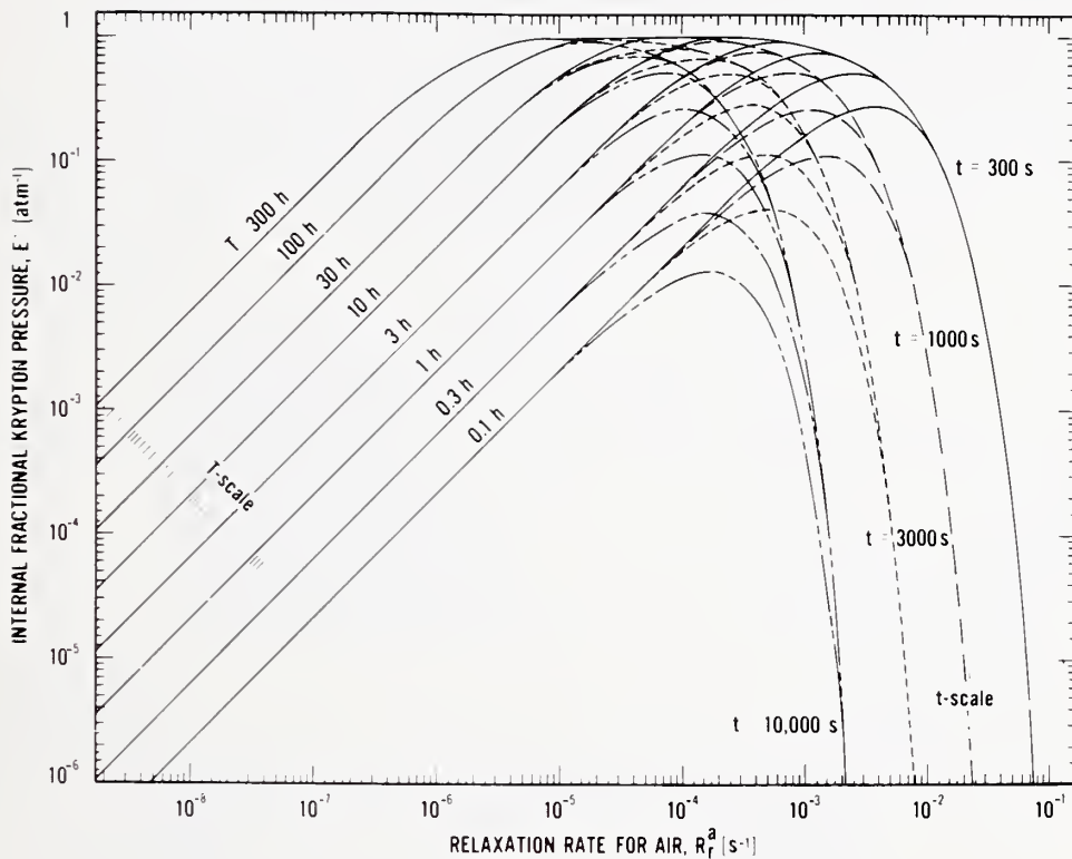
Figure 3. Characteristics for the krypton-85 radioisotope method. E^* , the relative partial pressure of krypton within the package per atmosphere of external krypton pressurization, as a function of the relaxation rate for air R_r^a with pressurization time T and dwell time t as parameters. Tick marks include those at 1.25, 1.5, 1.75, and 2.5 with the remainder at integral values for each decade on the axes, for T , and for t . Test lines are not included since these are easily constructed as horizontal lines at values for E^* = \text{const.} Use master graph 2 for photocopying.
