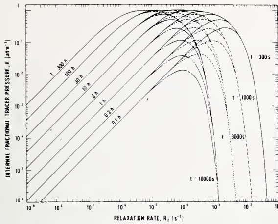
Fig. 1. E , the relative partial pressure of tracer gas within package interior free volume per atmosphere of external tracer gas pressurization, as function of relaxation rate R_r with pressurization time T and dwell time t as parameters. Transport mechanism is molecular flow.
