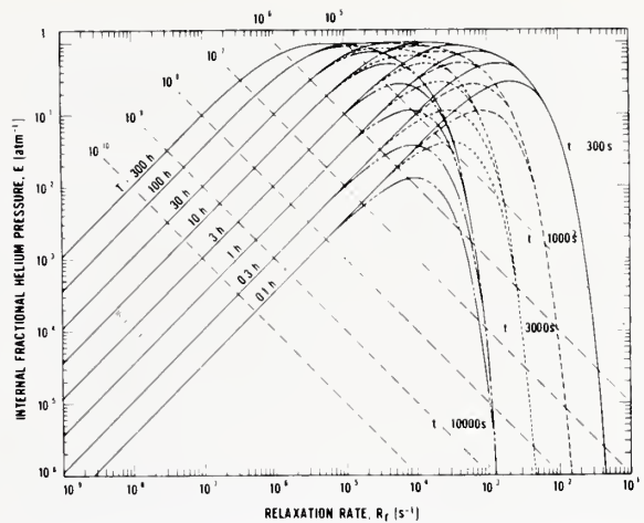
Fig. 2. Test lines for helium leak detector method. E and R_r are for helium gas. Test line values are for R_r \cdot E = \text{constant} with indicated lines ranging from 10^{-5} to 10^{-10} \text{ s}^{-1} \cdot \text{atm}^{-1} .
