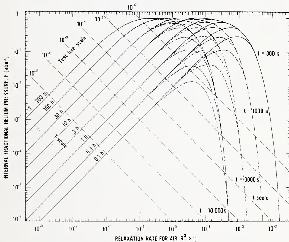
Figure 1. Characteristics and test lines for the helium leak detector method. E , the relative partial pressure of helium within the package per atmosphere of external helium pressurization, as a function of the relaxation rate for air R_r^a with pressurization time T and dwell time t as parameters. Test lines are at -45 deg and correspond to E \cdot R_r^a = \text{const} . Intermediate values for test lines, for T , and for t are indicated by the scale for each. Tick marks include those at 1.25, 1.5, 1.75, and 2.5 with the remainder at integral values for each decade on the axes for E \cdot R_r^a , for T , and for t . Use master graph 1 for photocopying.
