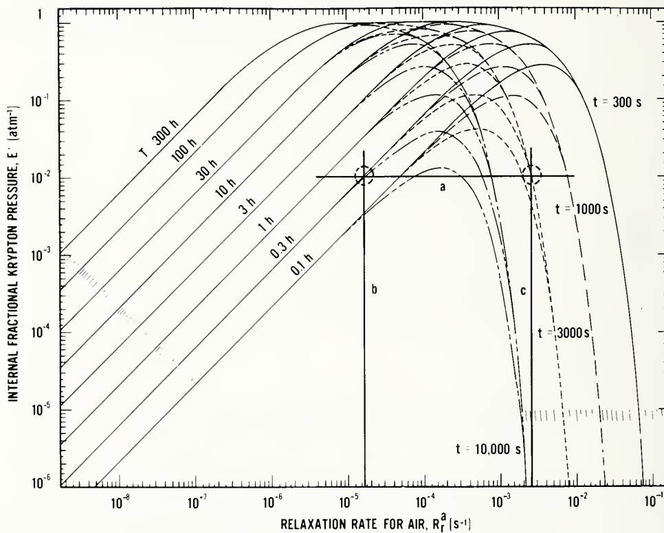
Figure 4. The graphical procedure for determining leak size with the radio-isotope test method from the gamma count rate for given conditions of P_E^* , T , t , and V . See example 1 of Section III. a - test line. b and c - two solutions for R_r^a and hence L_a .
