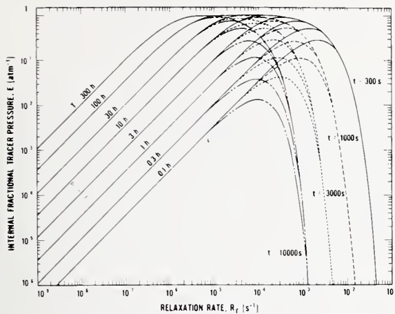
Fig. 1. E , the relative partial pressure of tracer gas within package interior free volume per atmosphere of external tracer gas pressurization, as function of relaxation rate R_r with pressurization time T and dwell time t as parameters. Transport mechanism is molecular flow.
