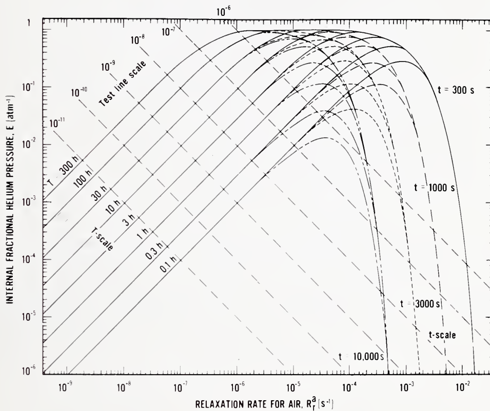
Figure 1. Characteristics and test lines for the helium leak detector method. E, the relative partial pressure of helium within the package per atmosphere of external helium pressurization, as a function of the relaxation rate for air R_r^a with pressurization time T and dwell time t as parameters. Test lines are at -45 deg and correspond to E \cdot R_r^a = \text{const.} Intermediate values for test lines, for T, and for t are indicated by the scale for each. Tick marks include those at 1.25, 1.5, 1.75, and 2.5 with the remainder at integral values for each decade on the axes for E \cdot R_r^a , for T, and for t. Use master graph 1 for photocopying.
