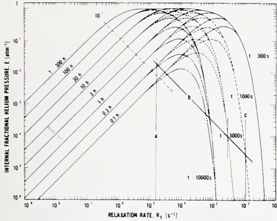
Fig. 3. Selection of pressurization parameters for helium leak detector method: an example. Reject leak size (air) of 5 \times 10^{-8} \text{ atm} \cdot \text{cm}^3/\text{s} with V = 0.01 \text{ cm}^3 , P_E = 5 \text{ atm} , t = 3000 \text{ s} , and minimum detectable signal of 5 \times 10^{-9} \text{ atm} \cdot \text{cm}^3/\text{s} for signal-to-noise of 5. Line (a) represents an R_r of 1.35 \times 10^{-5} \text{ s}^{-1} for helium. Then R/(P_0 V P_E) = 1 \times 10^{-7} \text{ s}^{-1} \cdot \text{atm}^{-1} . First intersection of 10^{-7} test line and (a) at T \sim 0.15 \text{ h} is not satisfactory, so T = 0.3 \text{ h} is chosen. Line (b) becomes the test line. Intersection of (b) at t = 3000 \text{ s} leads to leak size of 1.2 \times 10^{-5} \text{ atm} \cdot \text{cm}^3/\text{s} of air. Line (c) for intersect at t = 1000 \text{ s} leads to L_{\text{air}} \approx 4.1 \times 10^{-5} \text{ atm} \cdot \text{cm}^3/\text{s} .
