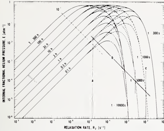
Fig. 3. Selection of pressurization parameters for helium leak detector method: an example. Reject leak size (air) of 5 \times 10^{-8} \text{ atm} \cdot \text{cm}^3/\text{s} with V = 0.01 \text{ cm}^3 , P_E = 5 \text{ atm} , t = 3000 \text{ s} , and minimum detectable signal of 5 \times 10^{-9} \text{ atm} \cdot \text{cm}^3/\text{s} for signal-to-noise of 5. Line (a) represents an R_r of 1.35 \times 10^{-5} \text{ s}^{-1} for helium. Then R/(P_0VP_E) = 1 \times 10^{-7} \text{ s}^{-1} \cdot \text{atm}^{-1} . First intersection of 10^{-7} test line and (a) at T \sim 0.15 \text{ h} is not satisfactory, so T = 0.3 \text{ h} is chosen. Line (b) becomes the test line. Intersection of (b) at t = 3000 \text{ s} leads to leak size of 1.2 \times 10^{-5} \text{ atm} \cdot \text{cm}^3/\text{s} of air. Line (c) for intersect at t = 10000 \text{ s} leads to L_{\text{air}} \approx 4.1 \times 10^{-5} \text{ atm} \cdot \text{cm}^3/\text{s} .
