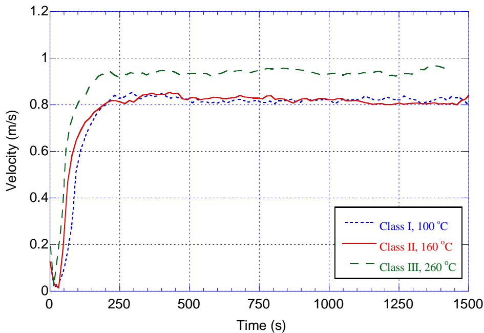
Figure 4 Velocity measured in the FEE test section at three different temperatures.
