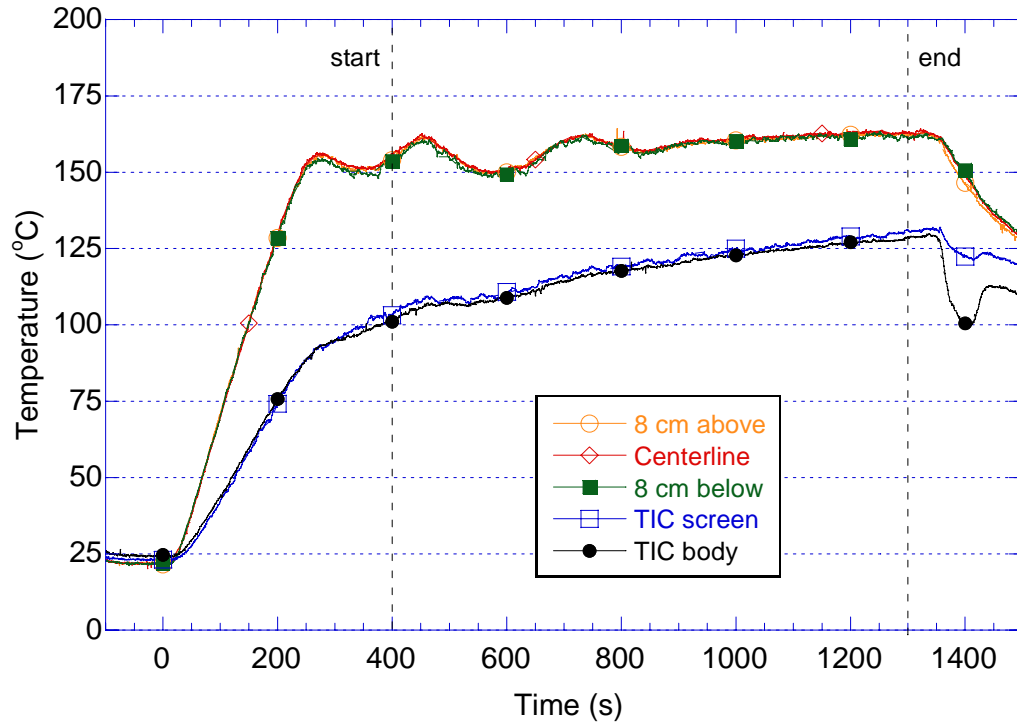
Figure 6 Temperature measurements at Thermal Class II, 160 °C.
