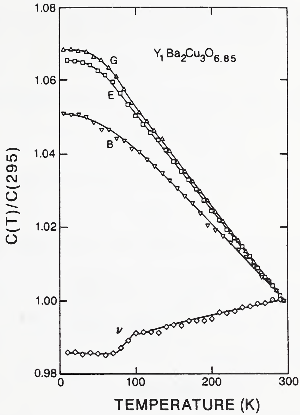
Figure 4.3: Temperature variation of elastic constants of polycrystal YBCO superconductor.
