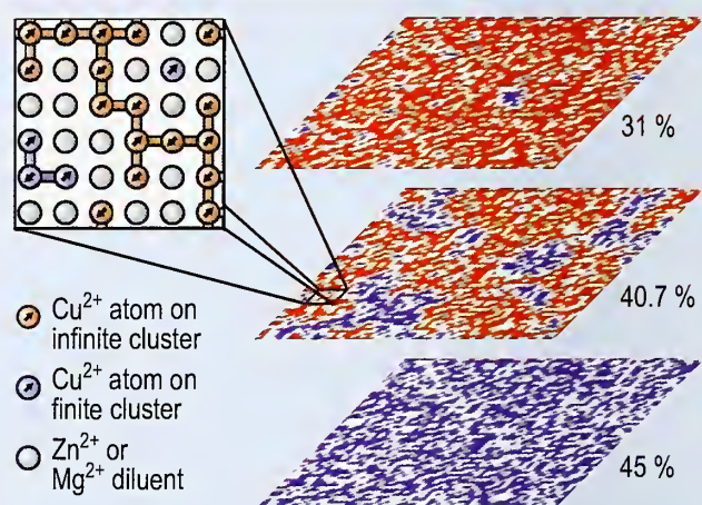
Fig. 1. A schematic of finite sections of the infinite lattice at dilution levels well below (31 %), just below (40.7 %), and above (45 %) the percolation threshold. Sites on the infinite cluster are shown in red, sites on finite disconnected clusters are blue, and diluents are in white. The inset is a close-up view for z = 40.7\% , showing the role that magnetic Cu and non-magnetic Zn/Mg ions play in the experimental system.
