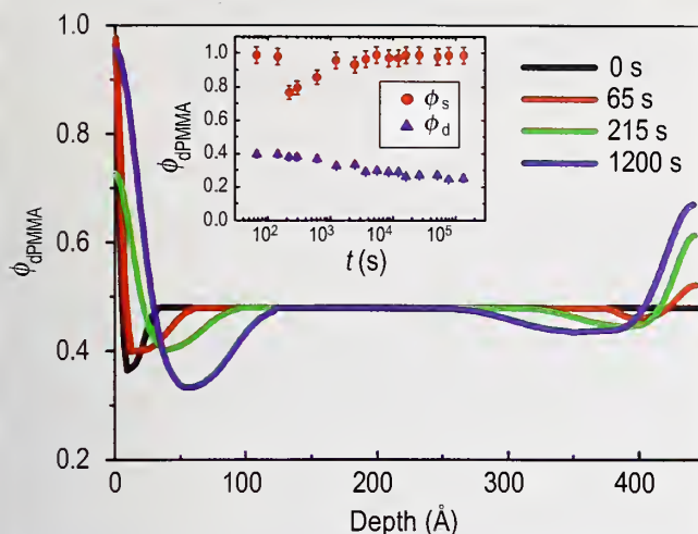
Fig. 2. \phi_{\text{PMMA}} profiles that give the best fit. The inset shows the evolution of surface composition, \phi_s (circles) and depletion layer composition, \phi_d (triangles).
