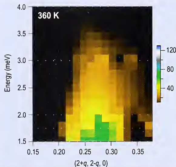
Fig. 3. Dynamic polaron correlations above the glass transition.
