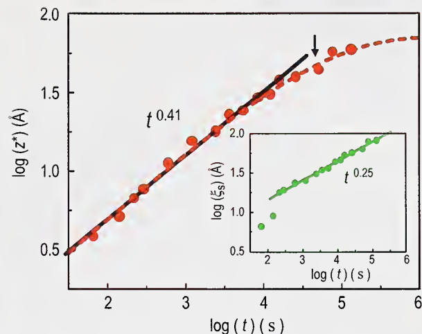
Fig. 3. z^* with a power-law fit (solid line), t^{0.41} , and a stretched exponential function (dashed curve). The arrow denotes a z^* \approx 40 \text{ Å} and the transition to slower growth. The inset shows the surface correlation length.
