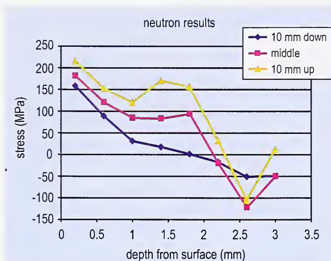
Fig. 4. Hoop stresses as a function of depth in the 3.2 mm thick steel cup, as determined by neutron diffraction.
