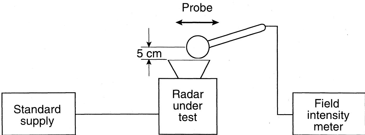
Figure 8. The antenna near-field power density measurement setup.
