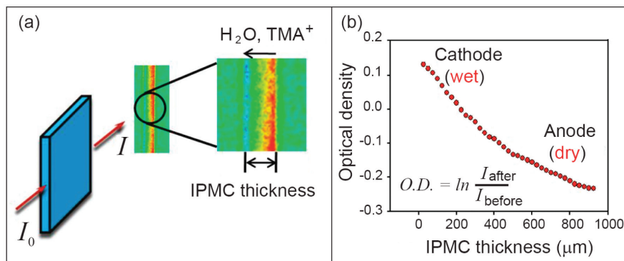
FIGURE 3: (a) Colorized images showing water/counterion -depleted zones represented by red pixels and water/counterion -rich areas represented by blue pixels. IPMC was subjected to 3 V DC. (b) Relative neutron optical density due to water/counterion gradient profile across the IPMC thickness.
