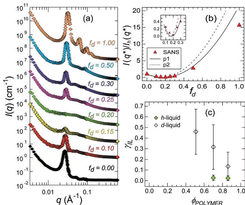
FIGURE 1: (a) SANS intensity profiles (offset for clarity) for various values of deuterated copolymer volume fraction f_d as a function of q for polymer volume fraction \phi_{\text{POLYMER}} = 0.86 mixtures in h -liquid at 30 °C. (b) Experimentally measured and modeled normalized peak intensities of the data in Fig. 1a as a function of f_d . Inset shows detail near the contrast match composition. (c) Ionic liquid partition coefficient, \gamma_{\text{IL}} , for partitioning into PS blocks for varying copolymer to h -liquid and d -liquid mixture compositions as a function of copolymer volume fraction \phi_{\text{POLYMER}} .
