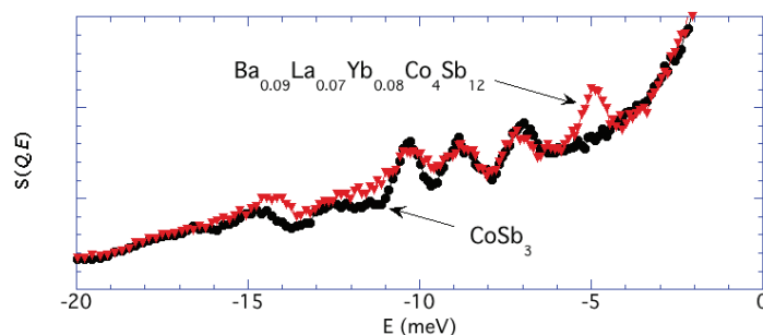
FIGURE 2: A comparison of 4.8 \text{ \AA} neutron energy gain data for the normalized unfilled \text{CoSb}_3 , and for \text{Ba}_{0.09}\text{La}_{0.07}\text{Yb}_{0.08}\text{Co}_4\text{Sb}_{12} .
