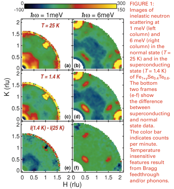
Figure 1f shows enhancement of magnetic scattering at \hbar\omega = 6 meV for elliptical regions associated with Q = (0.5, 0.5, 0) nesting of electron and hole pockets of the Fermi surface. A staple of magnetic superconductors, the corresponding spectroscopic resonance in \text{Fe}_{1+y}\text{Se}_{0.4}\text{Te}_{0.6} is evidence the (s+) superconducting gap function has opposite signs on the nesting electron and hole Fermi surfaces [3].
