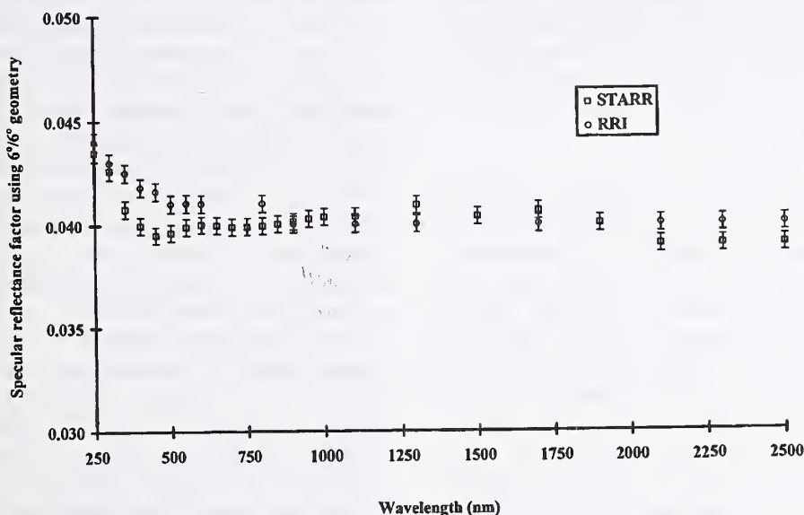
Fig. 5. Specular reflectance factor of NG-9 black glass using 6^\circ/6^\circ geometry as measured by STARR and by RRI.
