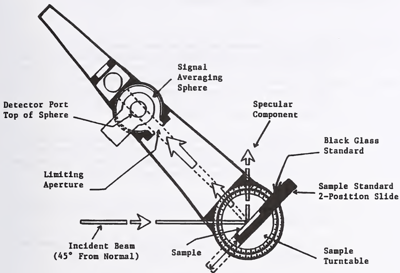
Figure 2. 45°/0° Reflectometer System (Top View)
