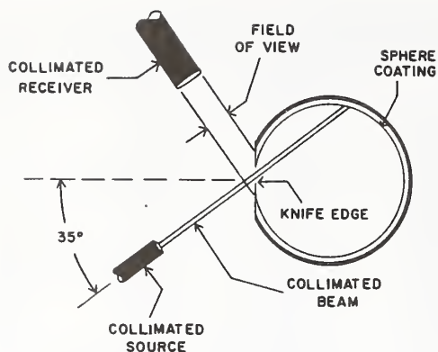
FIGURE 6. Arrangement of knife-edge apparatus for measuring N_g(\gamma) .
