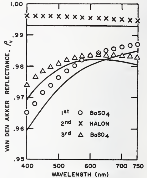
FIGURE 5. Van den Akker reflectance of three coatings. (The height of the symbols \times represent the total uncertainty. Height of the symbols 0 and \Delta represents approximately 4 times the total uncertainty.) The associated solid curves show \rho(6^\circ, \lambda) for each coating.
