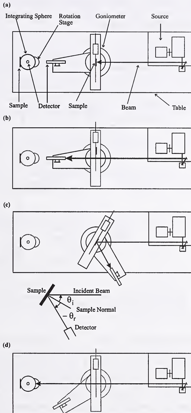
Figure 3.1. Schematics of the STARR instrument showing top views of the major components (a) and the geometrical arrangements for measuring the incident directional flux (b), the reflected directional flux (c), and the reflected hemispherical flux (d). The conventions for the incident and reflected angles are also shown in (c).
