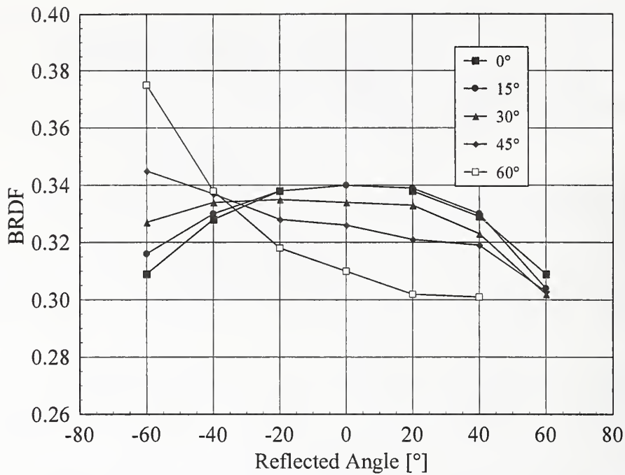
Figure 3.9. BRDF as a function of reflected angle at 632.8 nm for a PTFE plaque at the indicated incident angles. The relative expanded uncertainties of the BRDF, less than 0.2 percent, are within the sizes of the symbols.
