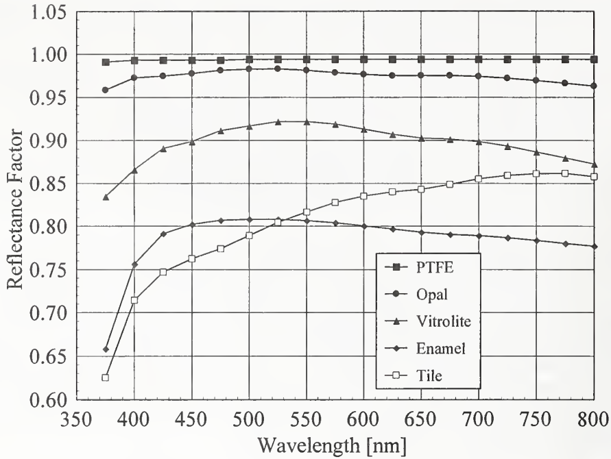
Figure 3.10. 6^\circ - hemispherical reflectance factor as a function of wavelength for the materials listed in the legend. The relative expanded uncertainties of the reflectance factor, approximately 0.3 percent, are within the sizes of the symbols.
