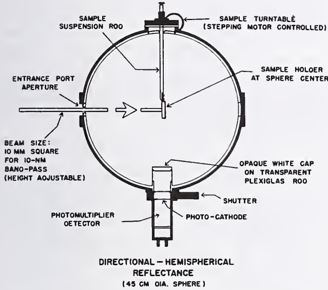
FIGURE 9. Integrating sphere for measuring relative directional-hemispherical reflectance as a function of angle of incidence.
