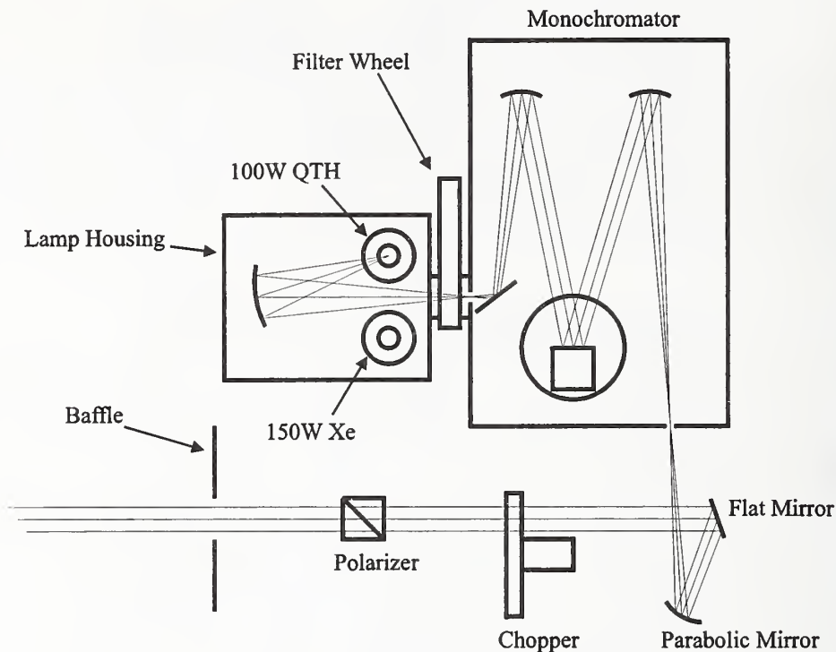
Figure 3.2. Top view of the components and optical path of the source of radiant flux for the STARR instrument.
