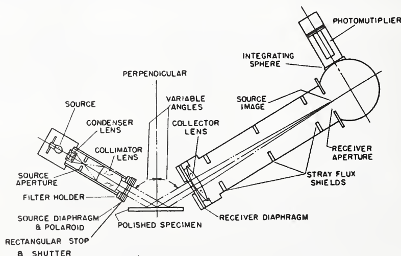
FIGURE 7. NBS-Gaertner goniophotometer.
