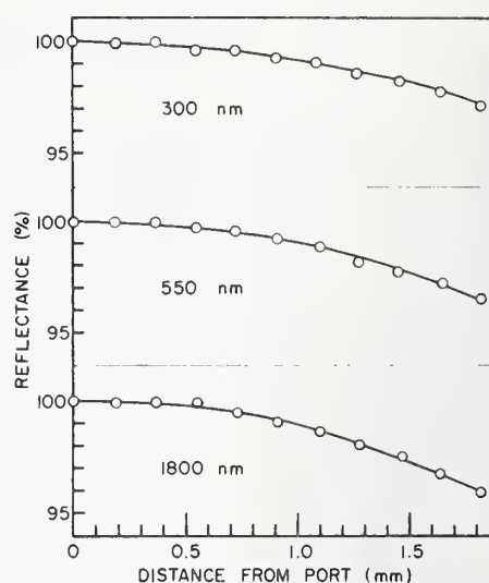
Figure 1. Measured diffuse reflectance of a pressed PTFE powder specimen is influenced by varying the spacing between the plane of the specimen and the plane of the integrating sphere port. The effect is shown for measurements at 300, 550, and 1800 nm.
