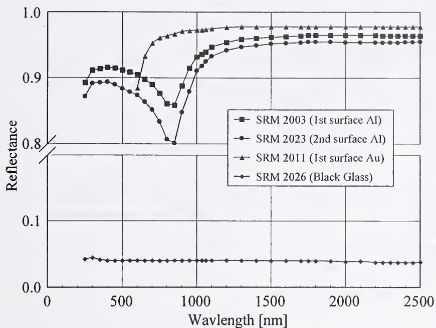
Figure 3.7. Specular reflectance as a function of wavelength for the SRMs listed in the legend. The relative expanded uncertainties of the reflectances, approximately 0.1 percent, are within the sizes of the symbols.
