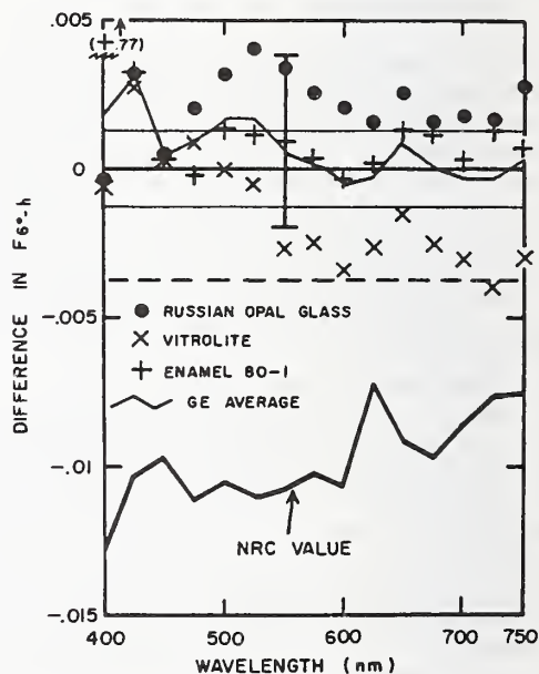
FIGURE 17. Comparison of present NBS scale of F_{d-h} (taken as zero line) to previous NBS scale and to Results of an intercomparison with NRC.
