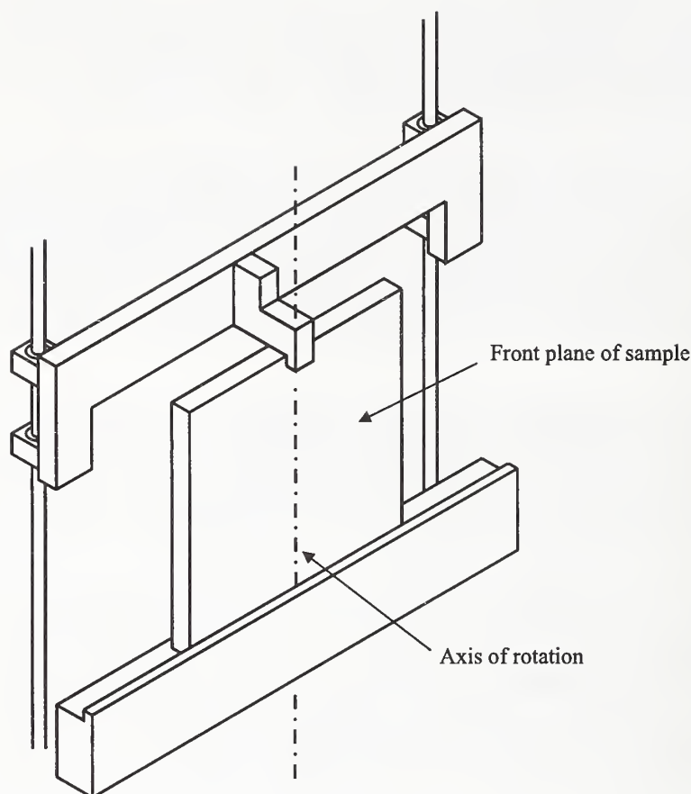
Figure 3.6. Sample mount of the STARR goniometer.
