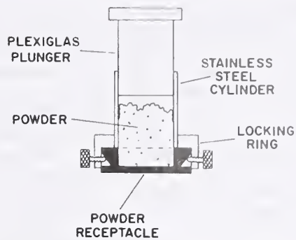
Fig. 2. Powder press is designed to provide a means for controlling the density of pressed PTFE diffuse reflectance standards. The preferred density is 1 g/cm 3 .
