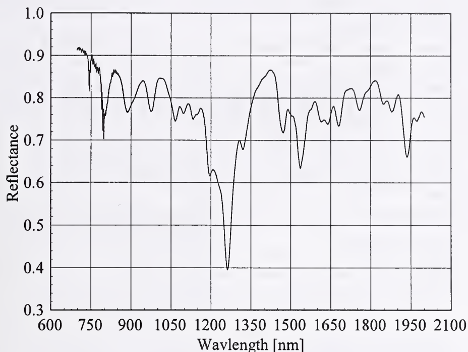
Figure 4.2. Reflectance as a function of wavelength for the rare-earth mixture wavelength standard SRM 1920a.
