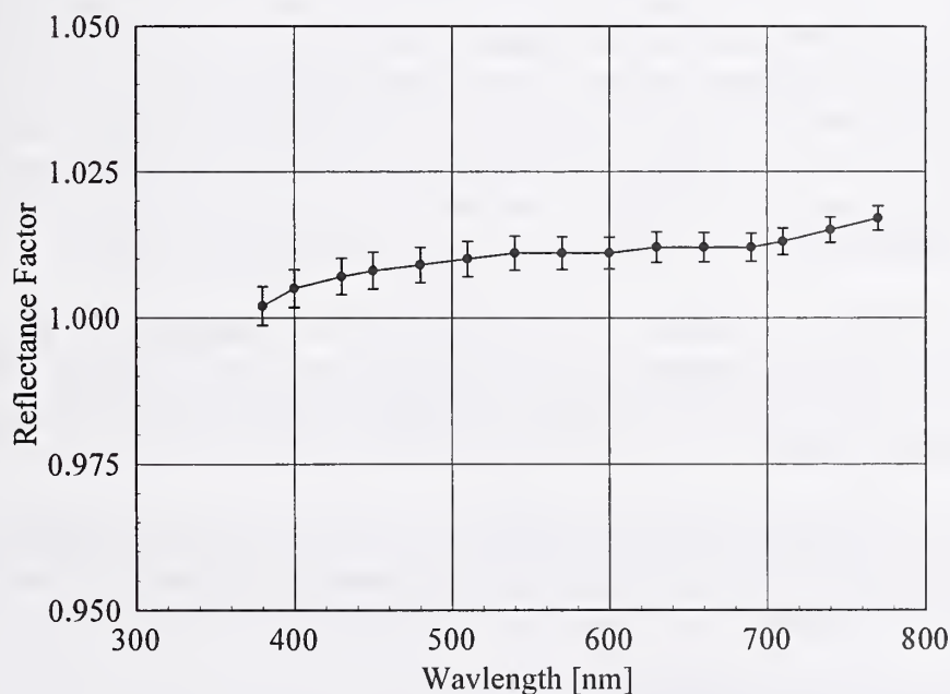
Figure 3.8. 45°/0° reflectance factor as a function of wavelength for a PTFE plaque. The vertical bars are the expanded uncertainties of the reflectance factor.
