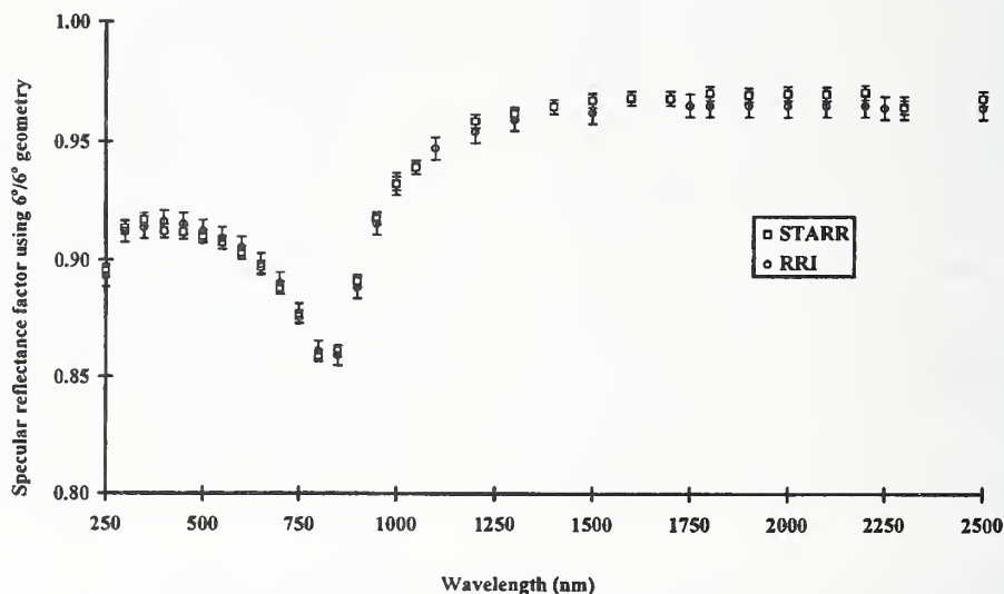
Fig. 3. Specular reflectance factor of a first-surface-aluminum-coated mirror using a 6^\circ angle of incidence and a 6^\circ angle of observation ( 6^\circ/6^\circ geometry) as measured by the STARR and the Reference Reflectance Instrument (RRI).
