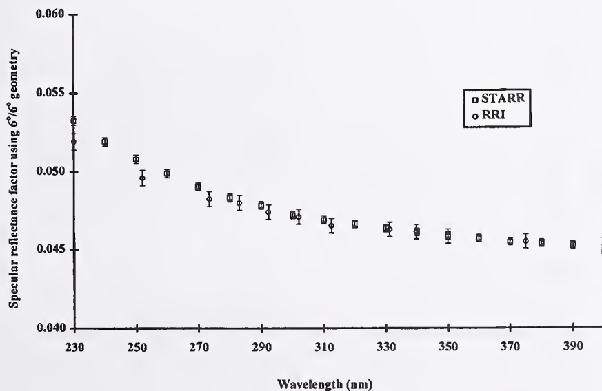
Fig. 6. Specular reflectance factor of GL-2 black glass using 6^\circ/6^\circ geometry as measured by STARR and by RRI.
