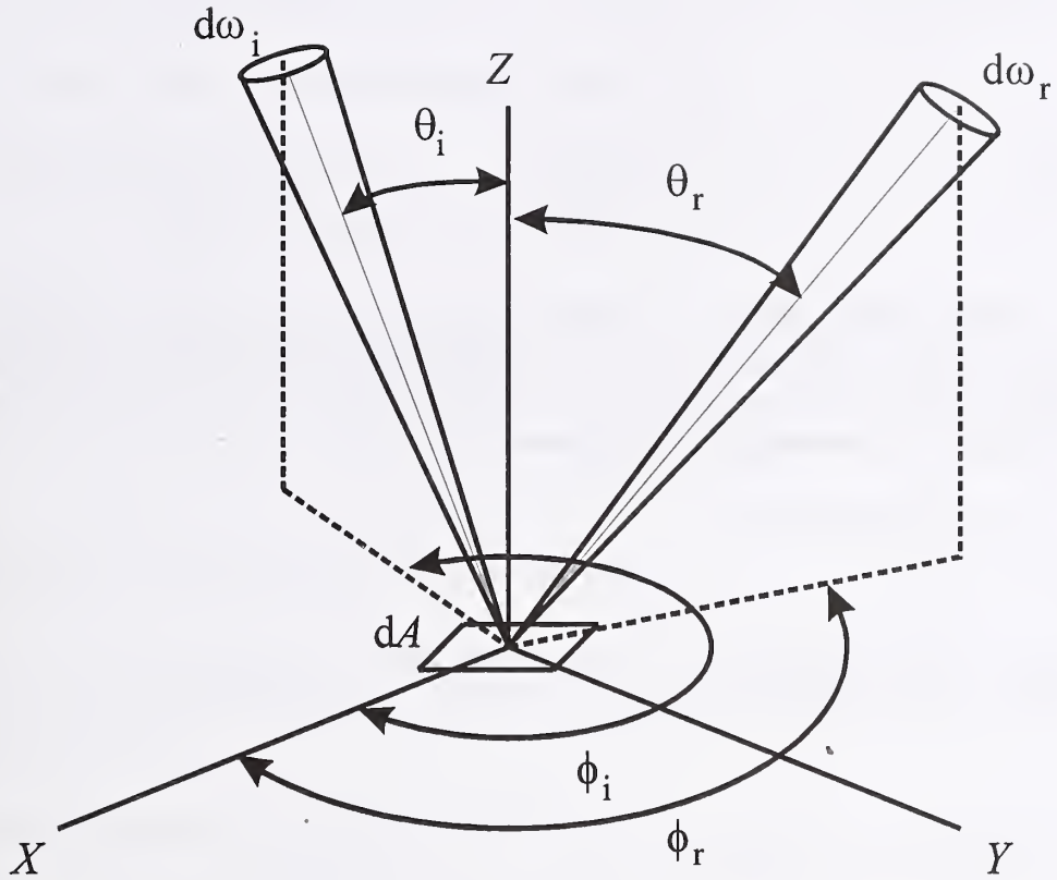
Figure 2.1. Geometry of incident and reflected elementary radiant beams.
