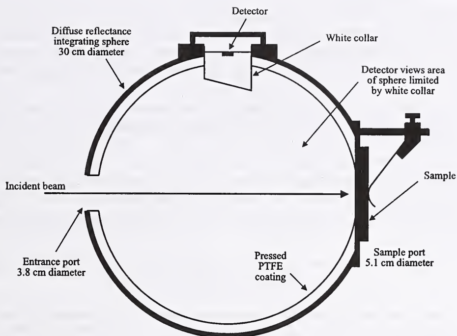
Figure 3.5. Cross-section of the integrating sphere used for 6° - hemispherical reflectance measurements with the STARR instrument.
