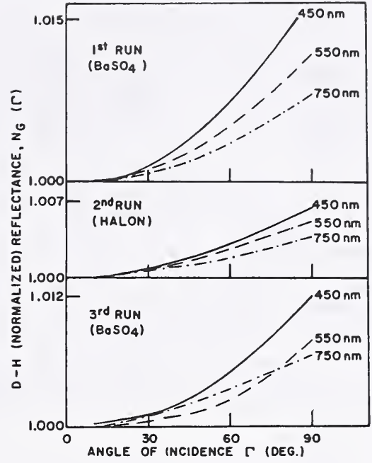
FIGURE 10. Relative directional-hemispherical reflectance N_d(\Gamma, \lambda) as a function of angle of incidence \Gamma for each of three coatings at three wavelengths.
