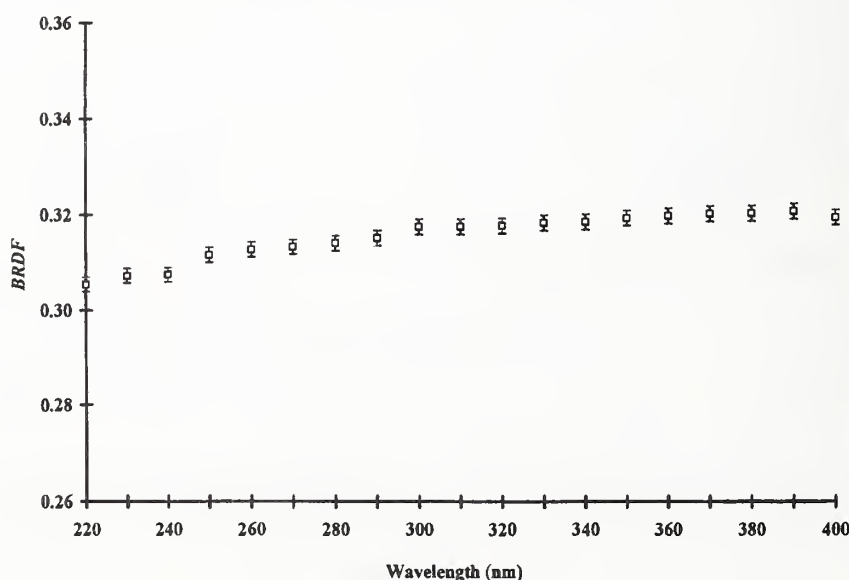
Figure 7. BRDF of pressed Polytetrafluoroethylene (PTFE) using 45°/0° geometry as measured by STARR.
