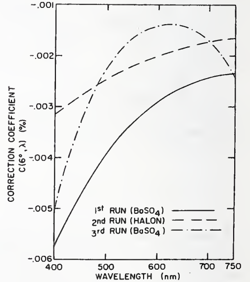
FIGURE 13. C(6^\circ, \lambda) as a function of wavelength for each of three coatings.
