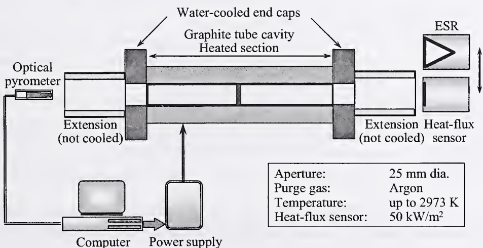
Figure 2. Schematic layout of the VTBB
