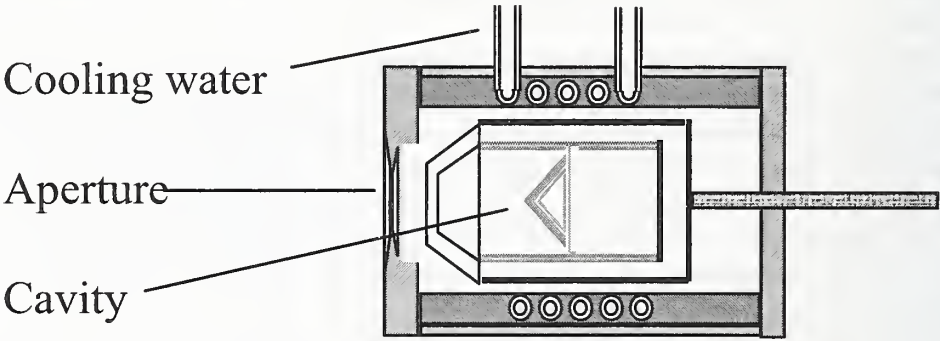
Figure 3. Transfer standard Kendall radiometer layout.
